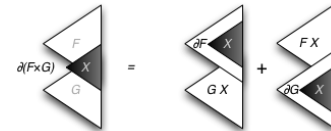
Figure 25 The hole in a one-hole context of a pair is either in the first or in the second component.
