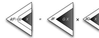
Figure 26 Chain rule. The hole in a composition arises by making a hole in the enclosing structure and fitting the enclosed structure in.
