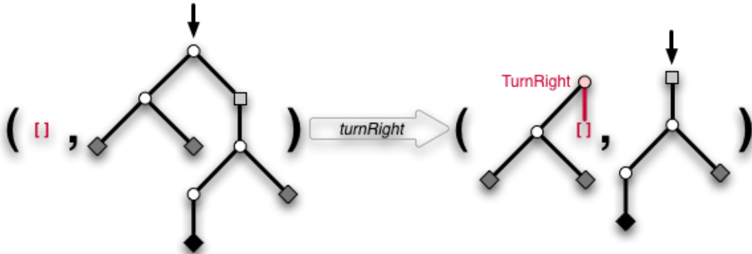
Figure 20: Taking the right subtree from the entrance. Of course, the thread is initially empty. Note that the thread runs backwards, i.e. the topmost segment is the most recent.
