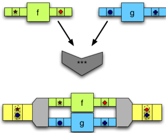
Figure 11: The (***) robot: running the combined arrow
