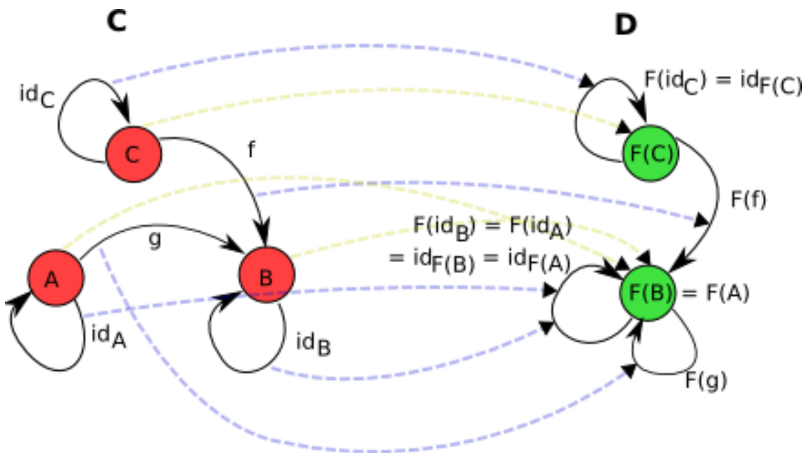
Figure 33: A functor between two categories, C and D . Of note is that the objects A and B both get mapped to the same object in D , and that therefore g becomes a morphism with the same source and target object (but isn't necessarily an identity), and id_A and id_B become the same morphism. The arrows showing the mapping of objects are shown in a dotted, pale olive. The arrows showing the mapping of morphisms are shown in a dotted, pale blue.
