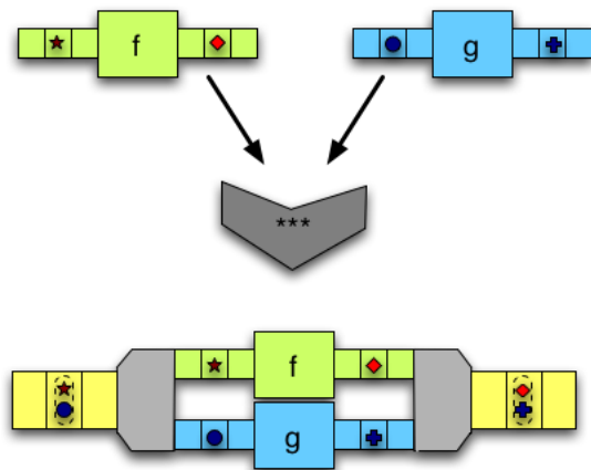
Figure 9: The (***) robot: running the combined arrow
