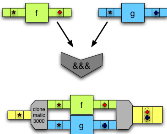
Figure 11: The &&& robot: the resulting arrow with inputs
