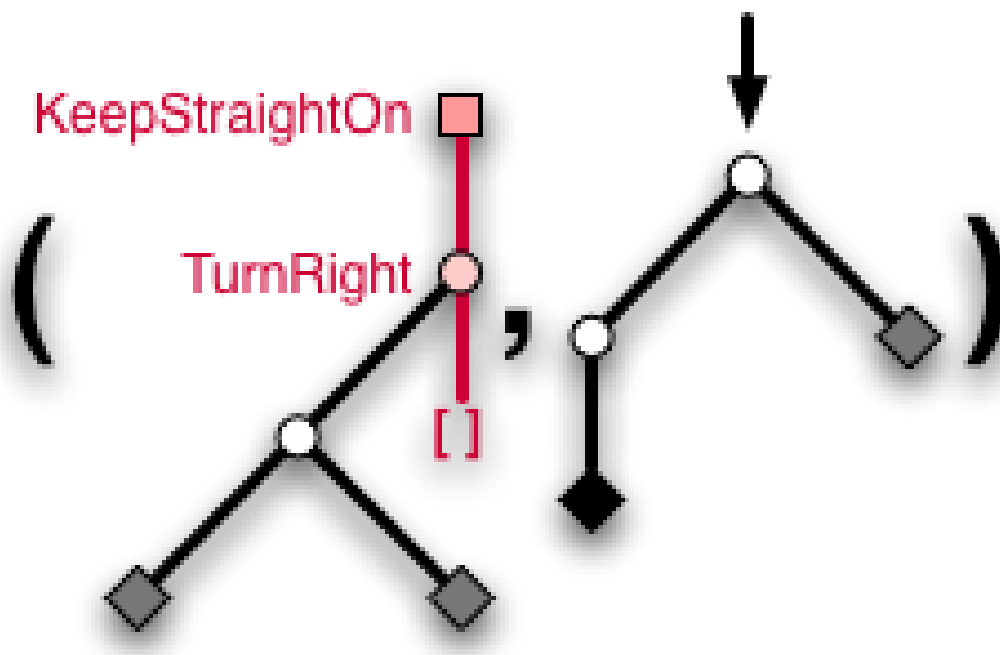
Figure 17: The zipper is a pair of Ariadne's thread and the current sub-labyrinth that the player stands on top. The main thread is colored red and has sub-labyrinths attached to it, such that the whole labyrinth can be reconstructed from the pair.
