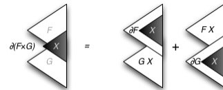
Figure 23 The hole in a one-hole context of a pair is either in the first or in the second component.
