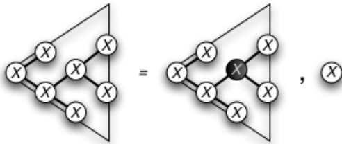
Figure 21: Removing a value of type X from a \text{Tree } X leaves a hole at that position.
