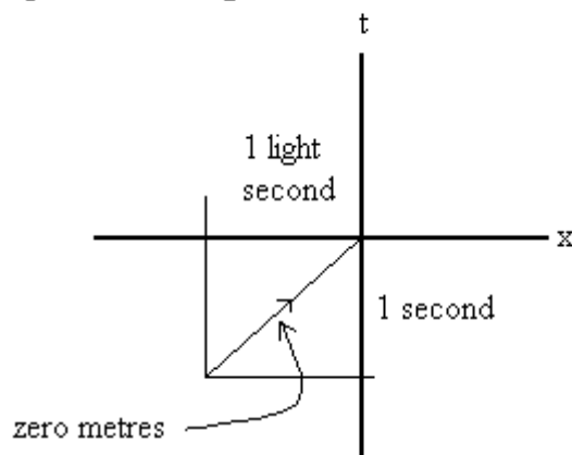
The path of a light ray is a space-time interval of zero but appears as a long line in the diagram.
