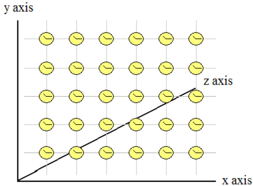
An inertial reference frame
