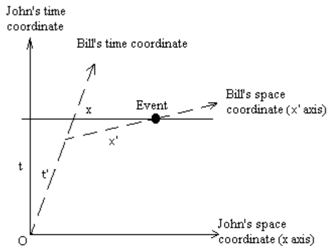
The Lorentz Transformation: How observers with two different coordinate systems view the same event. In this case John and Bill are in space vehicles travelling past each other at 'O' where they synchronise clocks. The objective is to calculate what the other observer reports as the time and position of the event
