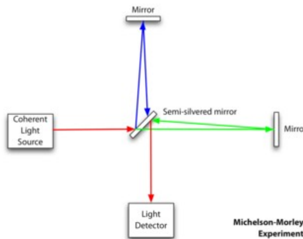
A Michelson Interferometer
