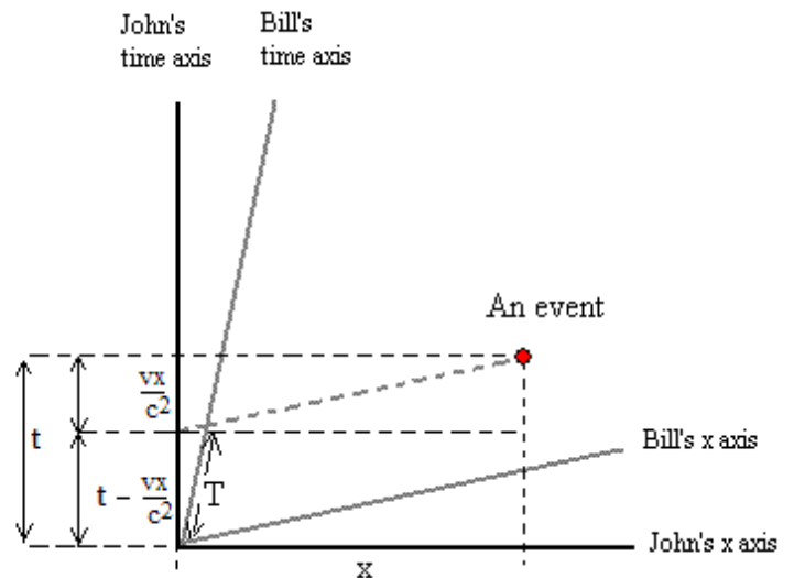
The Lorentz Transformation
