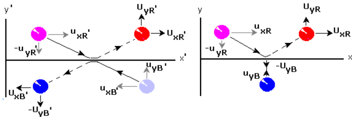
View of observer who is travelling at a velocity intermediate between that of the balls. (Red = +v Blue = -v Observer = 0 m/s)
