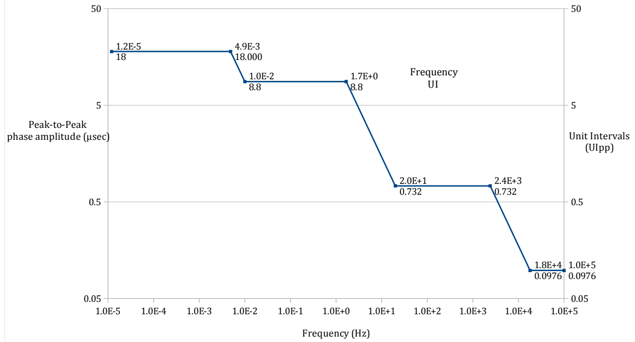
2048 kbps - Input wander and jitter tolerance limit
