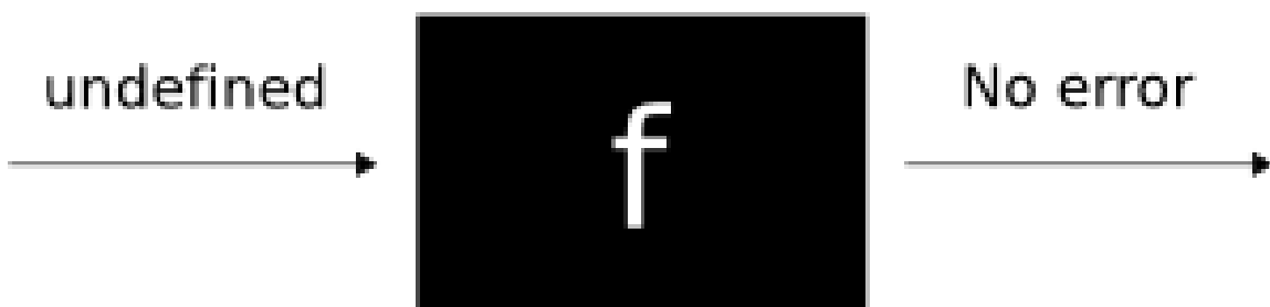
Figure 37: If f returns an error when passed undefined, it must be strict. Otherwise, it's lazy.
