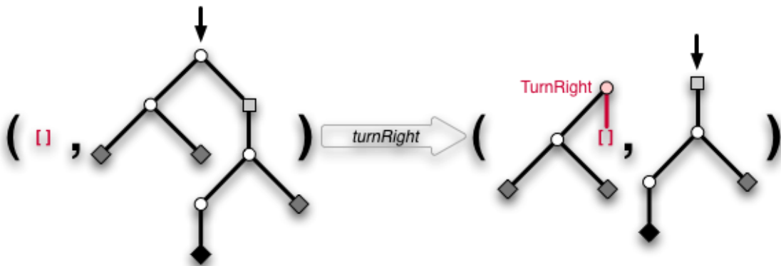
Figure 18: Taking the right subtree from the entrance. Of course, the thread is initially empty. Note that the thread runs backwards, i.e. the topmost segment is the most recent.
