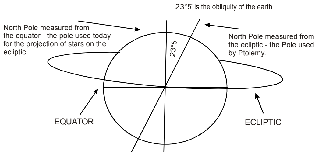
THE POLES OF THE ECLIPTIC AND THE POLES OF THE EQUATOR
