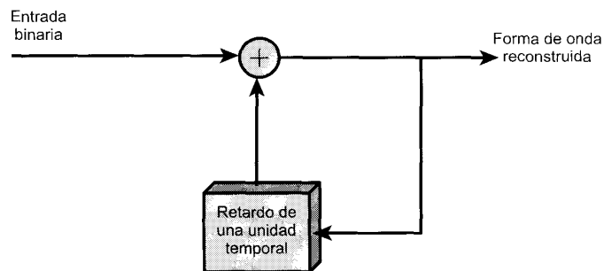
(b) Recepción
