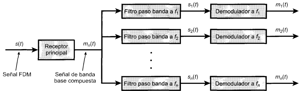
(c) Receptor
