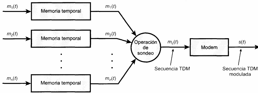
(a) Transmisor
