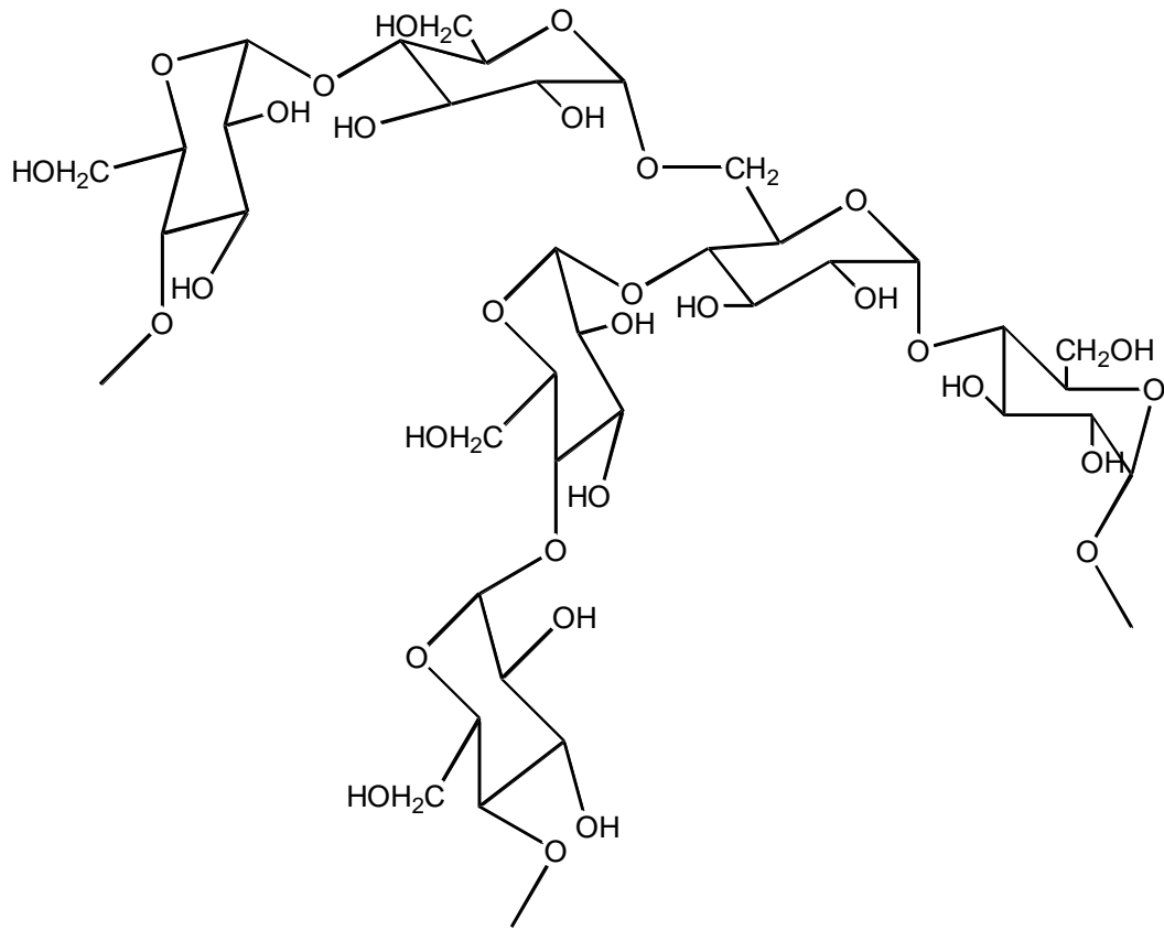
Amylopectin
