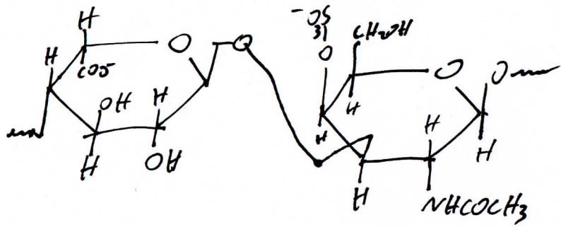
Dermatan sulfate
