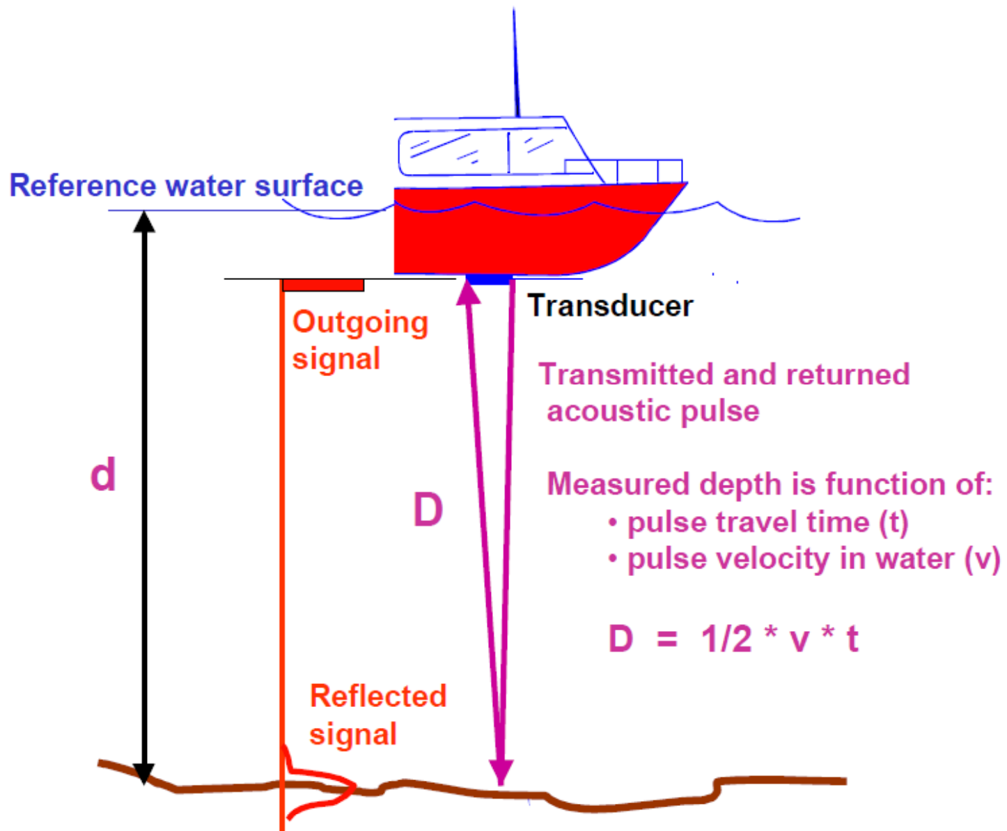
Figure 9-1. Acoustic depth measurement
