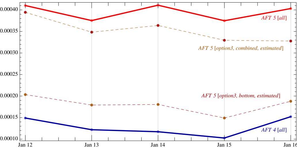
Conversion rates: AFT5 vs AFT4
