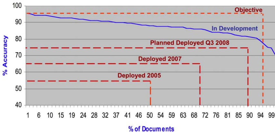
Figure 32: GALE's steadily improving Arabic newswire translation accuracy.
