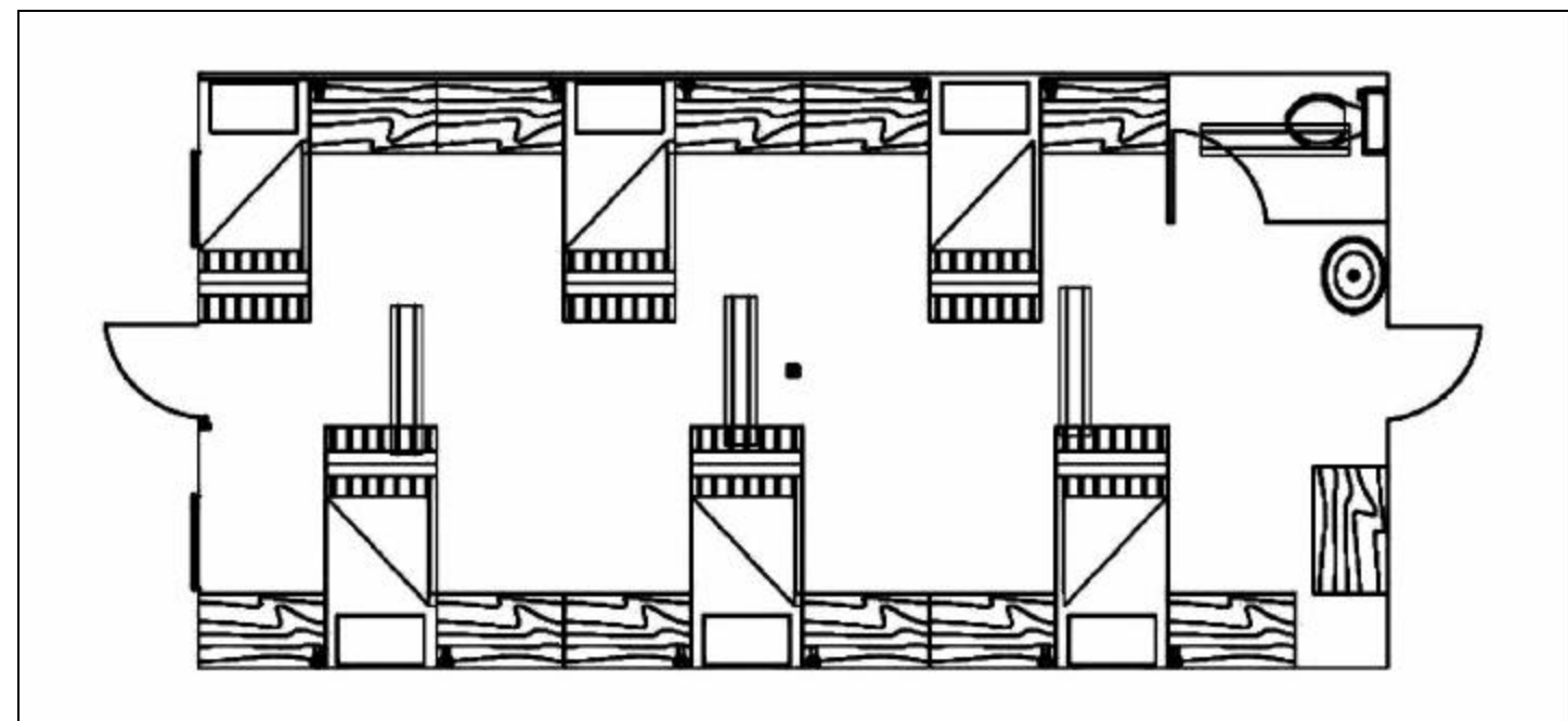
The new SEAhut: Floor diagram of one room of the planned Camp America North hard barracks. Each room will be a SEAhut-sized 16 feet by 32 feet, with six bunk beds, 12 wall lockers, 4 overhead lights and an in-house commode and sink.
