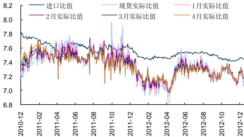
沪铜/伦铜各合约沪伦比值
