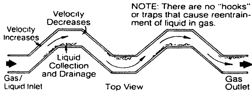
Serpentine Mist Extractor (NATCO, 1993)
