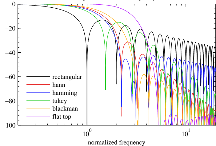
windowing functions in the frequency domain
