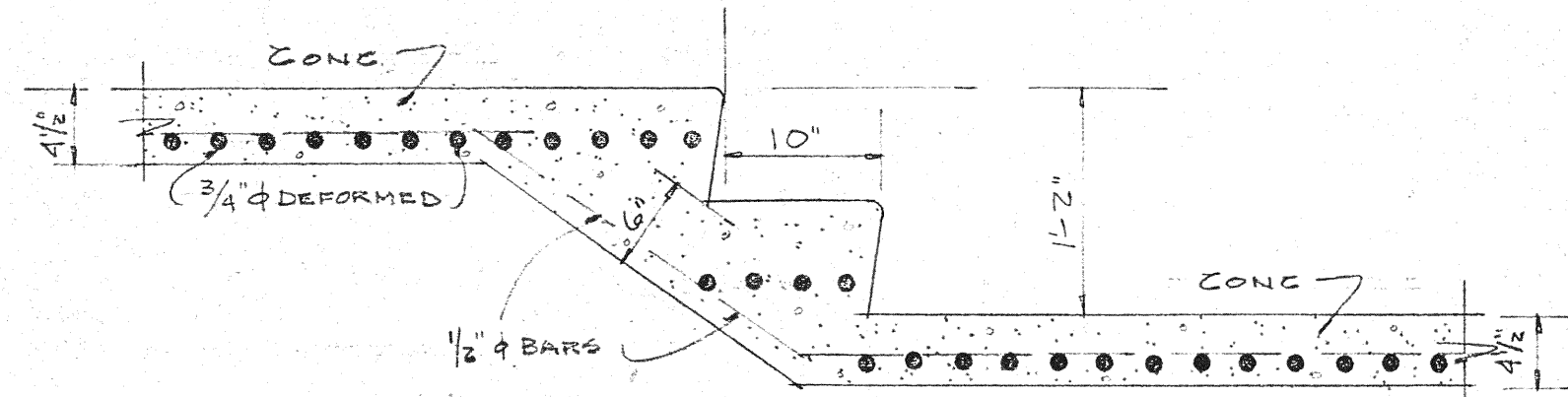
TYPICAL SECTION 1" = 1'-0"
