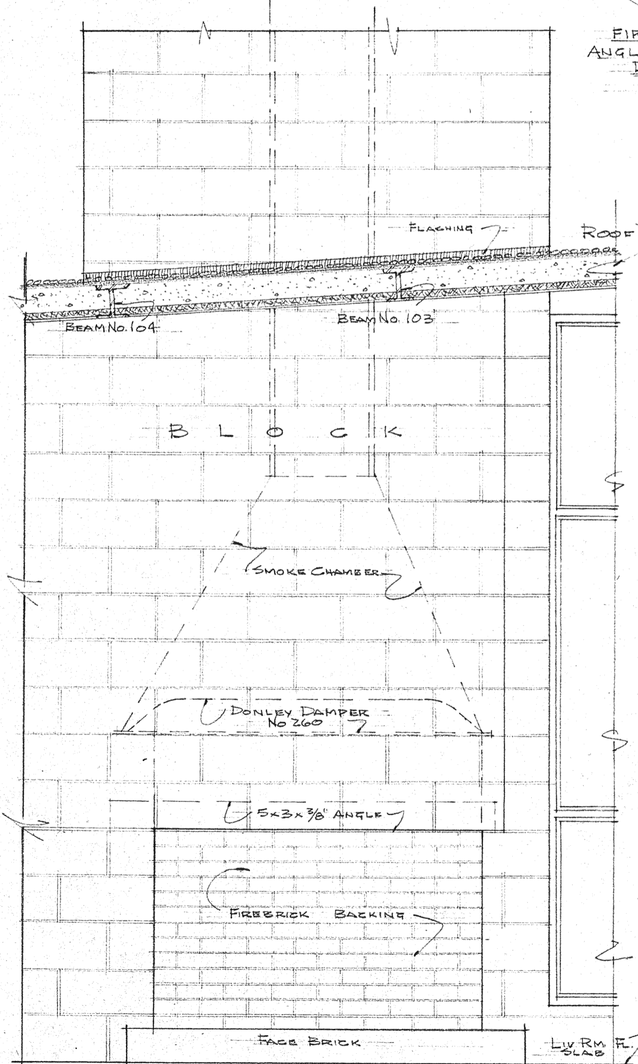
ELEVATION LIVING ROOM FIREPLACE 3/4" = 1'-0"
