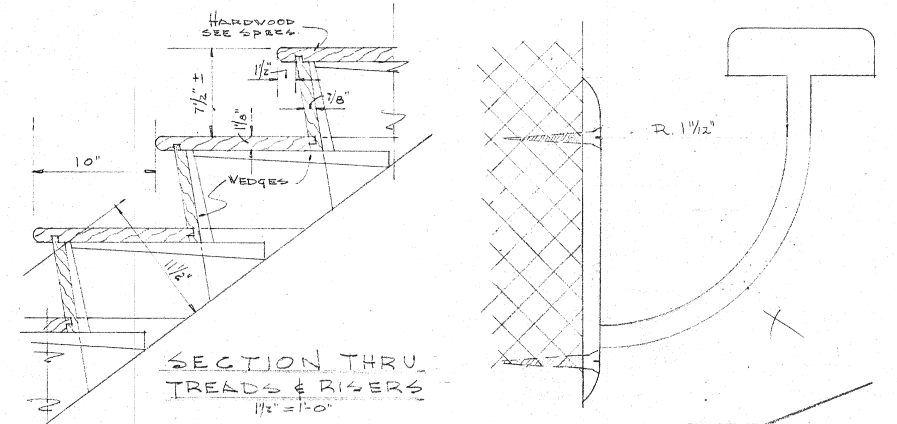
SECTION A-A 1/2" = 1'-0"
