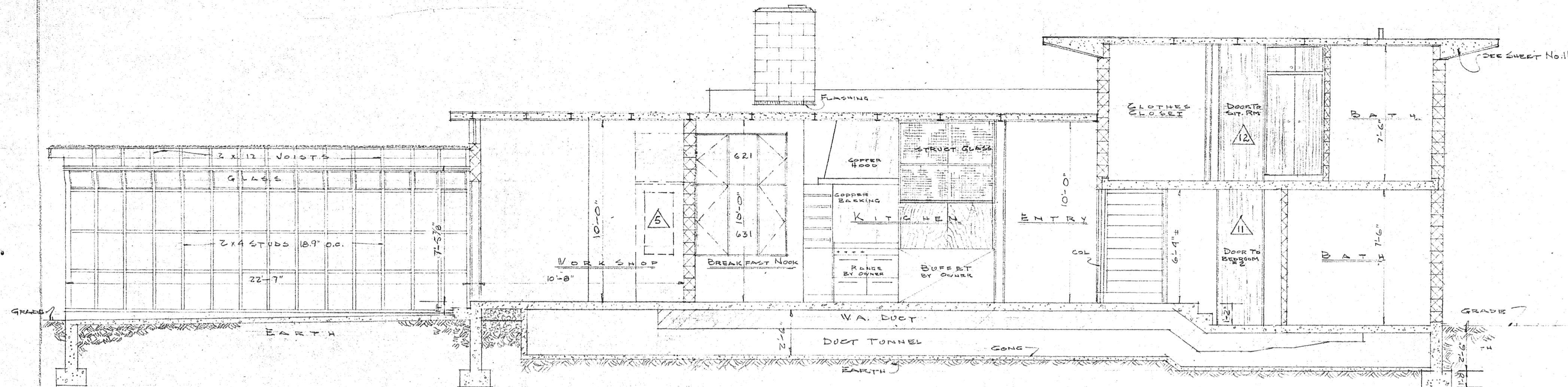
EAST - WEST SECTION \frac{1}{4}'' = 1'-0''
