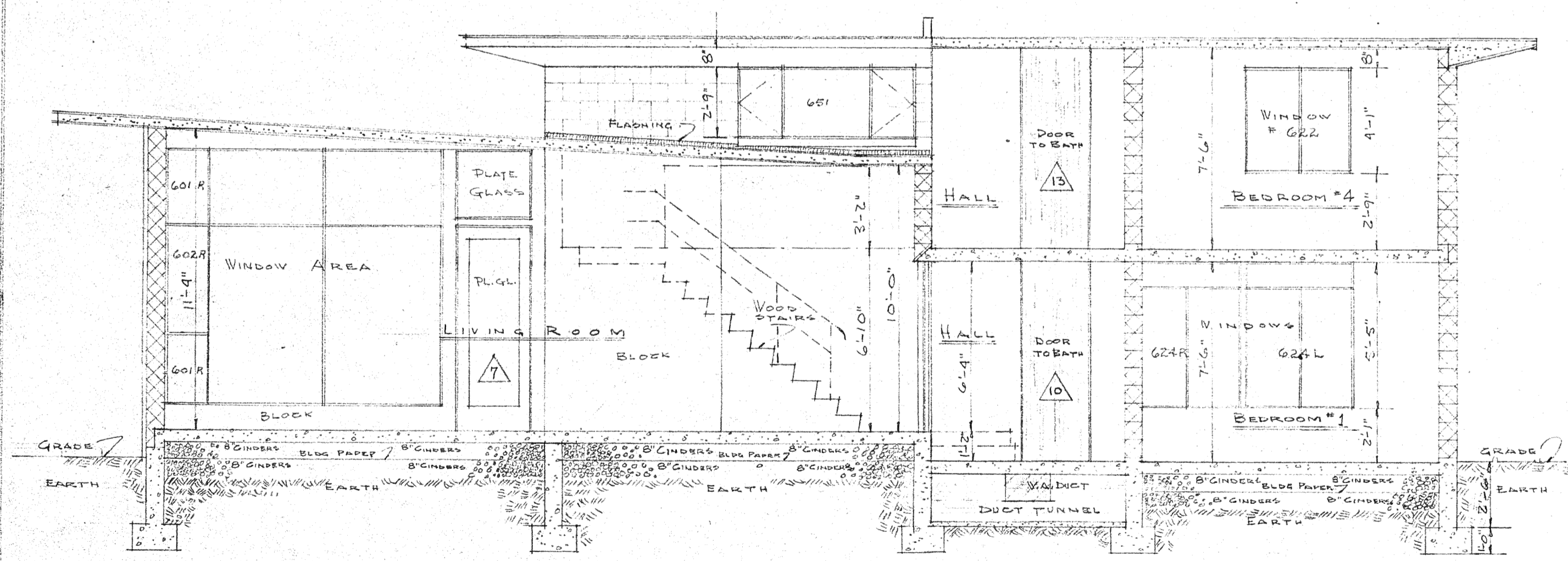
NORTH - SOUTH SECTION \frac{1}{4}'' = 1'-0''
