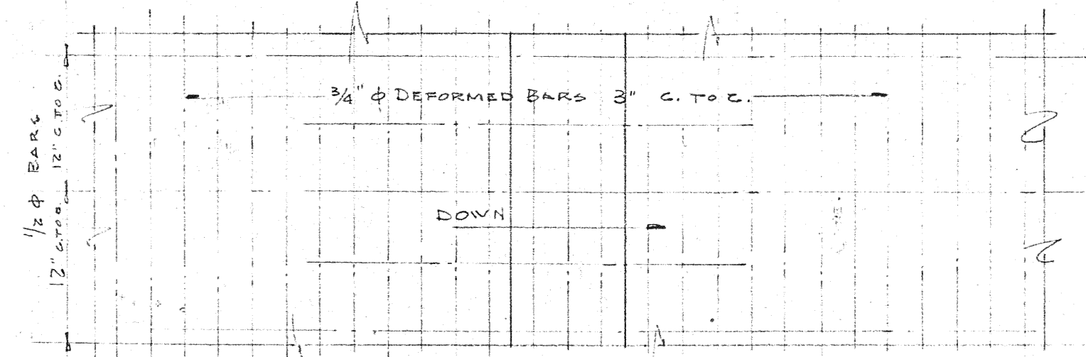
PLAN SLAB OVER PLENUM SEE SECTION B-B 1" = 1'-0"
