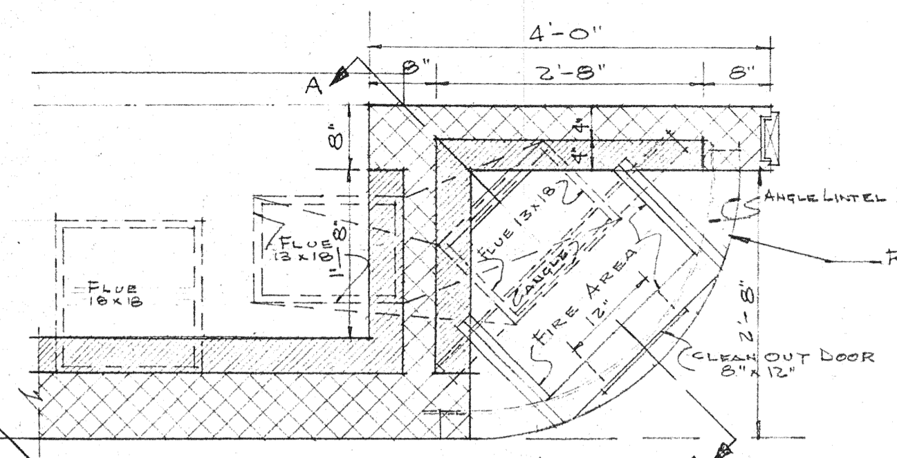
PLAN EXTERIOR FIREPLACE 3/4" = 1'-0"
