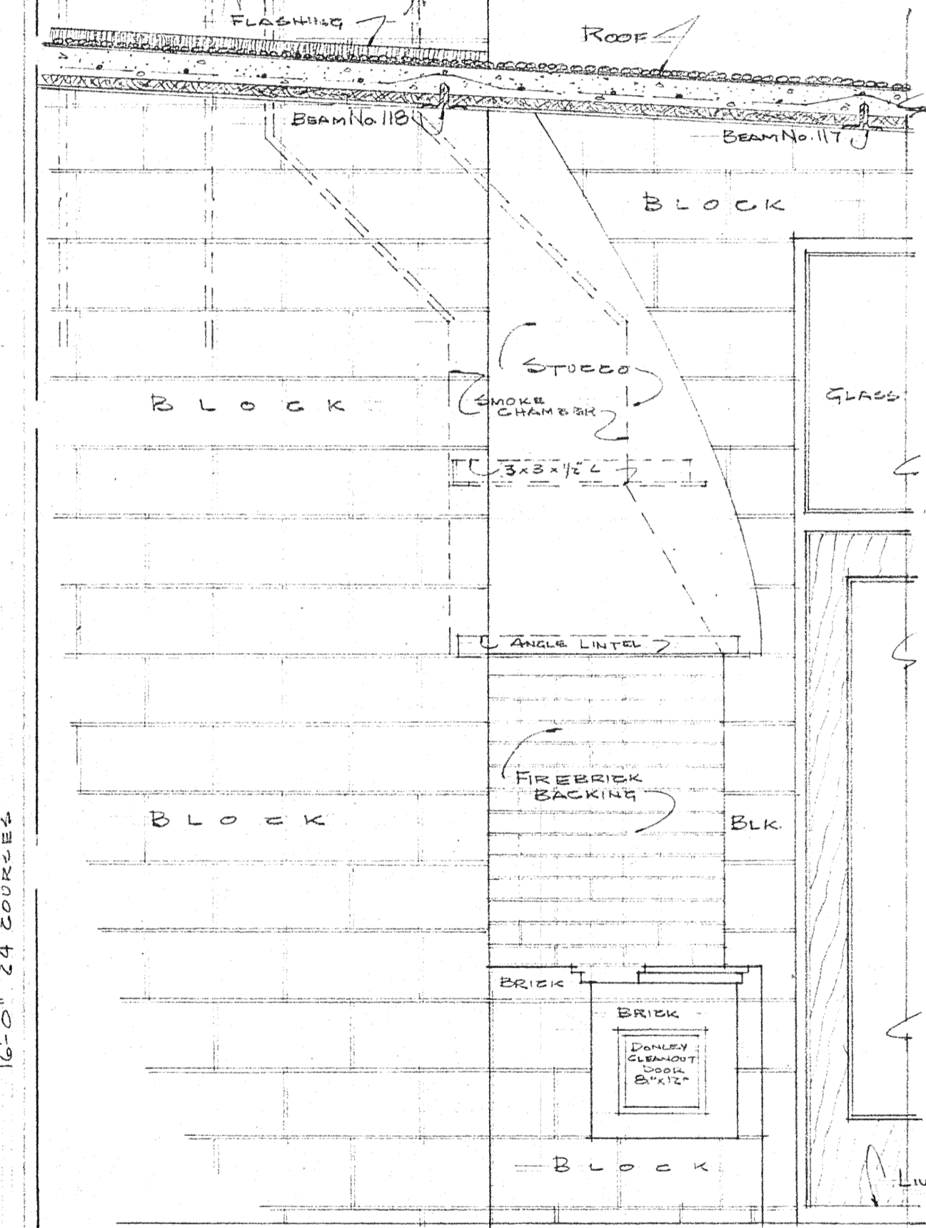
SIDE ELEVATION EXTERIOR FIREPLACE 3/4" = 1'-0"
