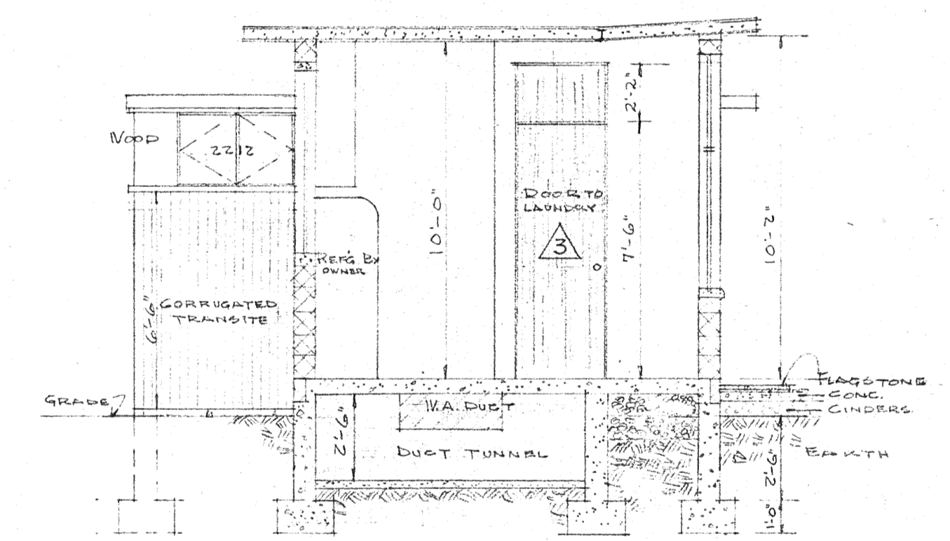
SECTION THRU KITCHEN \frac{1}{4}'' = 1'-0''
