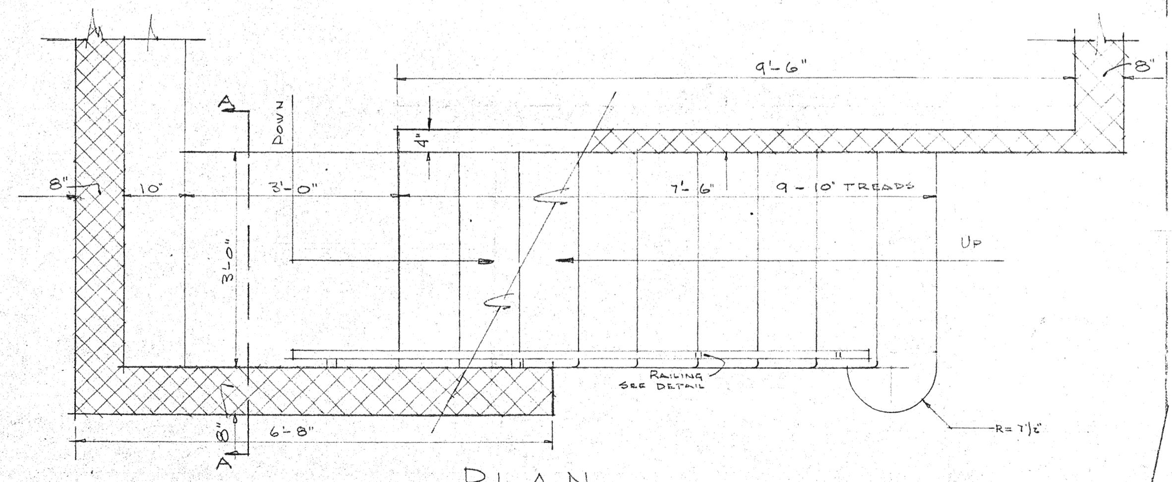
PLAN MAIN STAIRS 3/4" = 1'-0"
