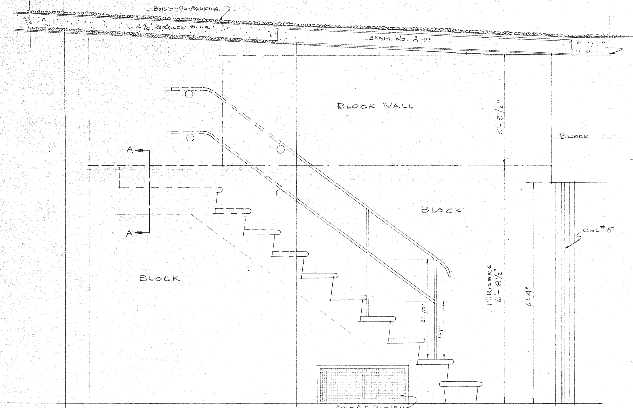
ELEVATION MAIN STAIRS 3/4" = 1'-0"
