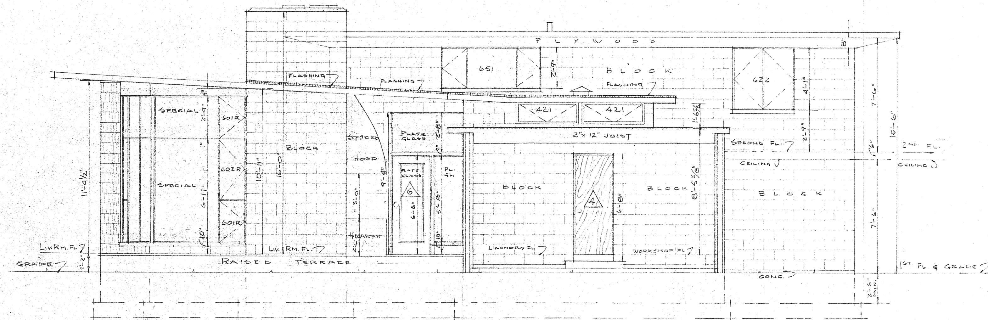
EAST ELEVATION 1/4" = 1'-0"
