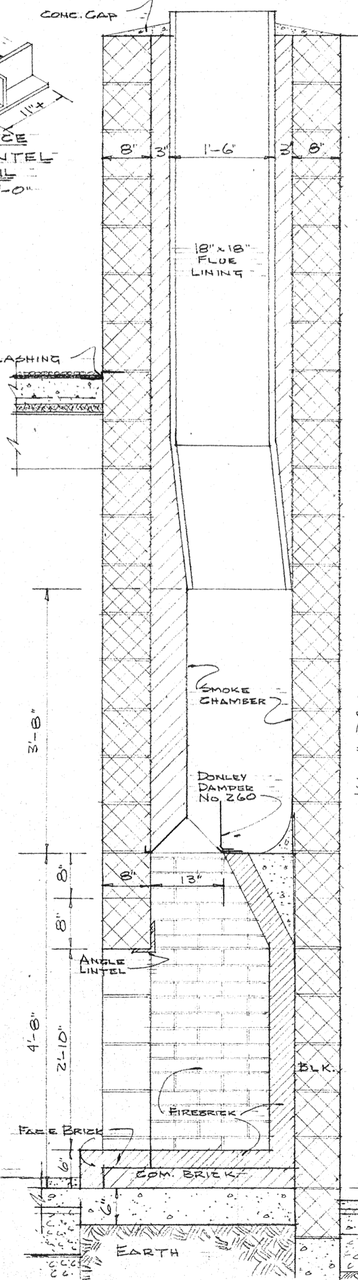
SECTION A-A 3/4" = 1'-0"
