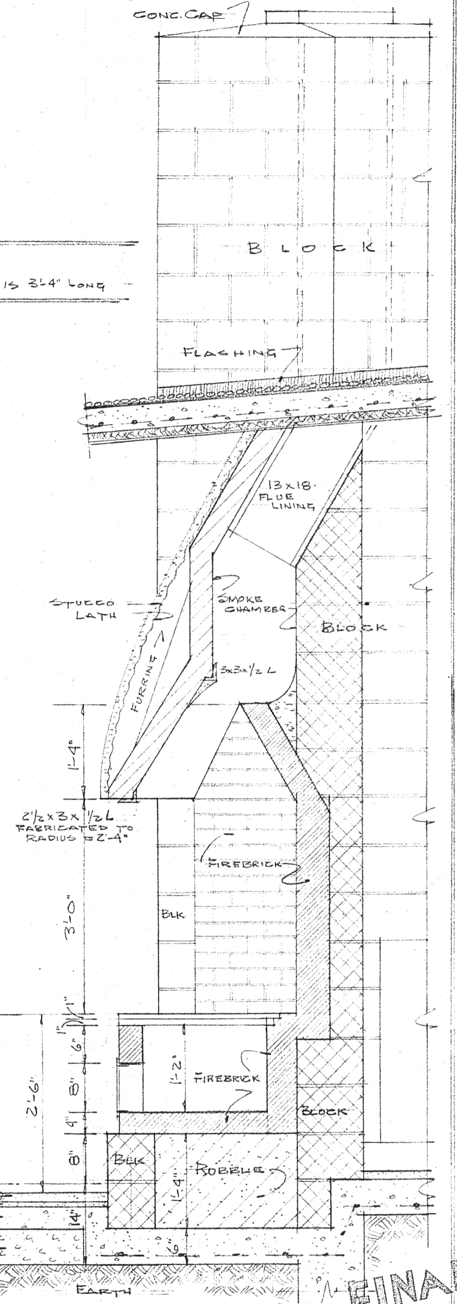
SECTION A-A 3/4" = 1'-0"
