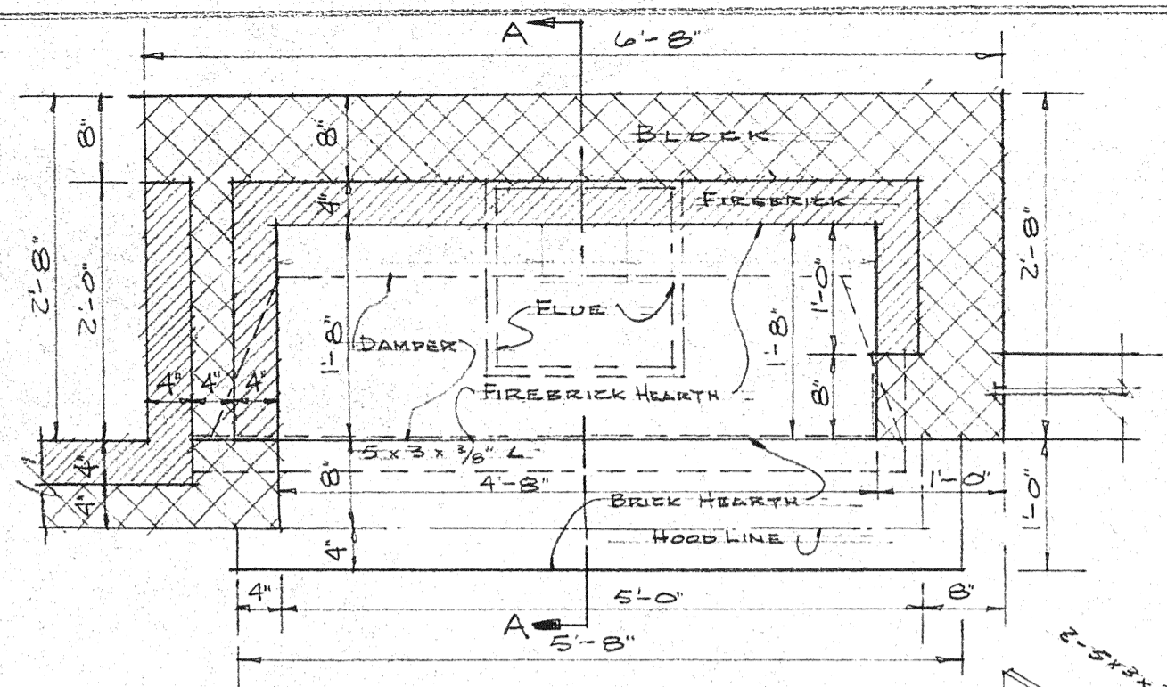
PLAN LIVING ROOM FIREPLACE 3/4" = 1'-0"
