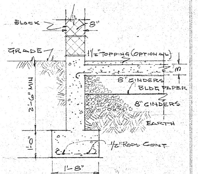
TYPICAL SECTION C-C 1/2" = 1'-0"
