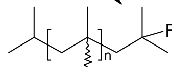
Fluor-Addition
