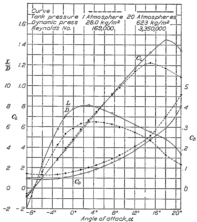
FIG. 19.—Characteristic curves of S. M. model with Clark Y wings and no propeller
