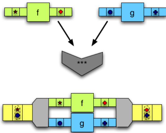
Figure 9: The (***) robot: running the combined arrow
