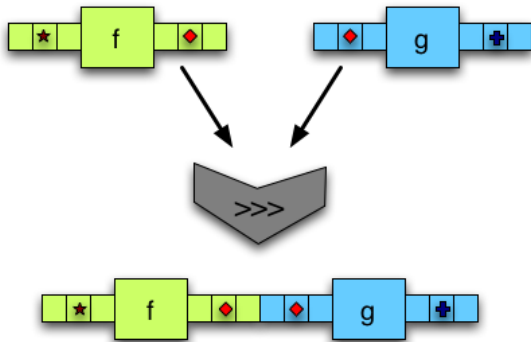
Figure 4: running the combined arrow
