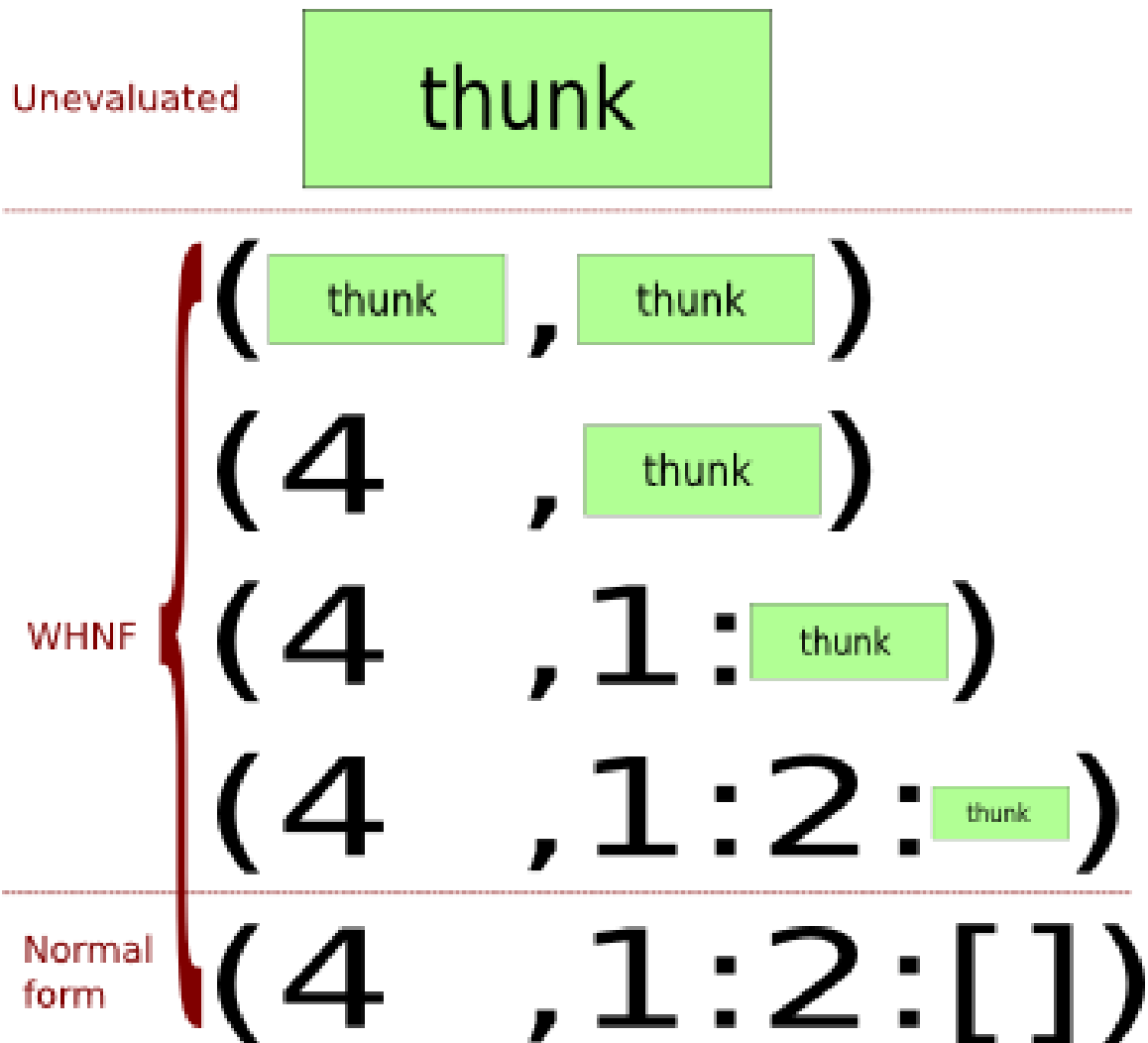
Figure 36: Evaluating the value (4, [1, 2]) step by step. The first stage is completely unevaluated; all subsequent forms are in WHNF, and the last one is also in normal form.
