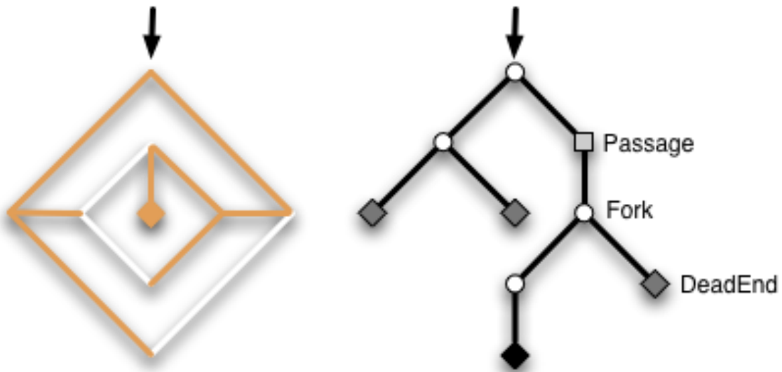
Figure 15: An example labyrinth and its representation as tree.
