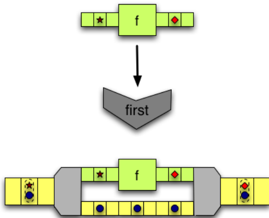
Figure 6: The combined arrow from the first robot
