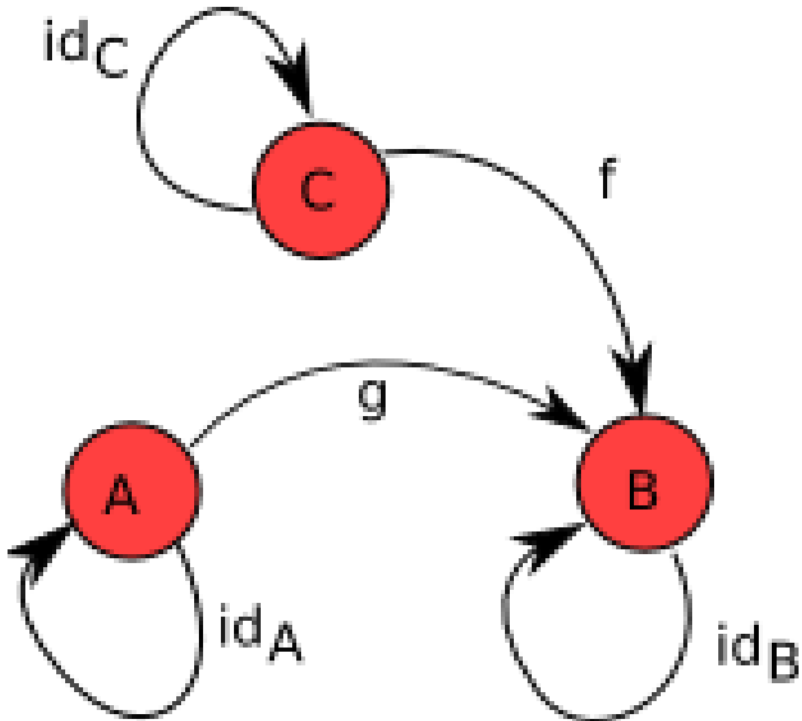
Figure 30: A simple category, with three objects A , B and C , three identity morphisms id_A , id_B and id_C , and two other morphisms f : C \rightarrow B and g : A \rightarrow B . The third element (the specification of how to compose the morphisms) is not shown.
