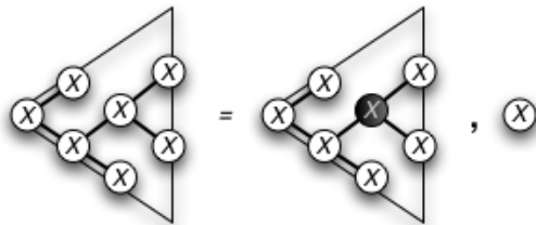
Figure 21: Removing a value of type X from a Tree\ X leaves a hole at that position.
