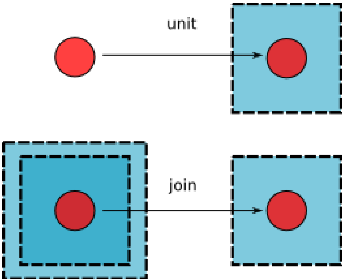
Figure 34: unit and join , the two morphisms that must exist for every object for a given monad.
