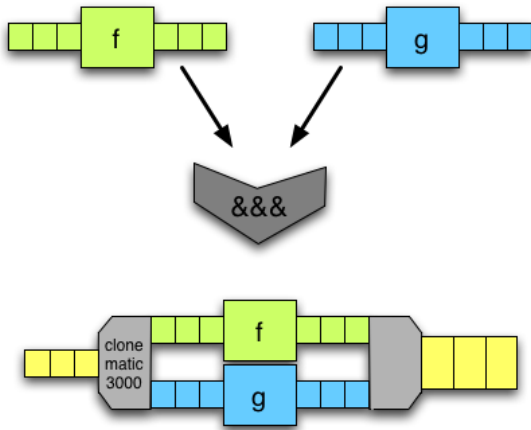
Figure 10: The &amp;&amp;&amp; robot
