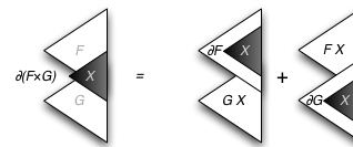
Figure 23 The hole in a one-hole context of a pair is either in the first or in the second component.
