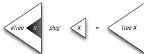
Figure 22: A more abstract illustration of plugging X into a one-hole context.
