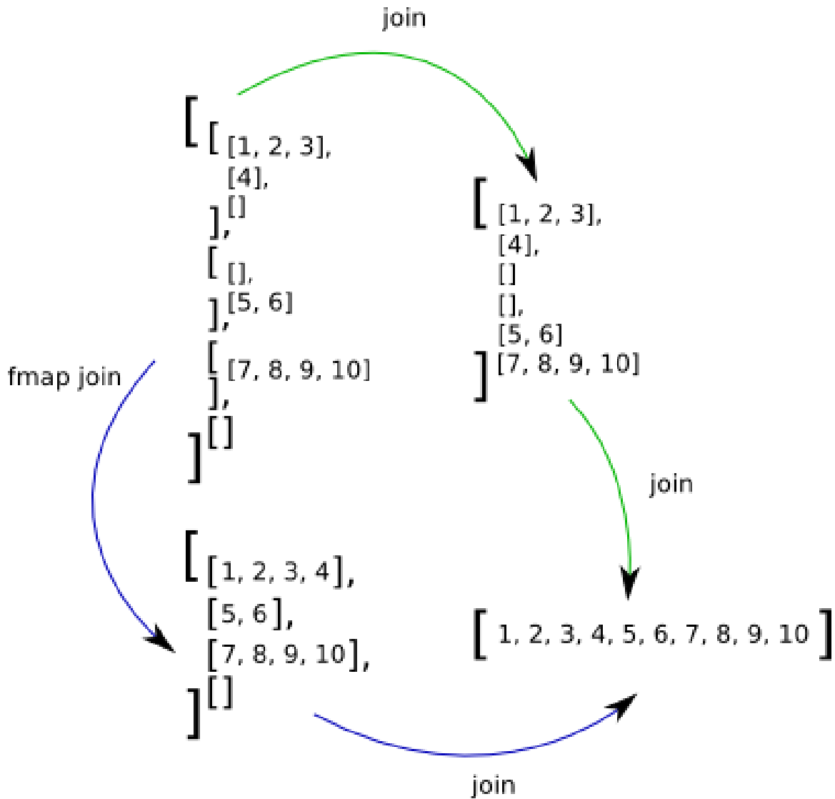
Figure 35: A demonstration of the first law for lists. Remember that join is concat and fmap is map in the list monad.
