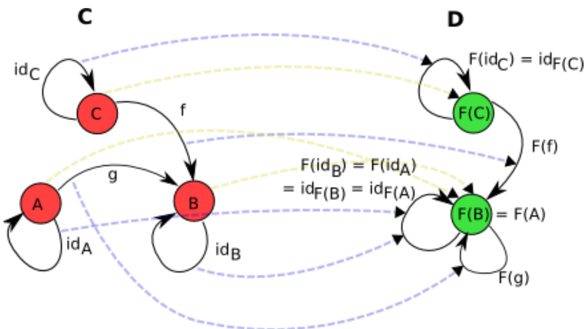
Figure 33: A functor between two categories, C and D . Of note is that the objects A and B both get mapped to the same object in D , and that therefore g becomes a morphism with the same source and target object (but isn't necessarily an identity), and id_A and id_B become the same morphism. The arrows showing the mapping of objects are shown in a dotted, pale olive. The arrows showing the mapping of morphisms are shown in a dotted, pale blue.
