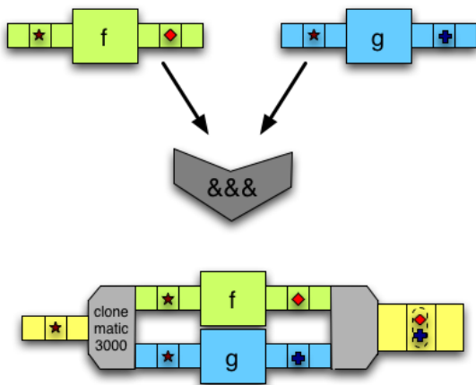
Figure 11: The &amp;&amp;&amp; robot: the resulting arrow with inputs
