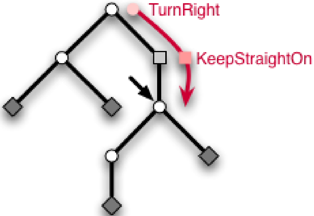
Figure 16: Representation of the player's position by Ariadne's thread.
