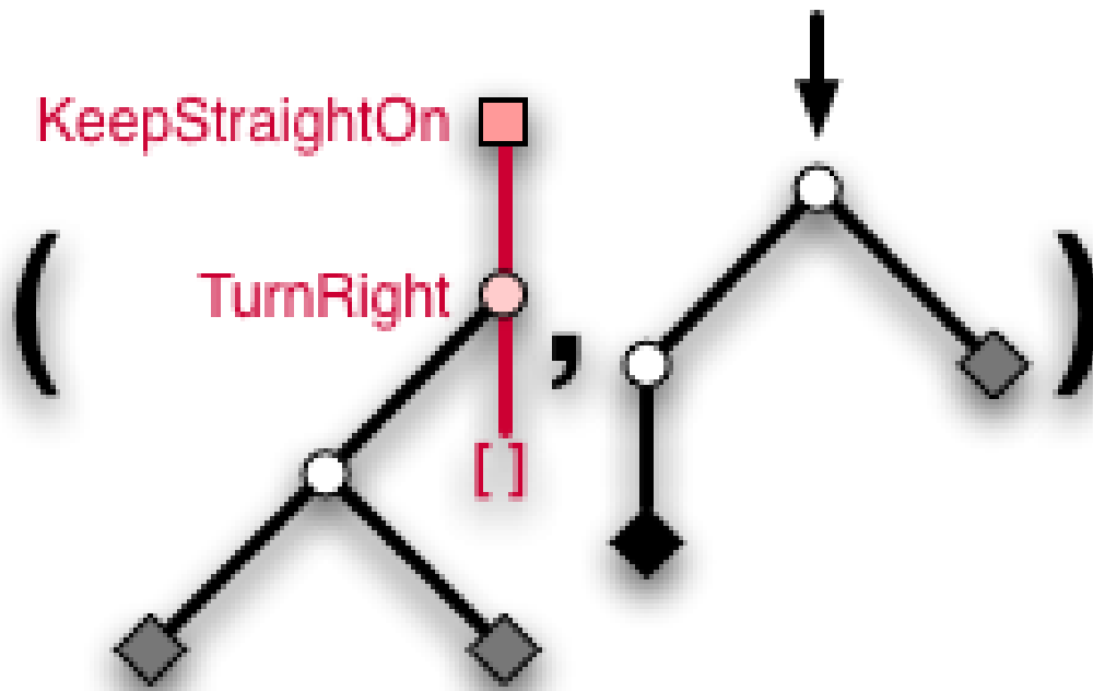
Figure 17: The zipper is a pair of Ariadne's thread and the current sub-labyrinth that the player stands on top. The main thread is colored red and has sub-labyrinths attached to it, such that the whole labyrinth can be reconstructed from the pair.
