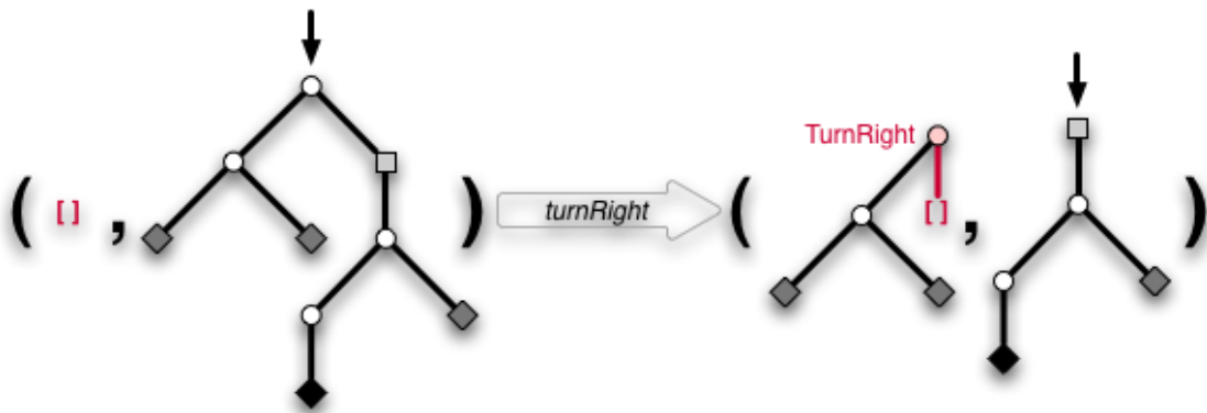
Figure 18: Taking the right subtree from the entrance. Of course, the thread is initially empty. Note that the thread runs backwards, i.e. the topmost segment is the most recent.
