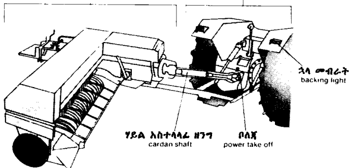
ተላላፊ ግጭድ reciprocating knife mower
