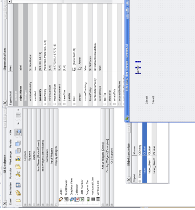
Abb. 11 Unser Dialogfenster
