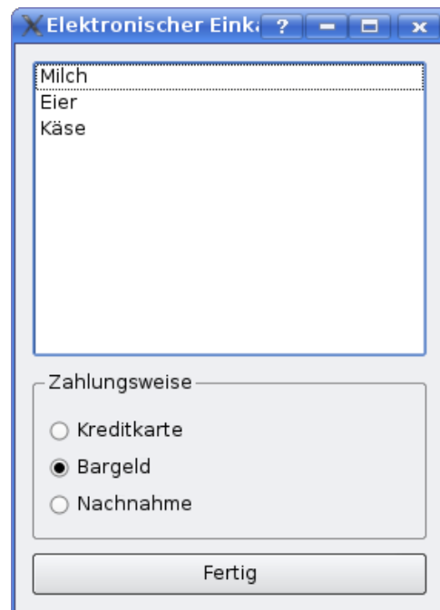
Abbildung 9: guiqt3.py Dialogfenster
