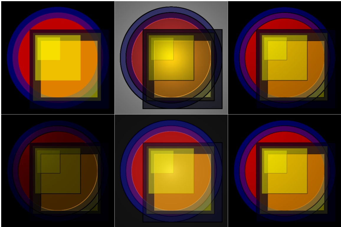
Abb. 368 Animation
