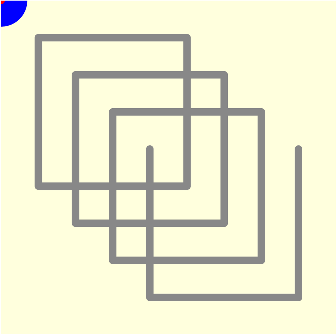
Abb. 260 kumulative animateMotion
