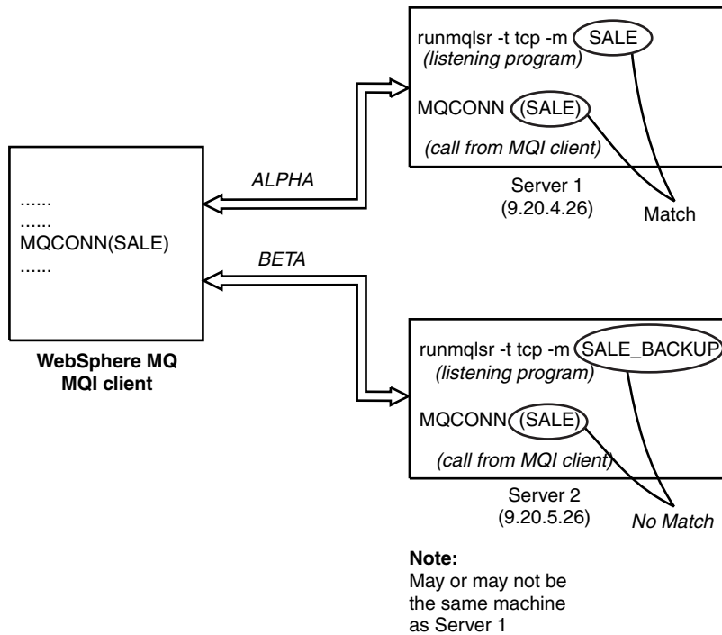
Figure 82. MQCONN example
