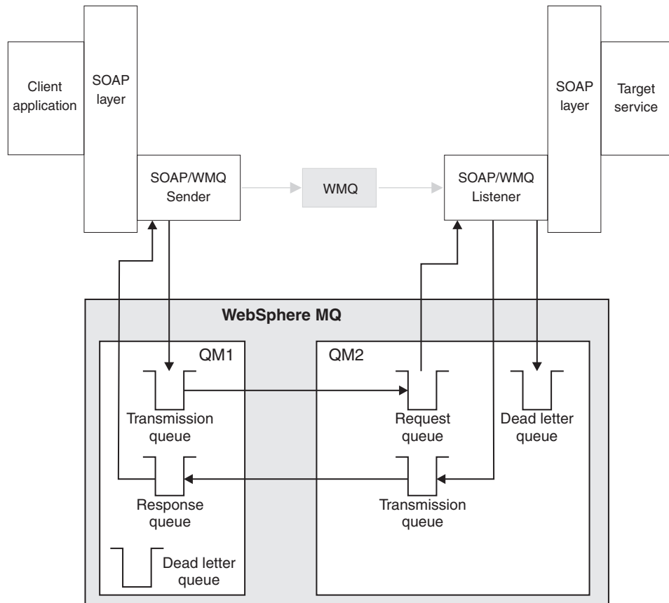
Figure 196. Queues used by SOAP/WebSphere MQ (separate queue managers)
