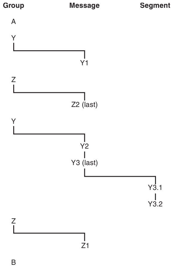
Figure 45. Physical order on a queue
