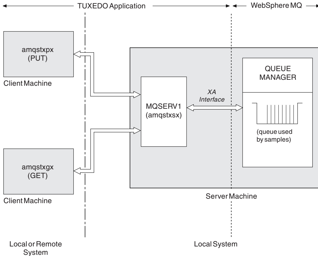
Figure 28. How TUXEDO samples work together
