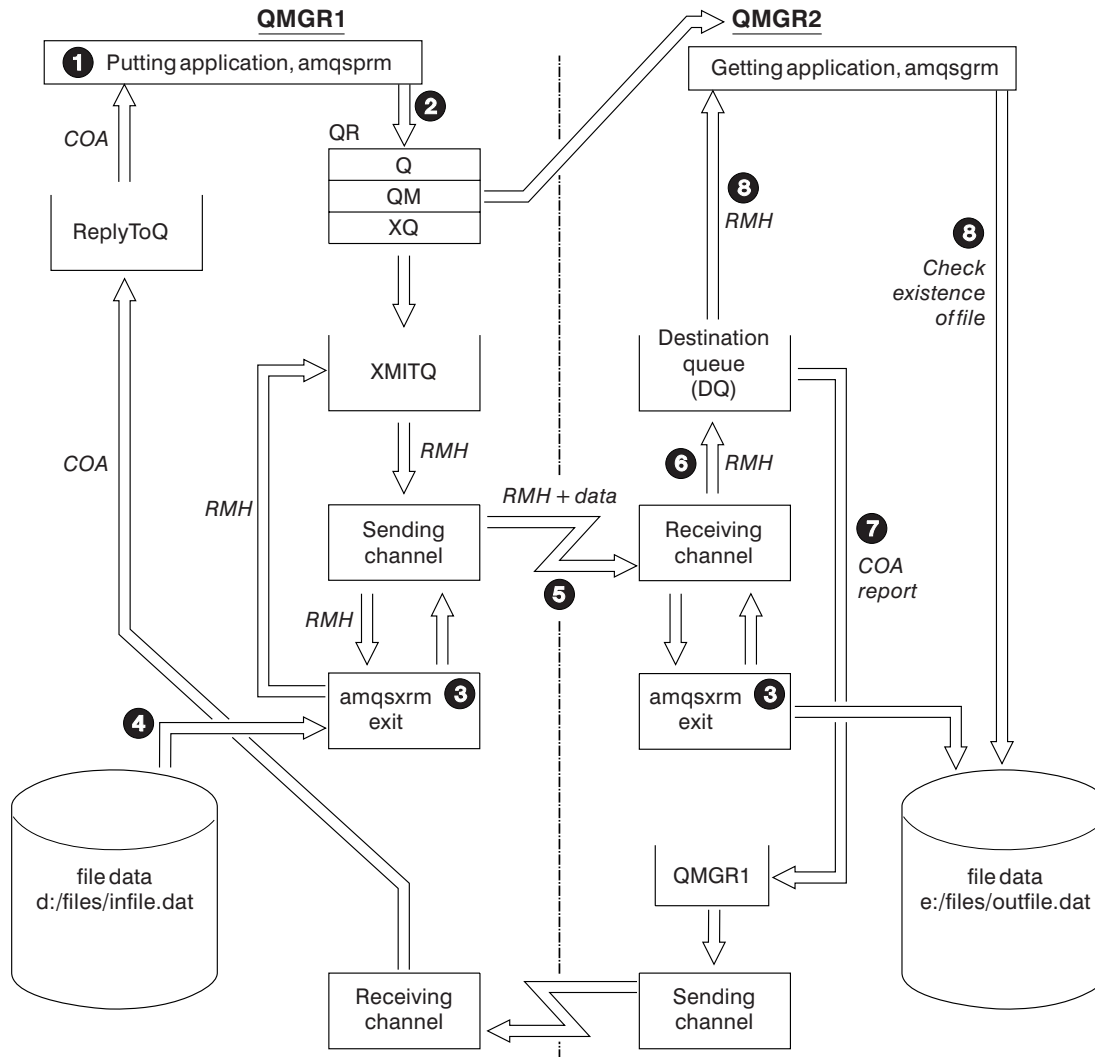
Figure 21. Running the Reference Message samples
