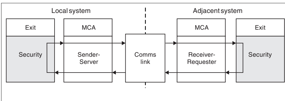
Figure 89. Security exit loop
