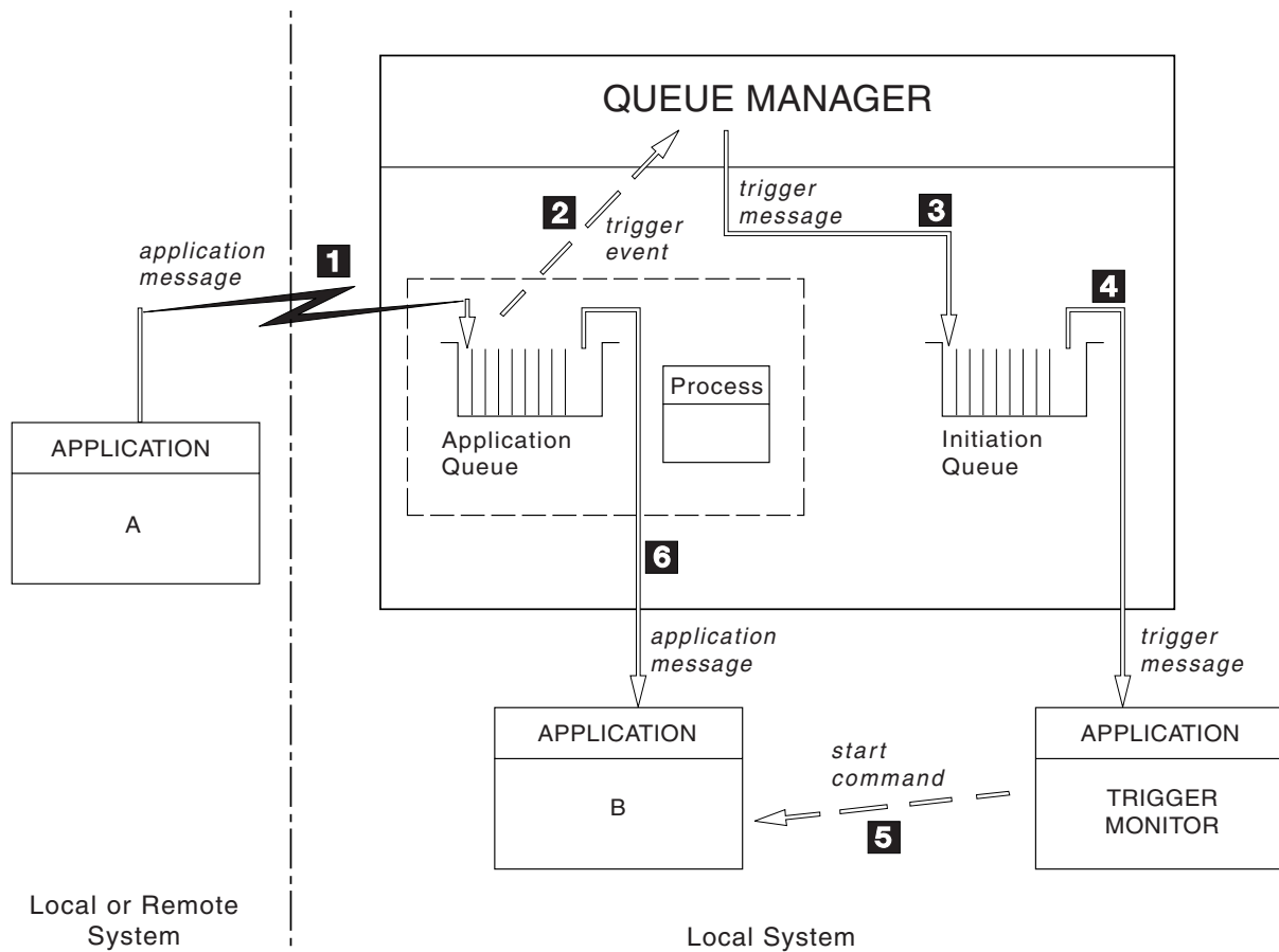
Figure 78. Flow of application and trigger messages
