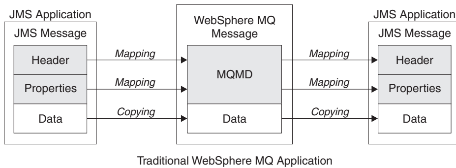
Figure 156. How JMS messages are transformed to WebSphere MQ messages with no MQRFH2 header
