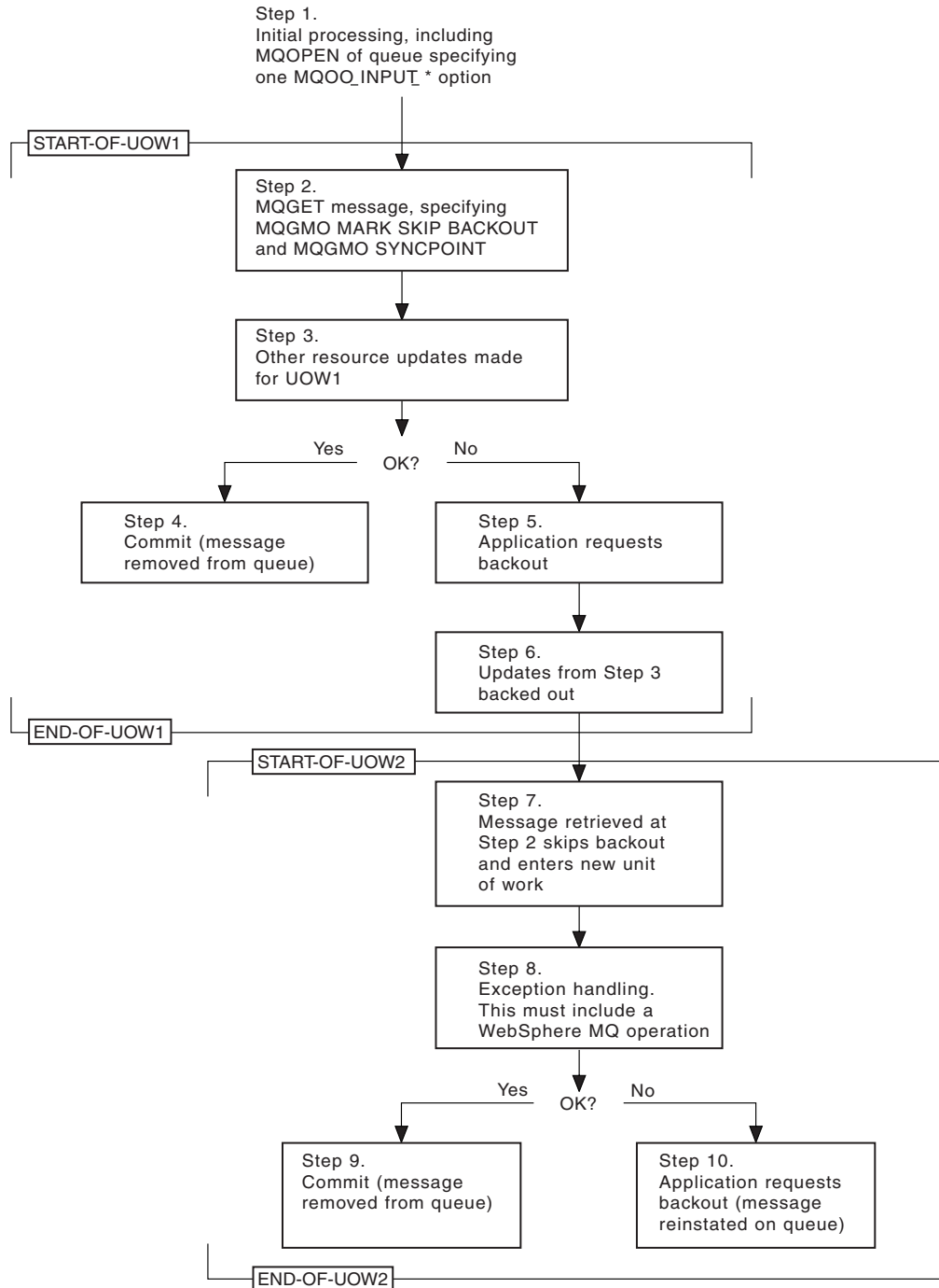
Figure 46. Skipping backout using MQGMO_MARK_SKIP_BACKOUT
