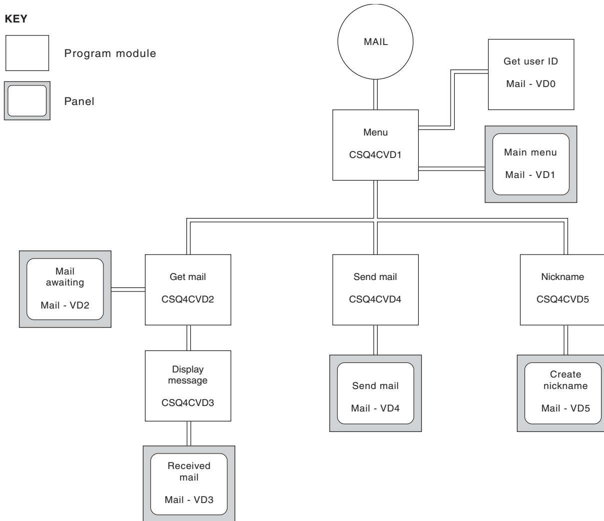
Figure 31. Programs and panels for the CICS version of the Mail Manager
