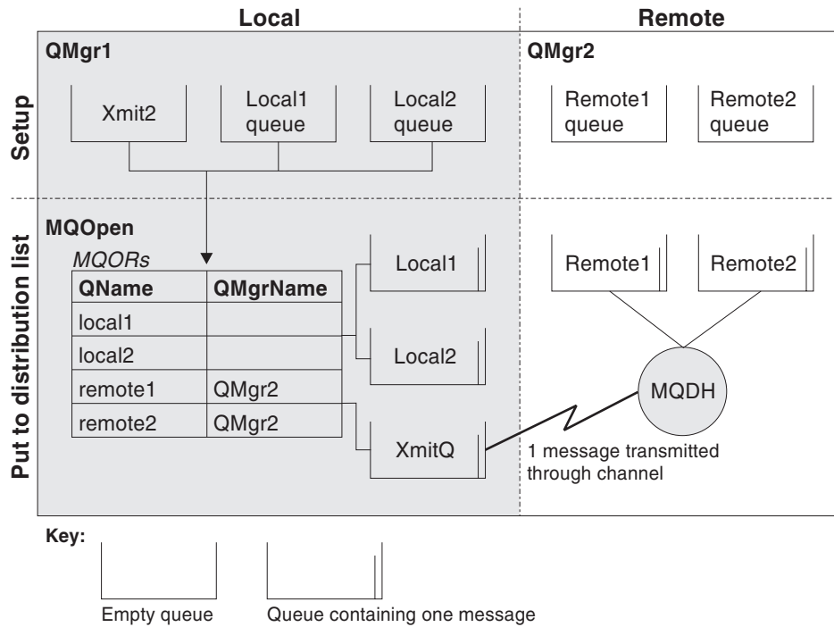
Figure 39. How distribution lists work. This diagram shows that one message is transmitted through the channel and can be put on more than one remote queue.
