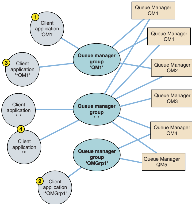
Figure 81. Queue manager groups
