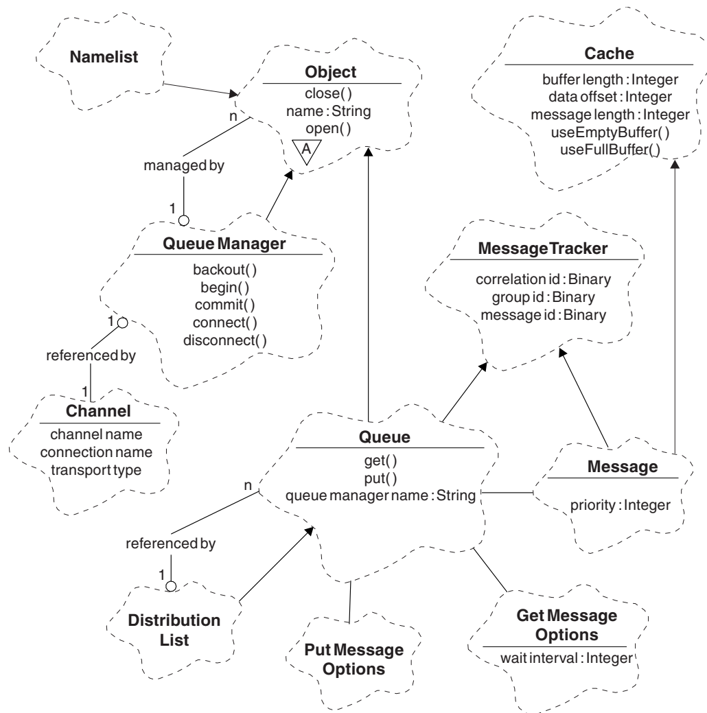
Figure 148. WebSphere MQ C++ classes (queue management)
