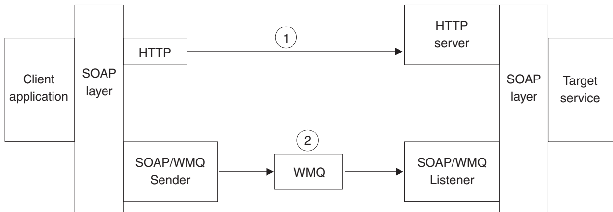
Figure 194. Overview of WebSphere MQ transport for SOAP
