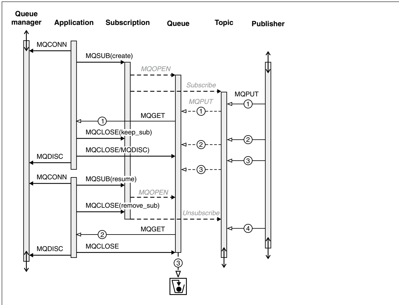
Figure 67. Managed durable subscriber lifelines
