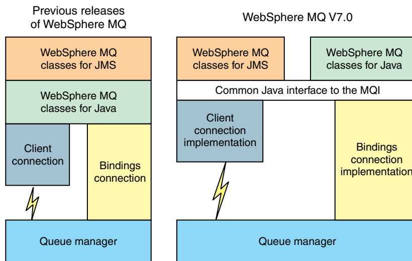
Figure 153. The relationship between WebSphere MQ classes for JMS and WebSphere MQ classes for Java
