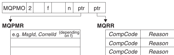
Figure 42. Putting a message to a distribution list in C. The MQPMO uses pointers to the MQPMR and MQRR structures.
