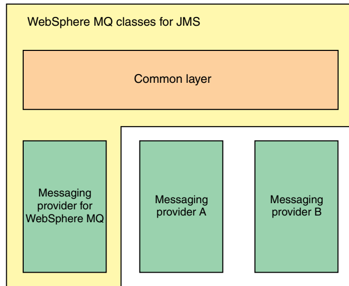
Figure 152. The layered architecture for IBM JMS providers
