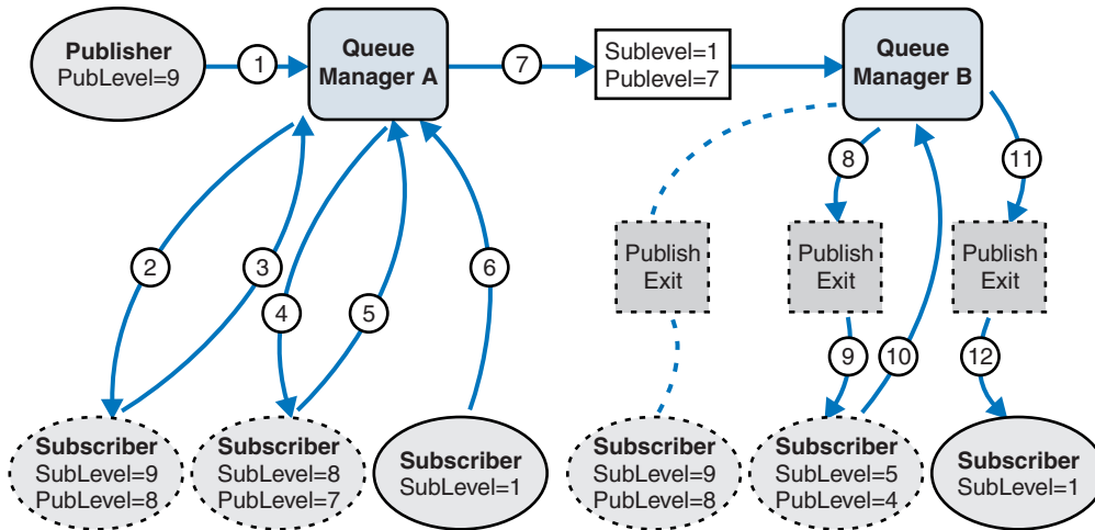
Figure 77. Complex deployment of intercepting subscribers
