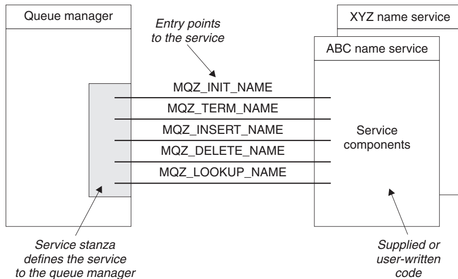
Figure 83. Understanding services, components, and entry points
