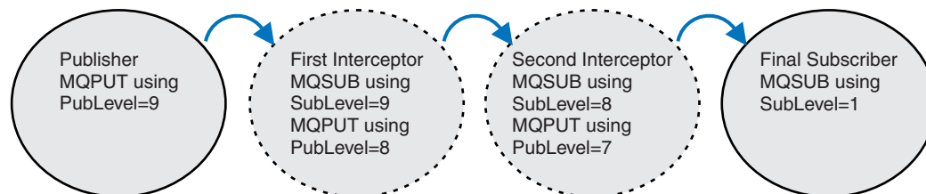
Figure 69. Sequence of intercepting subscribers
