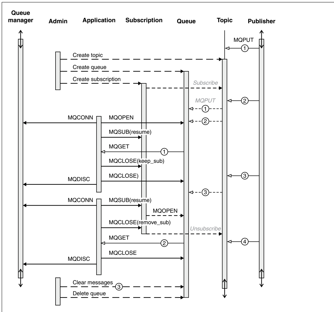
Figure 68. Unmanaged durable subscriber lifelines
