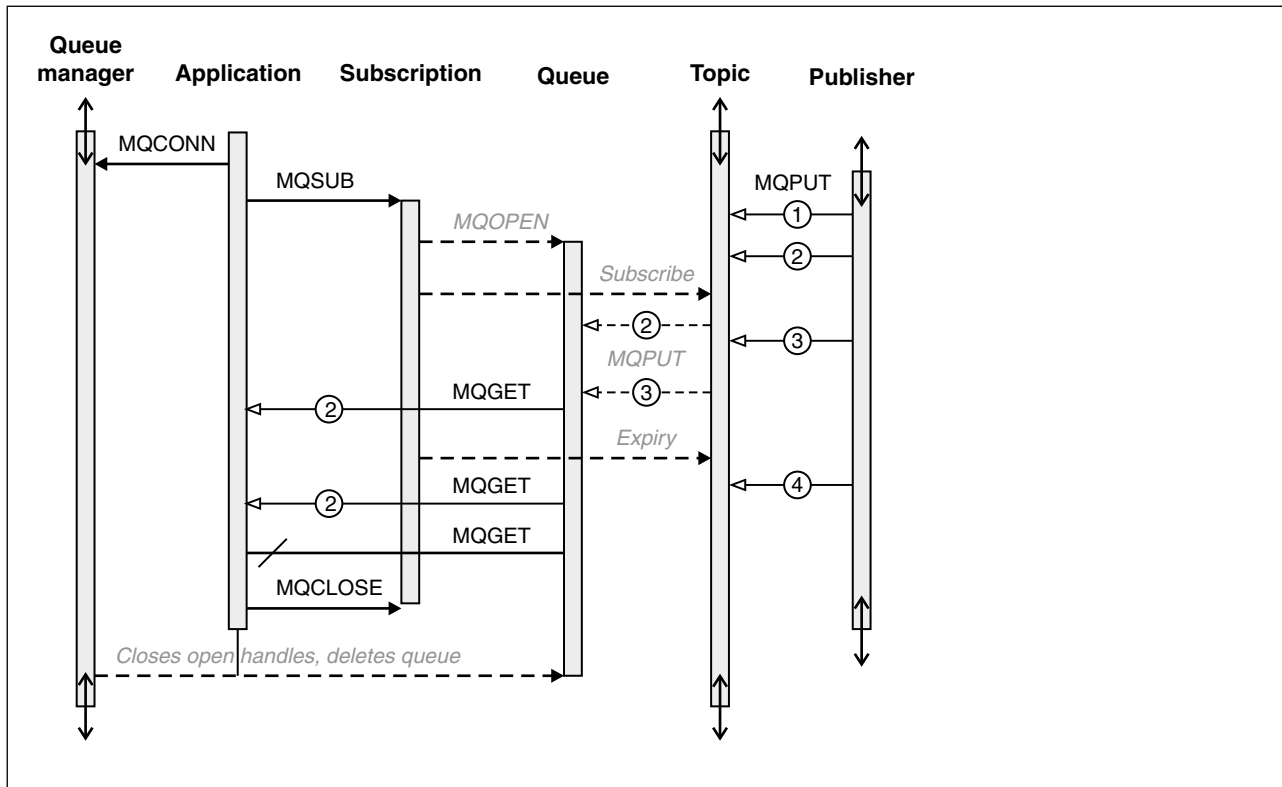
Figure 66. Managed non-durable subscriber lifelines
