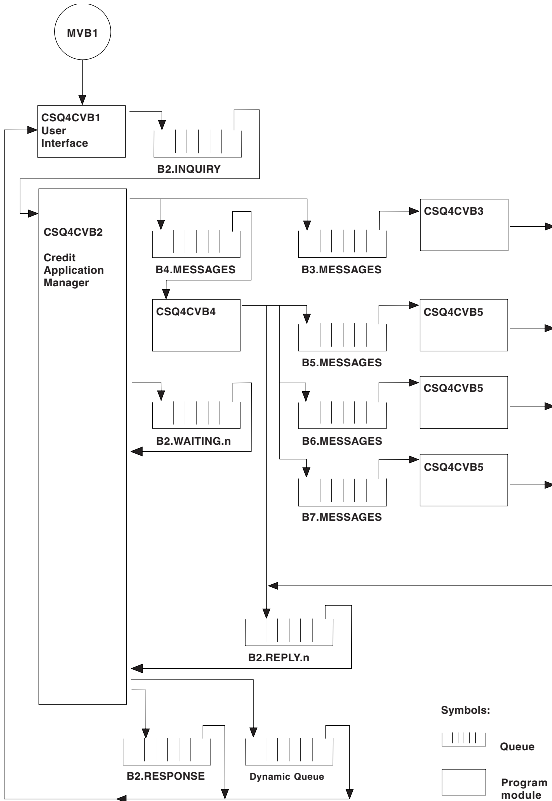
Figure 35. Programs and queues for the Credit Check sample application (COBOL programs only). In the sample application, the queue names shown in this figure have the prefix CSQ4SAMP.
