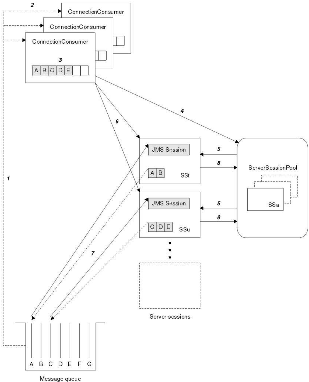
Figure 192. ServerSessionPool and ServerSession functionality
