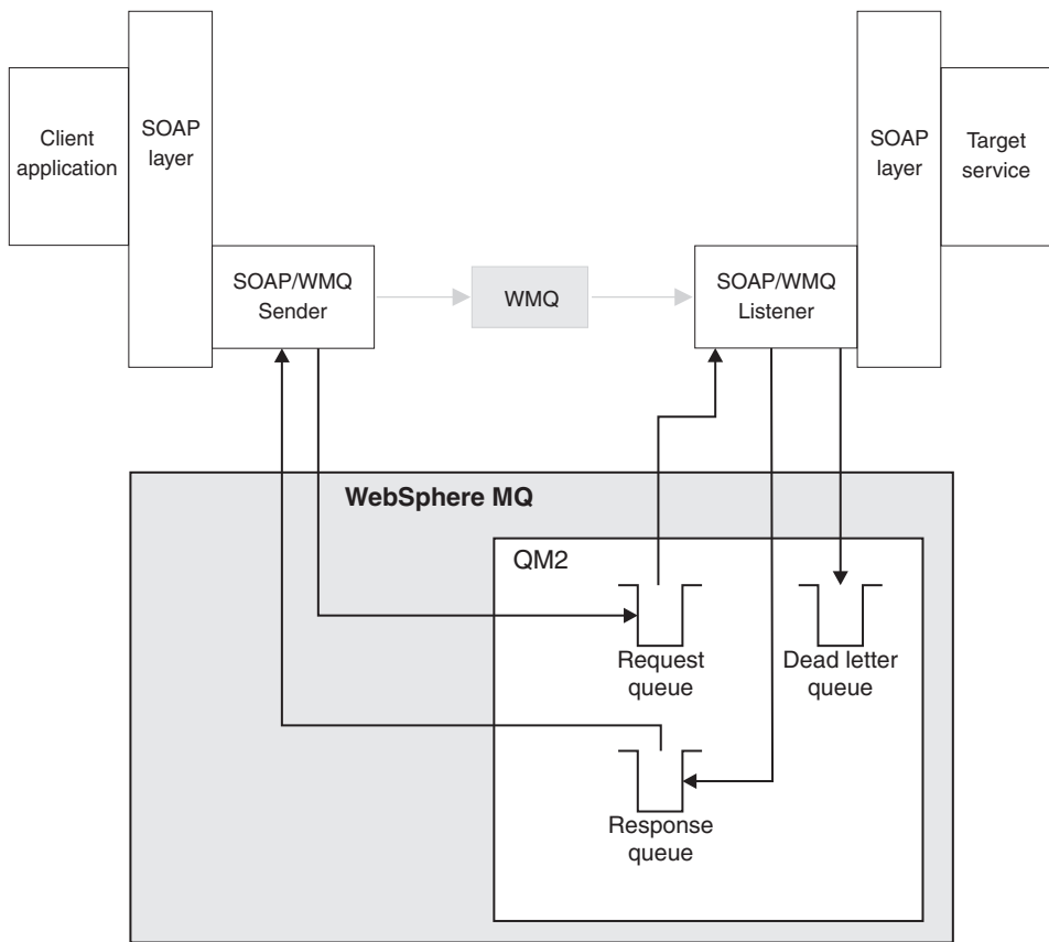
Figure 195. Queues used by SOAP/WebSphere MQ (single queue manager)
