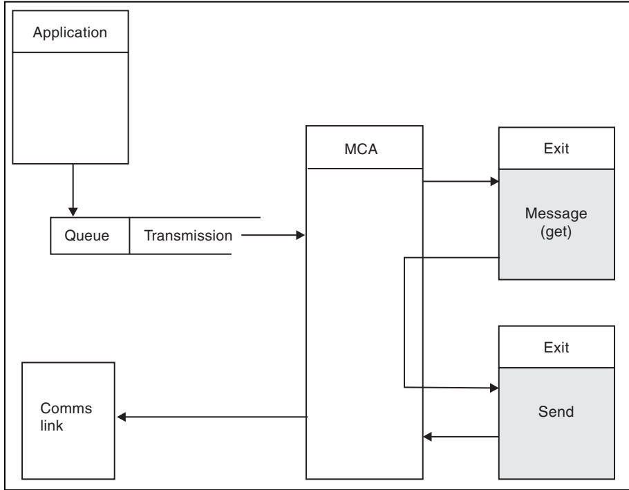
Figure 90. Example of a send exit at the sender end of message channel
