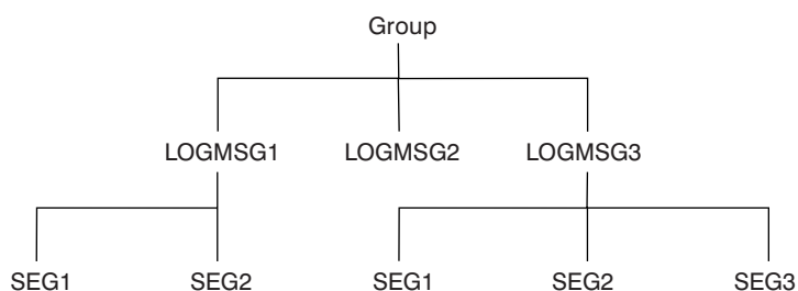
Figure 8. Segmented messages
