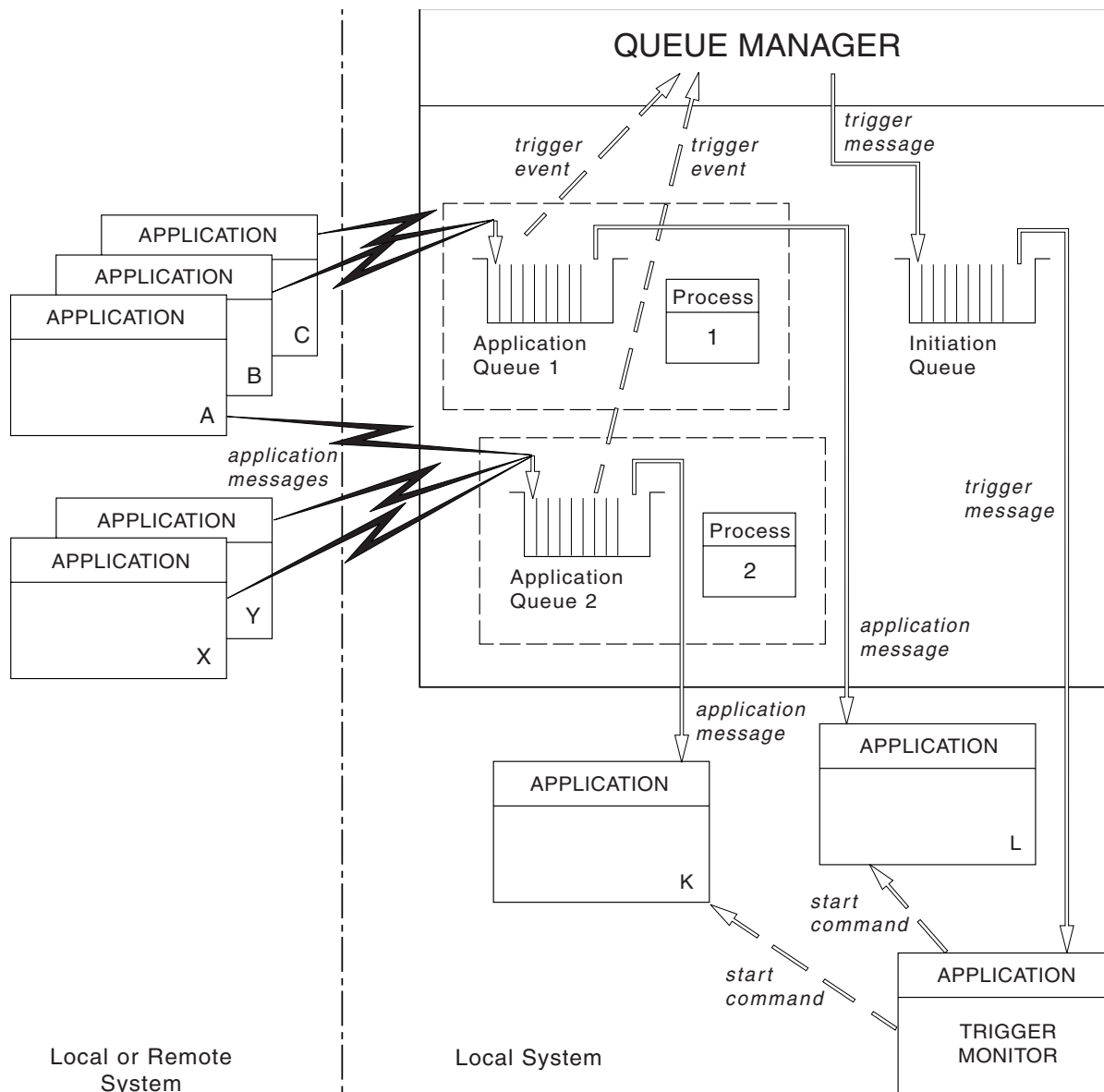
Figure 79. Relationship of queues within triggering
