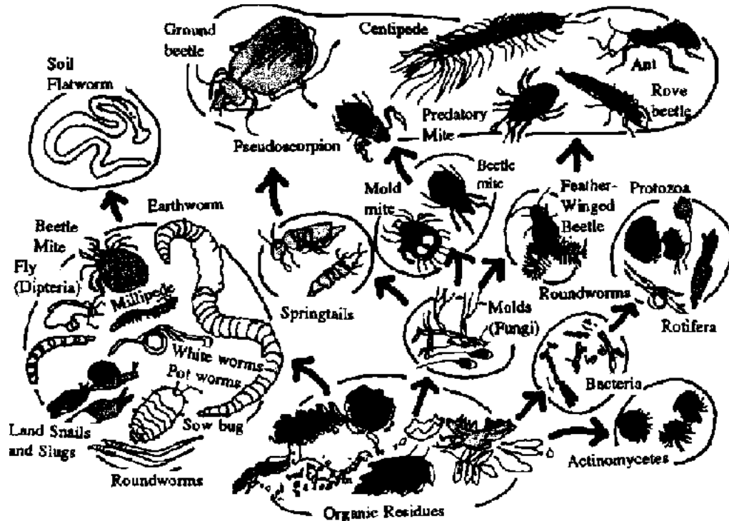
Figure 2: Food web of the compost pile (D. Dindal)
