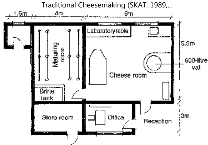
Figure 20. Plan of a 600-litre-capacity cheese factory (1:75 scale)
