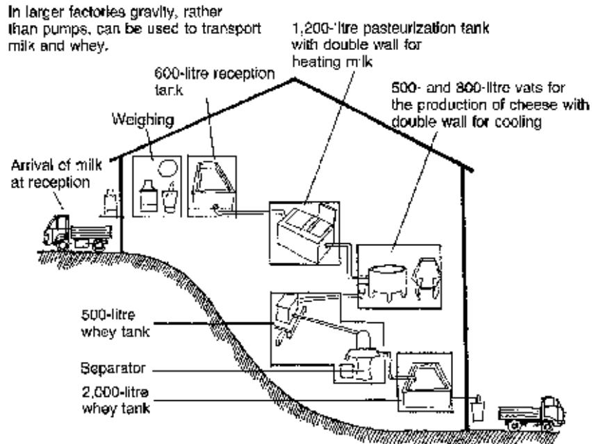
Figure 19. Gravity circuit of a 2,000-litre cheese factory
