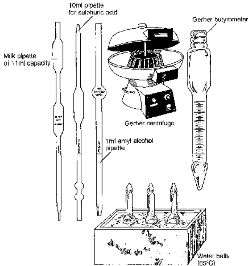
Figure 8. Equipment for testing fat content
