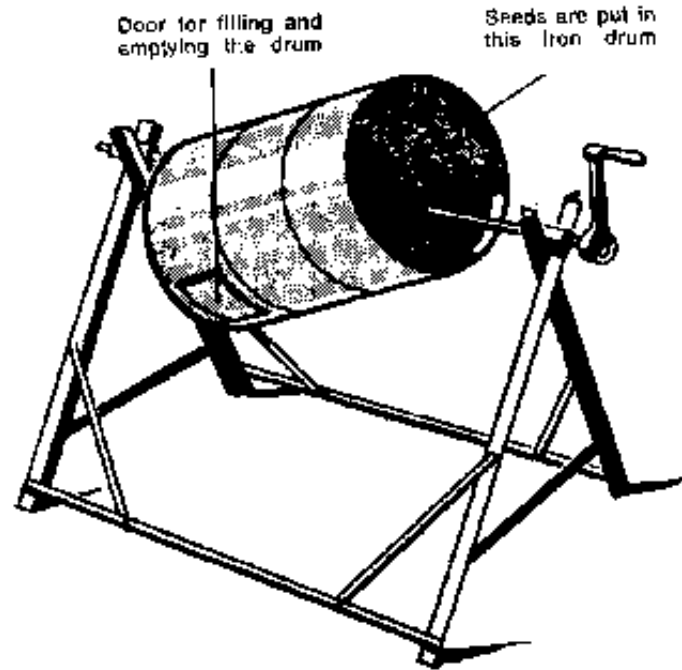
Device for disinfecting seeds
