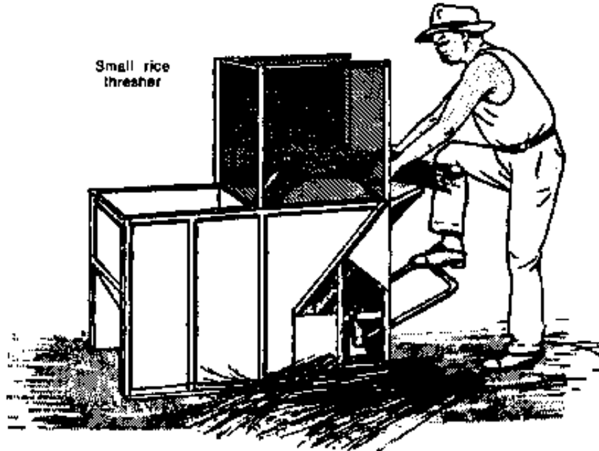
Small rice thresher
