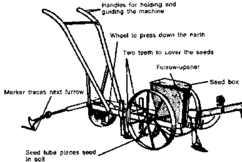
Seed drill
