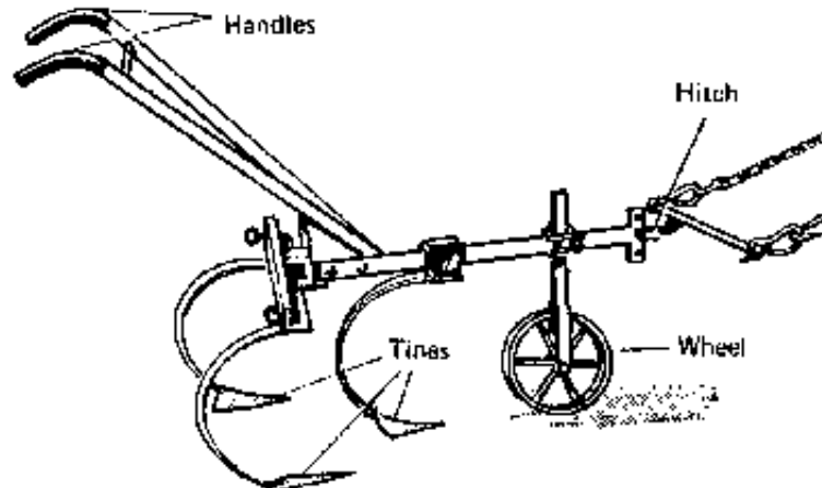
Animal- drawn cultivator
