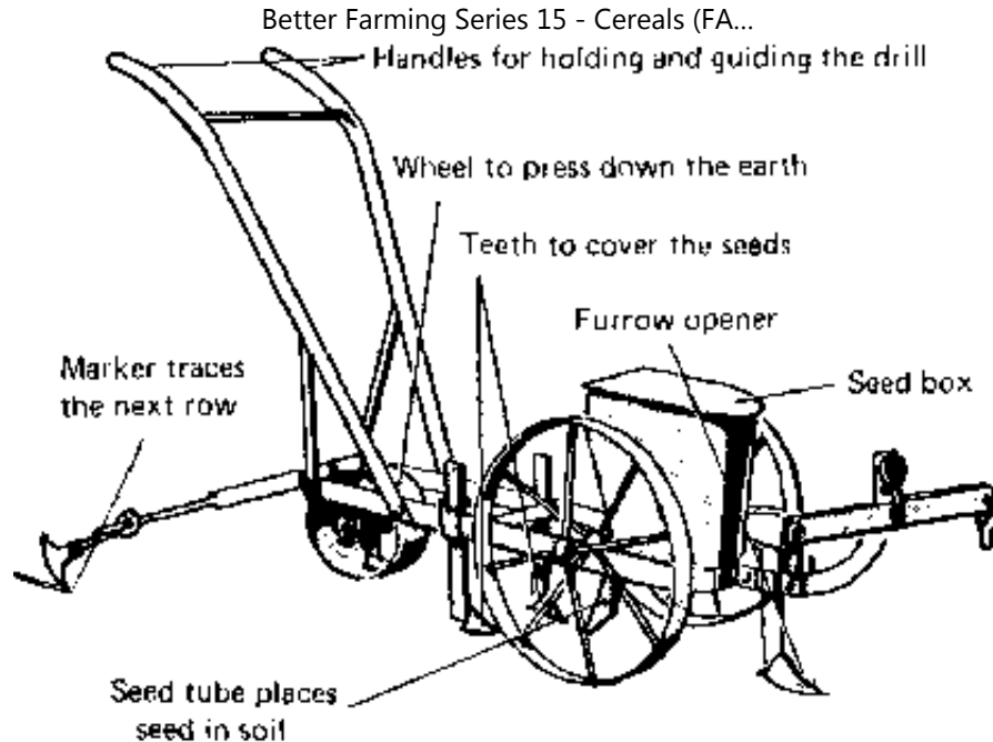
Seed drill
