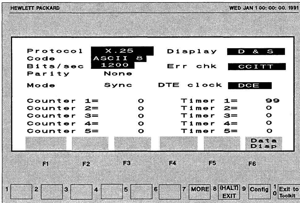
Figure 5-4: Timers and Counters
