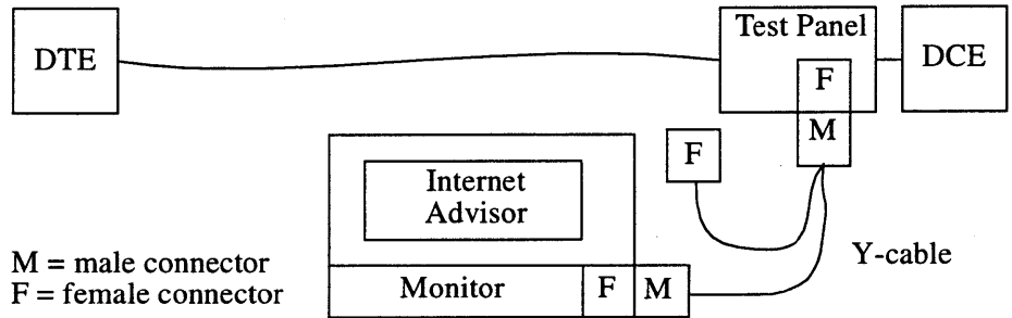
Figure 2-2: V-Series Passive Monitor Test Panel Connection
