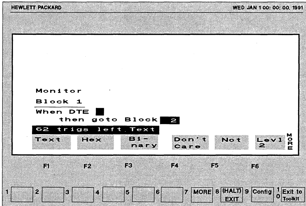
Figure 4-3: Defining a Trigger
