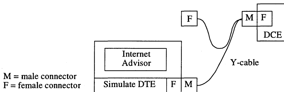
Figure 2-4: V-Series Active Connections to Test DCE and Link
