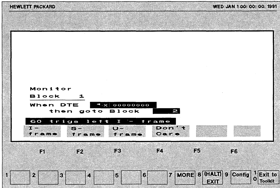
Figure 4-4: Selecting an Information Frame
