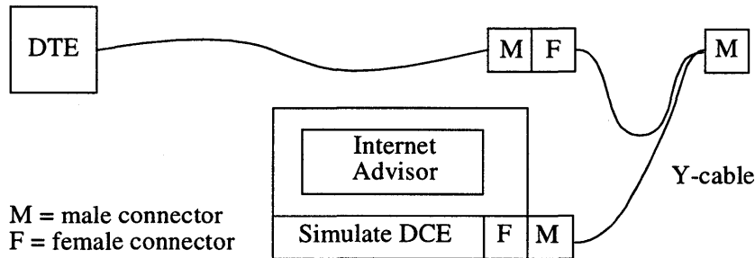
Figure 2-3: V-Series Active Connection to Test Terminal Device
