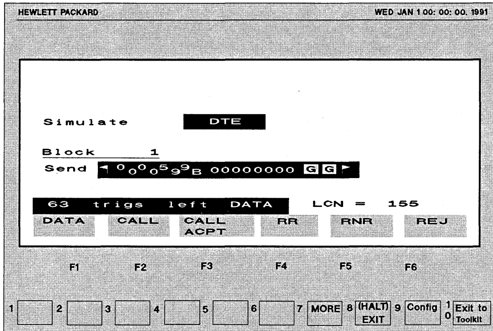
Figure 4-8: Mod 8 and LCN in Level 3 Send String
