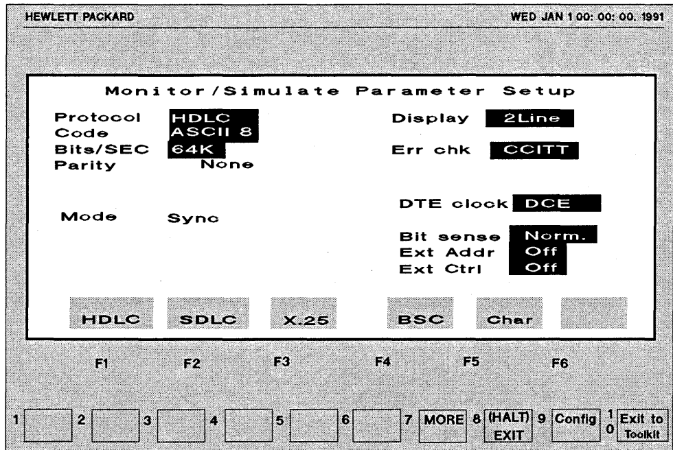
Figure 4-1: The Setup Menu
