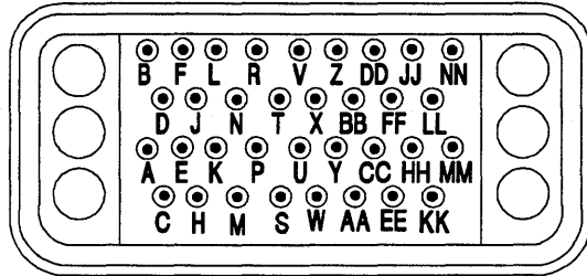
Figure 1-4: V.35 Interface Connector Pins Assignment
