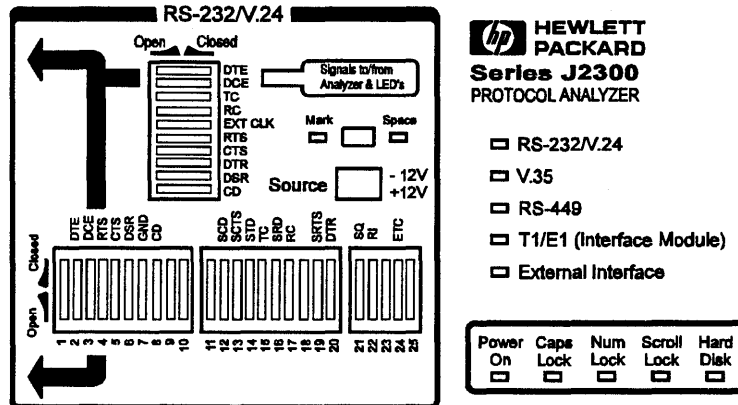
Figure 1-1: RS-232/V.24 Breakout Box
