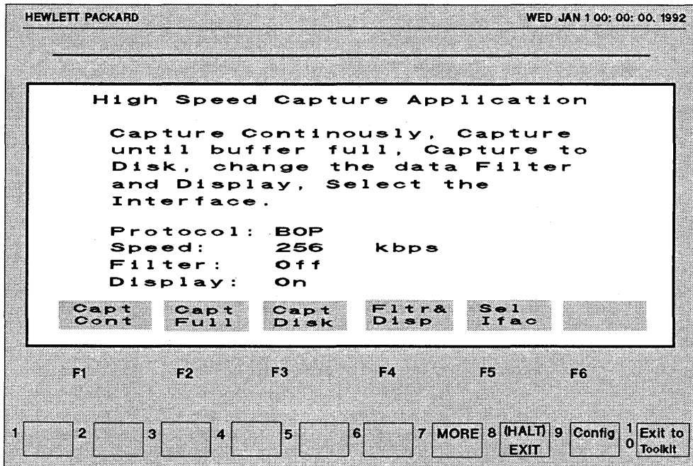
Figure 9-2: Selection Screen for High Speed Capture
