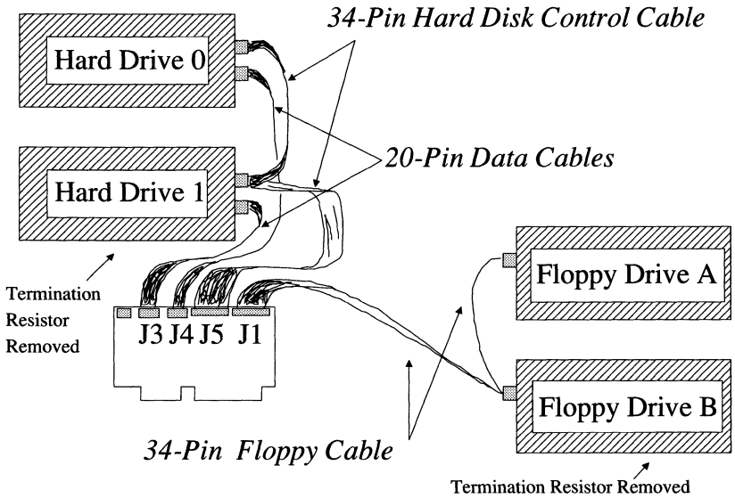
FIGURE 2-6. INSTALLATION
