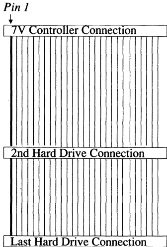
Cable without a twist
