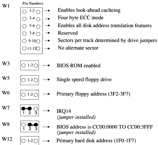
FIGURE 2-3. DEFAULT JUMPER SETTINGS
