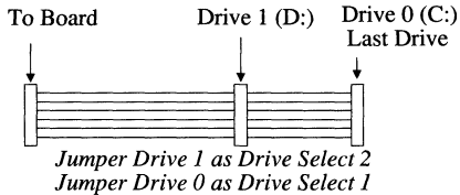
FIGURE 2-1. HARD DISK DRIVE SELECT & CABLES
