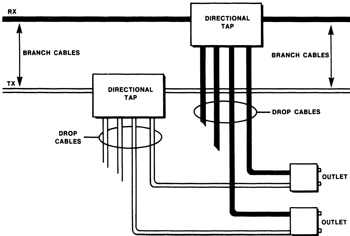
Figure 2-25 Directional Tap Application
