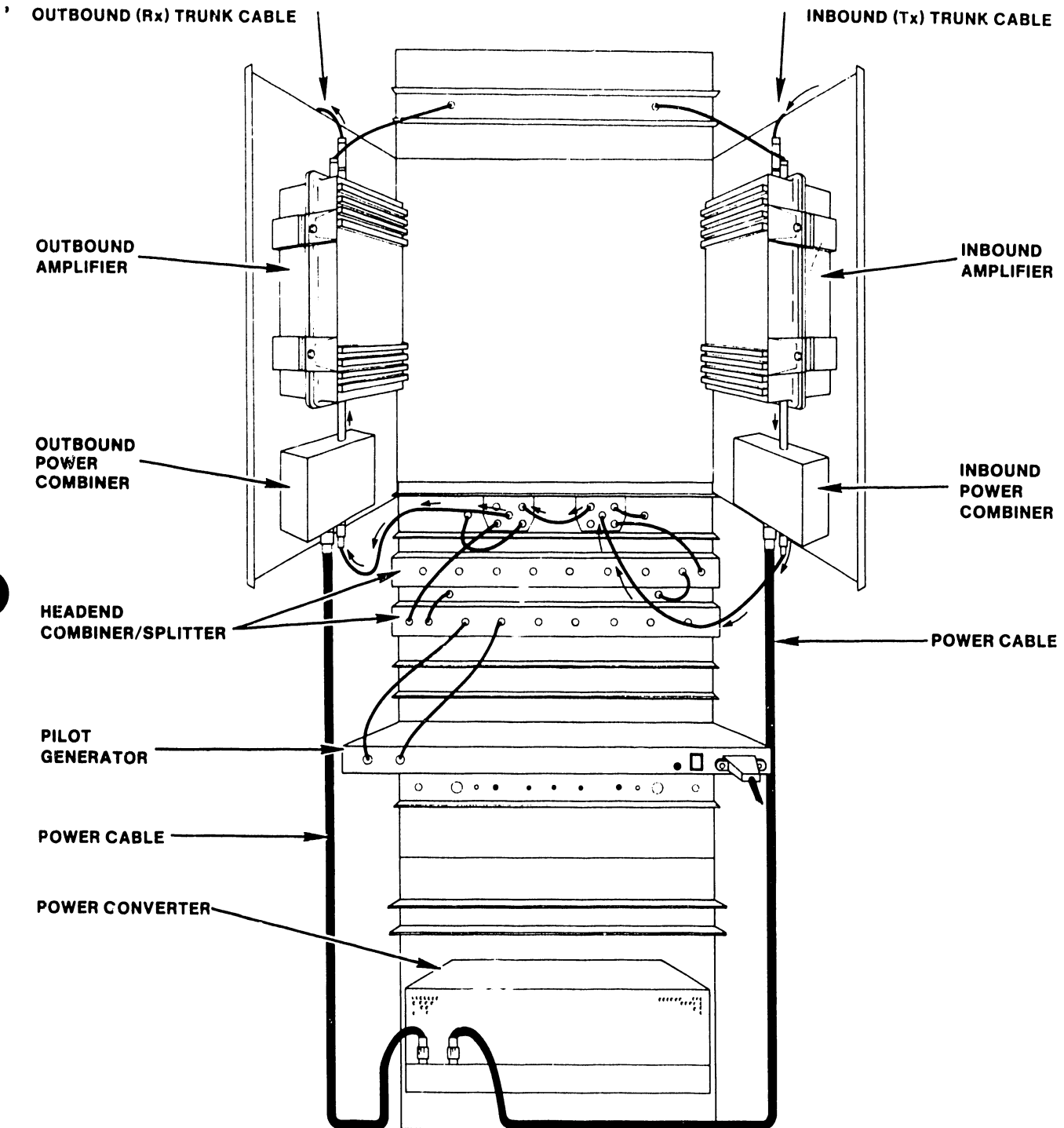
TYPICAL HEADEND, REARVIEW
