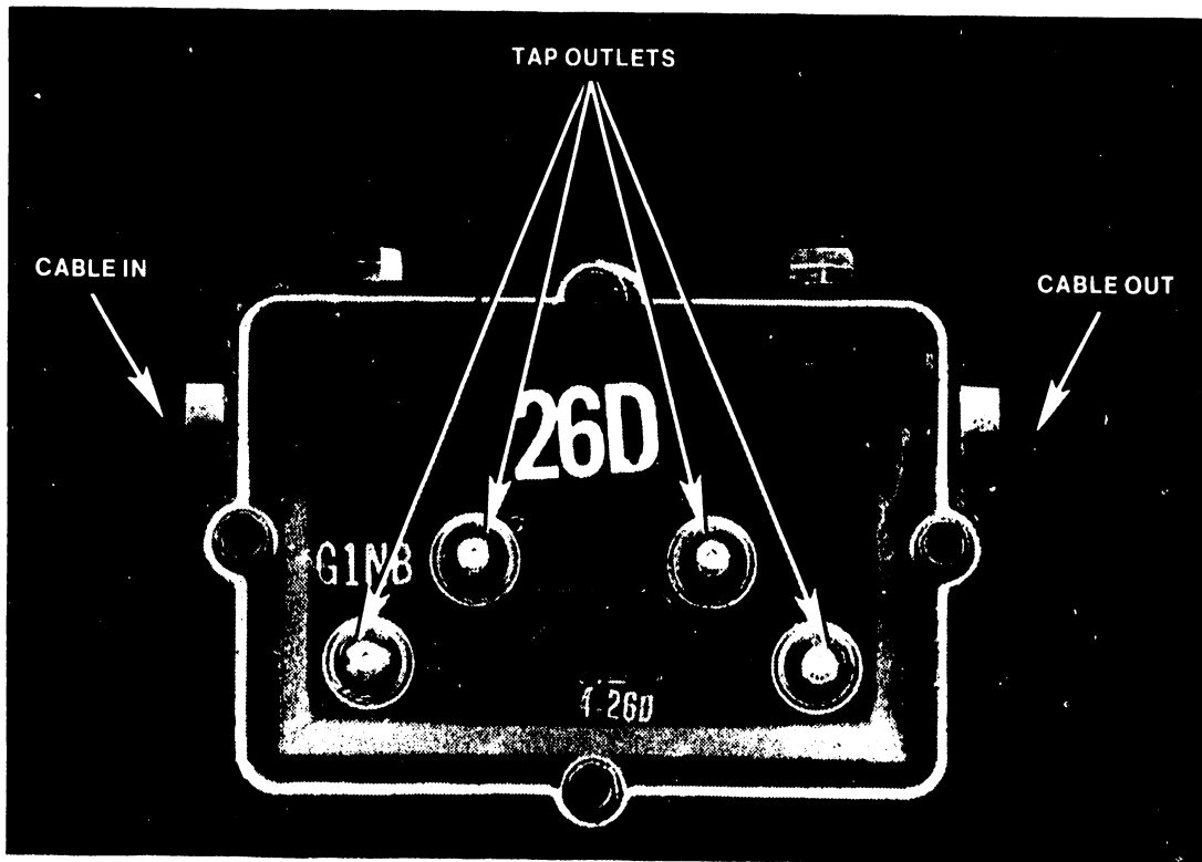
Figure 2-26 Typical Directional Tap Exterior View
