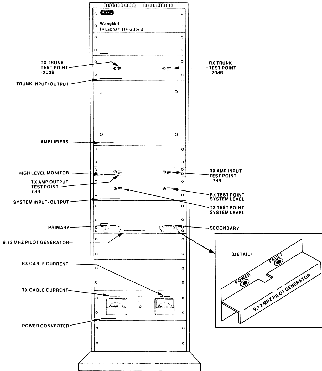
TYPICAL HEADEND, FRONT VIEW
