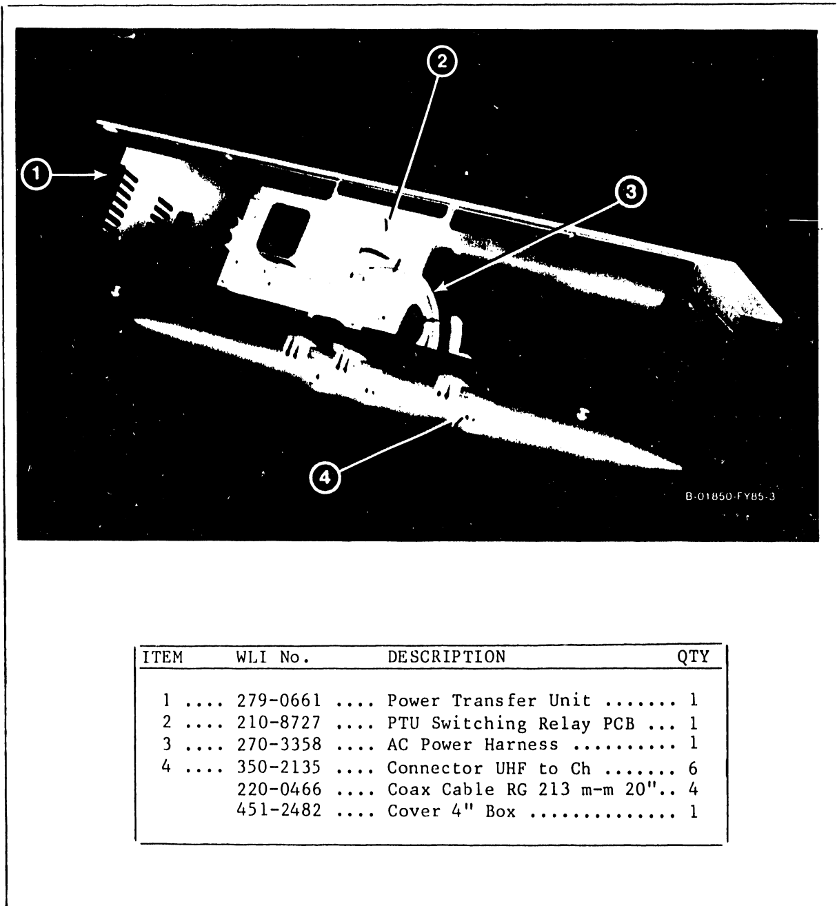
Figure G-5 Illustrated Parts Breakdown
