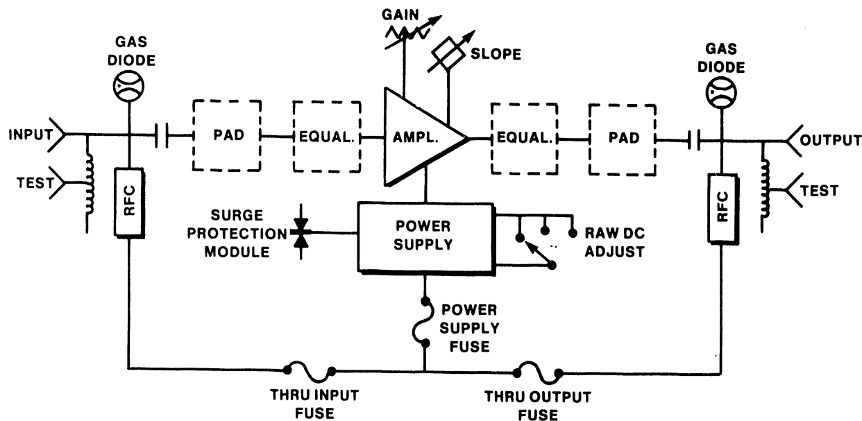
Figure 2-5 Amplifier Block Diagram
