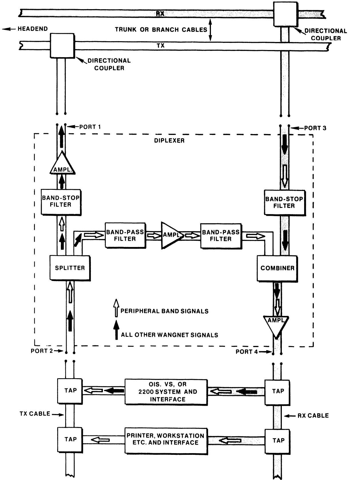
Figure 2-12 Diplexer Block Diagram
