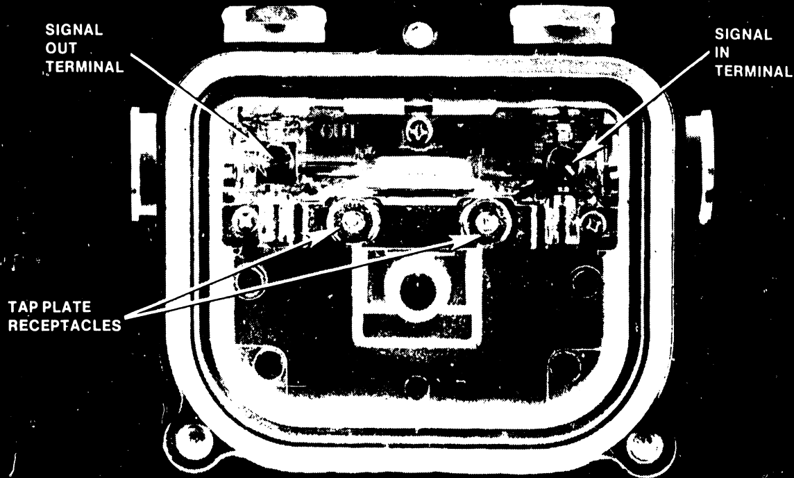
RMS CA-4500 TAP CASE INTERIOR VIEW
