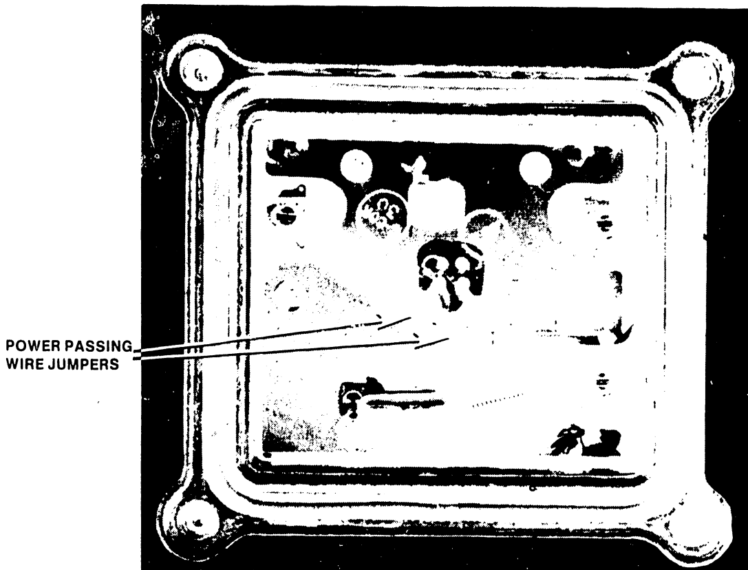
Figure 2-34 Typical Power Combiner Interior View
