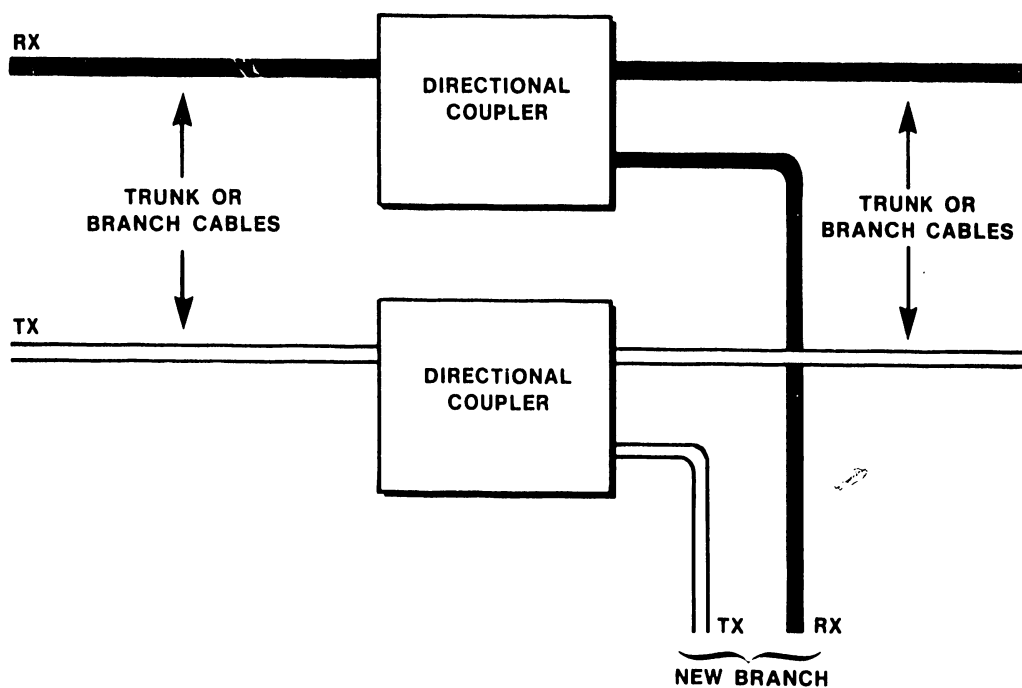
Figure 2-21 Directional Coupler Application
