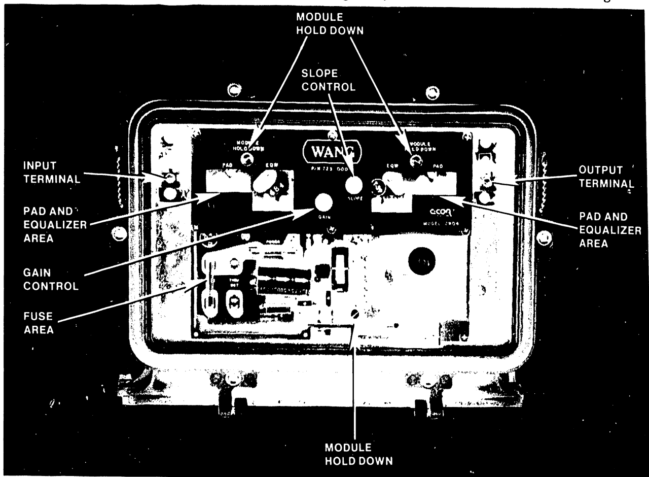
Figure 5-10 Wang Model 2904 Amplifier
