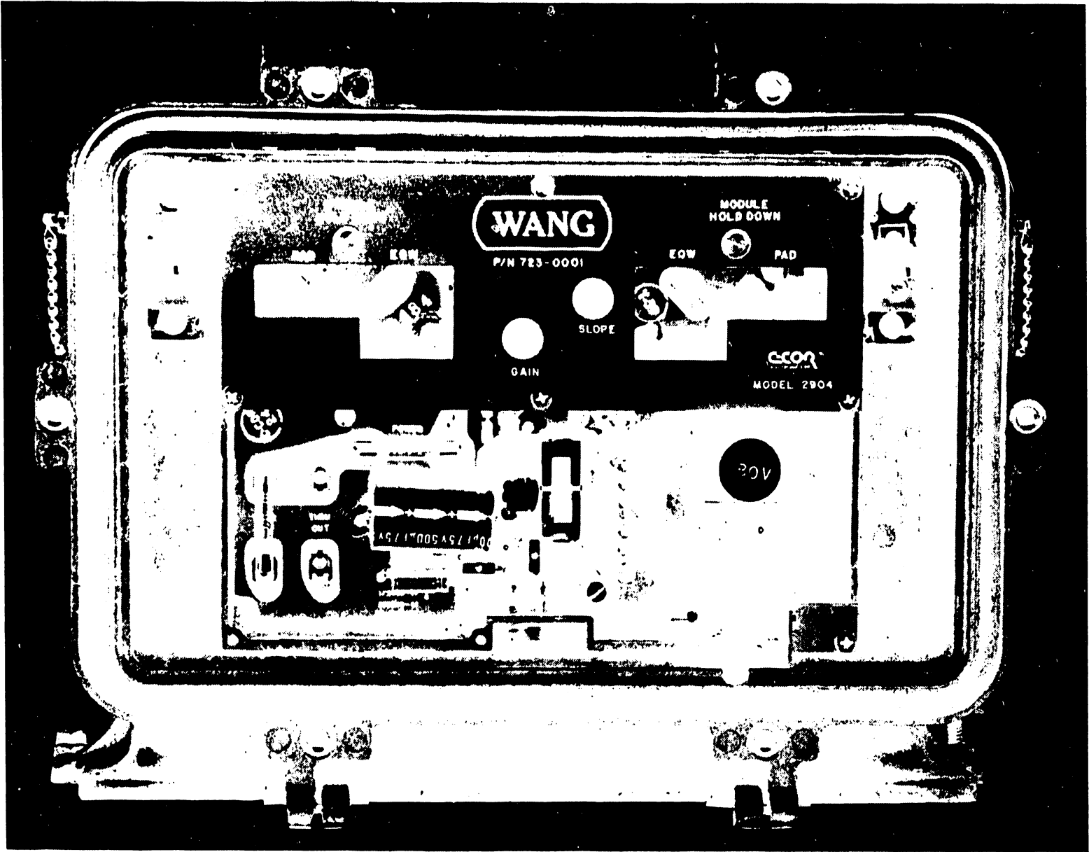
Figure 2-7 Amplifier Interior View
