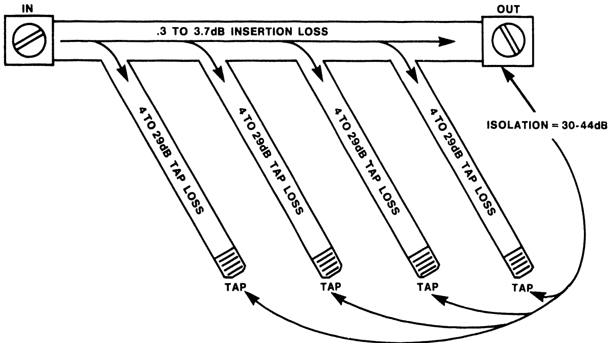
Figure 2-24 Directional Tap Functional Diagram
