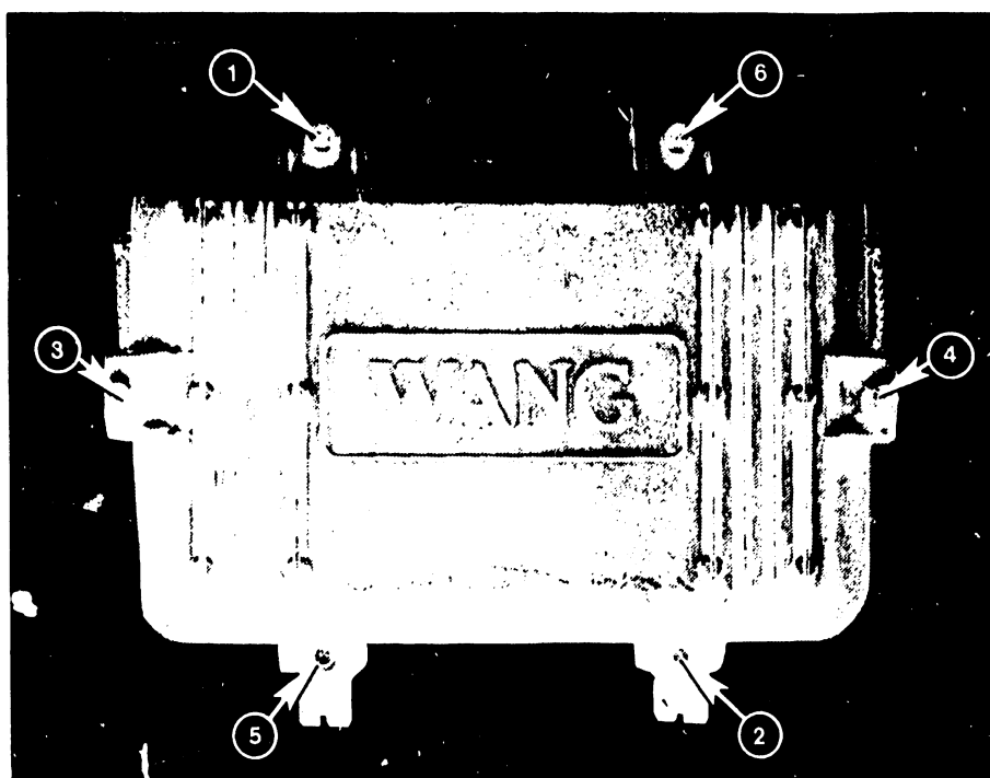
Figure 5-13 Cover Bolt Tightening Sequence
