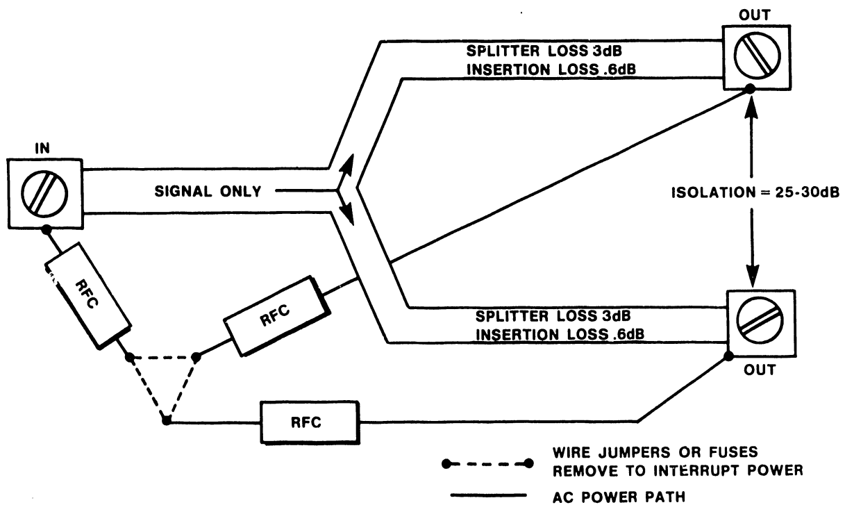
Figure 2-15 Splitter (Combiner) Application
