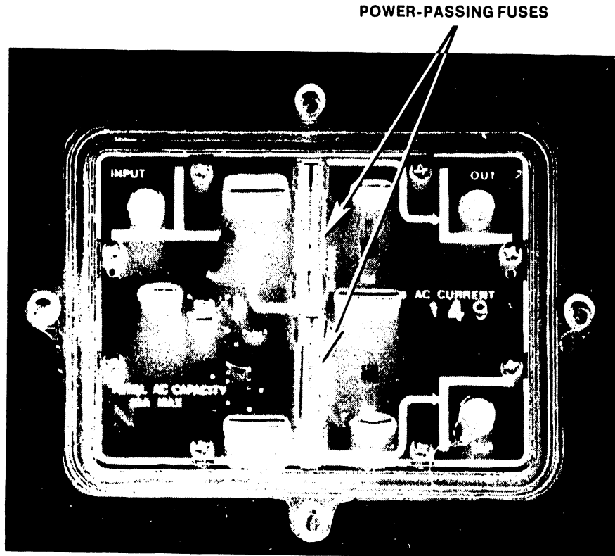
Figure 2-23 Typical Directional Coupler Interior View
