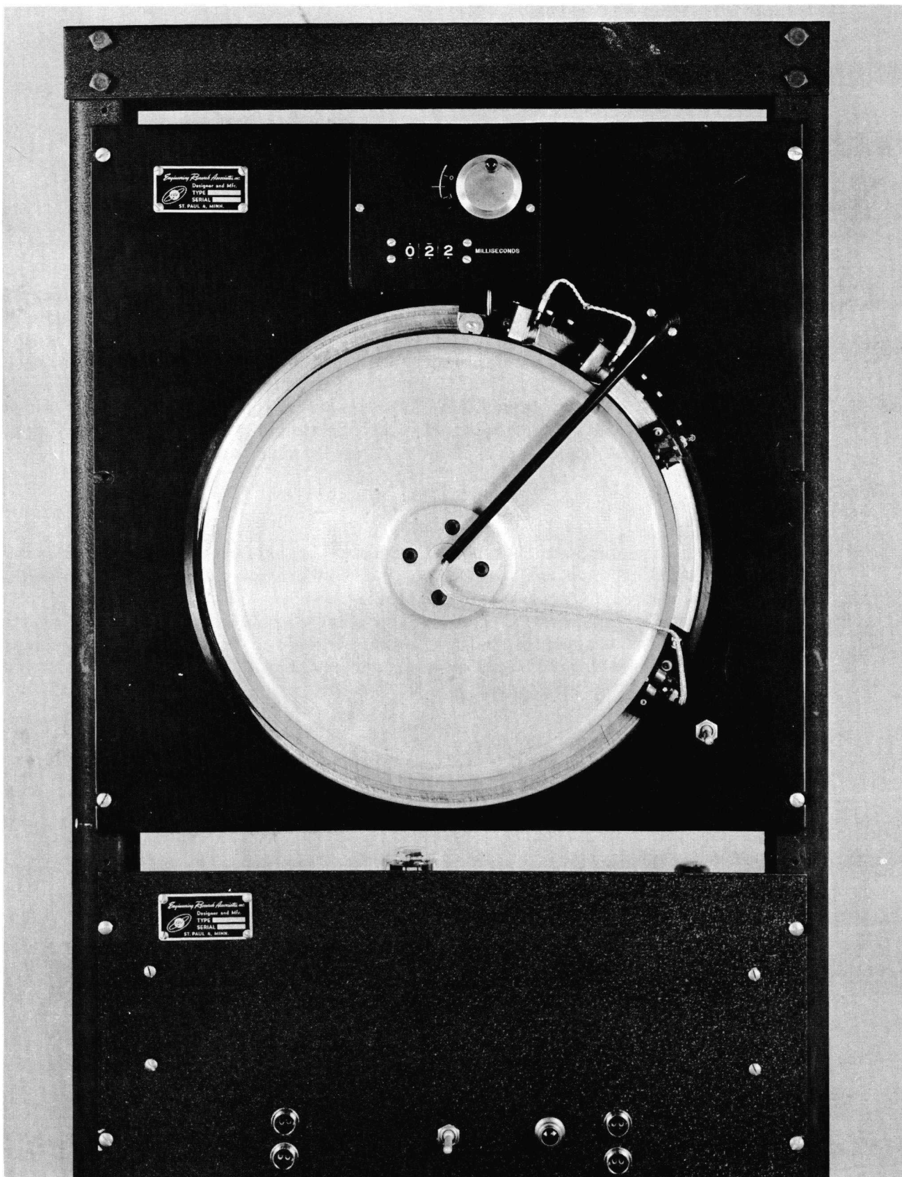
Boundary Displacement Delay Line
