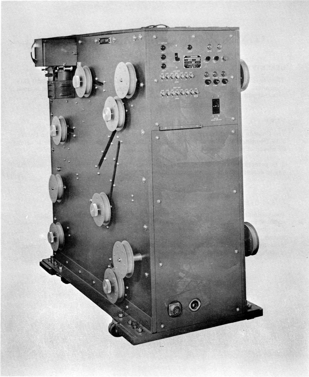
Dual Tape Reader
