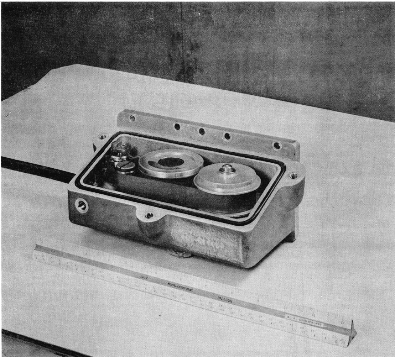
Self-Recording Accelerometer with Top Removed
