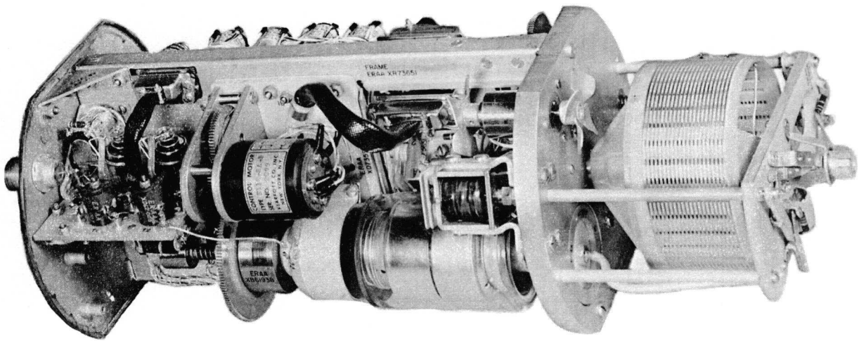
Automatic Antenna Coupler, Out of Container
