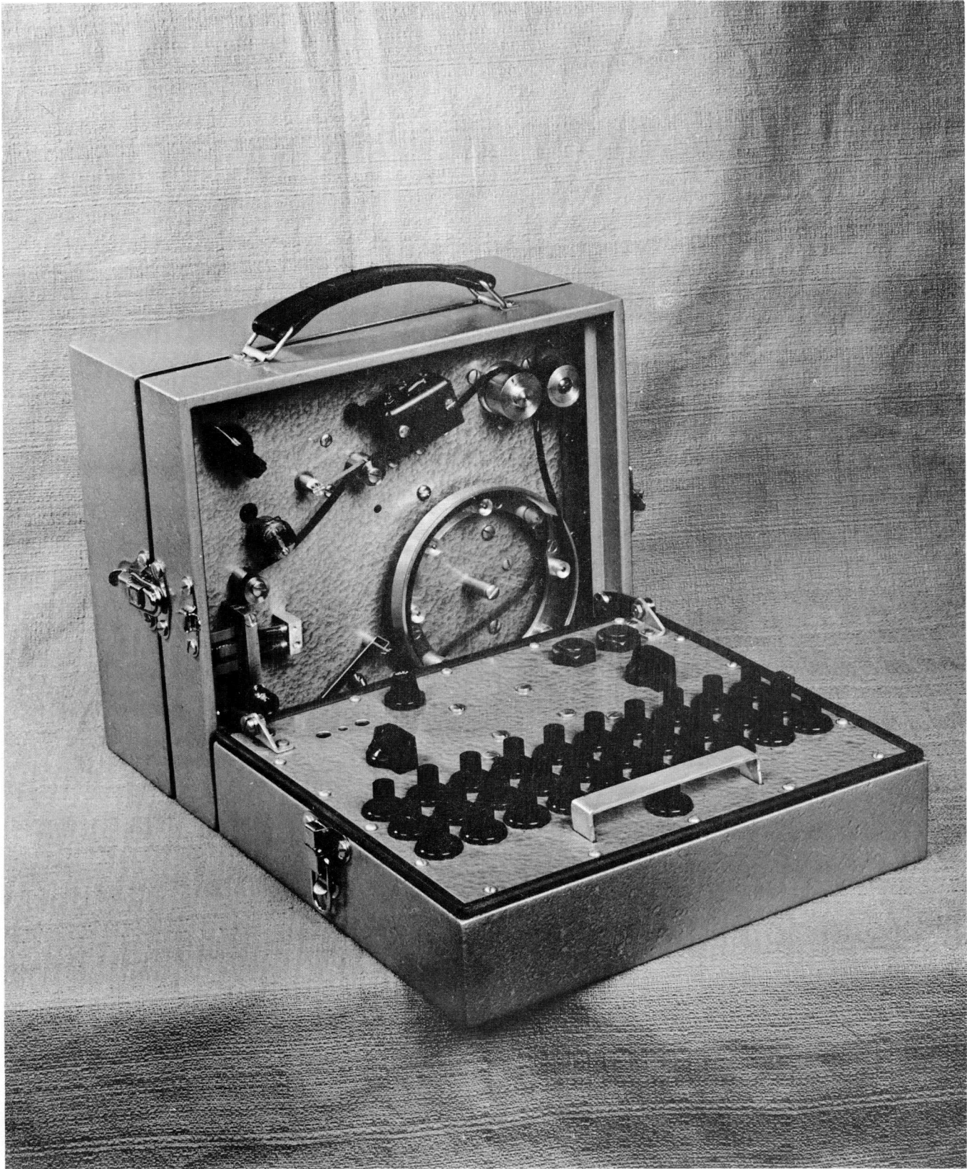
Portable Magnetic Tape Recorder
