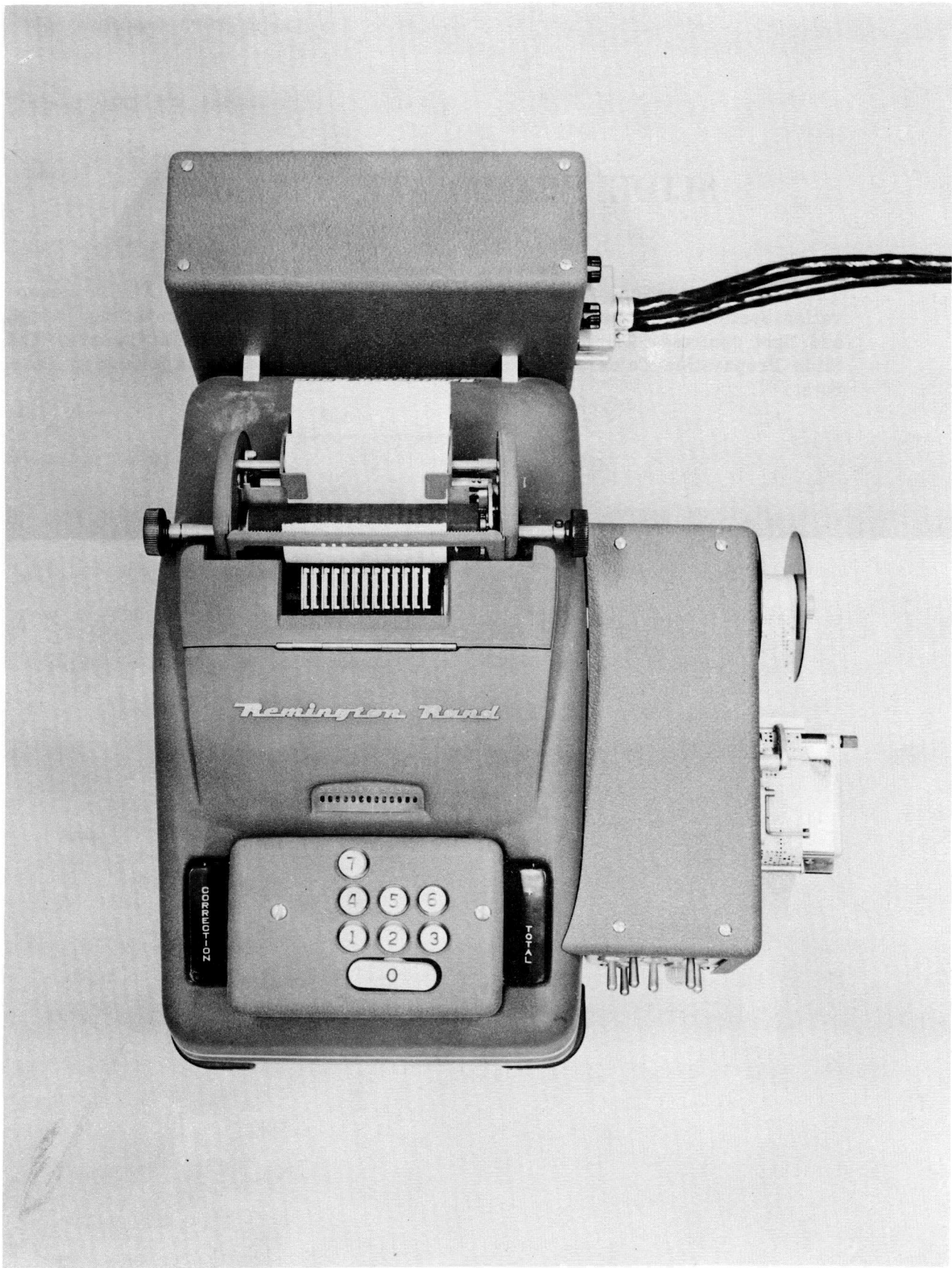
Tape Preparation Unit
