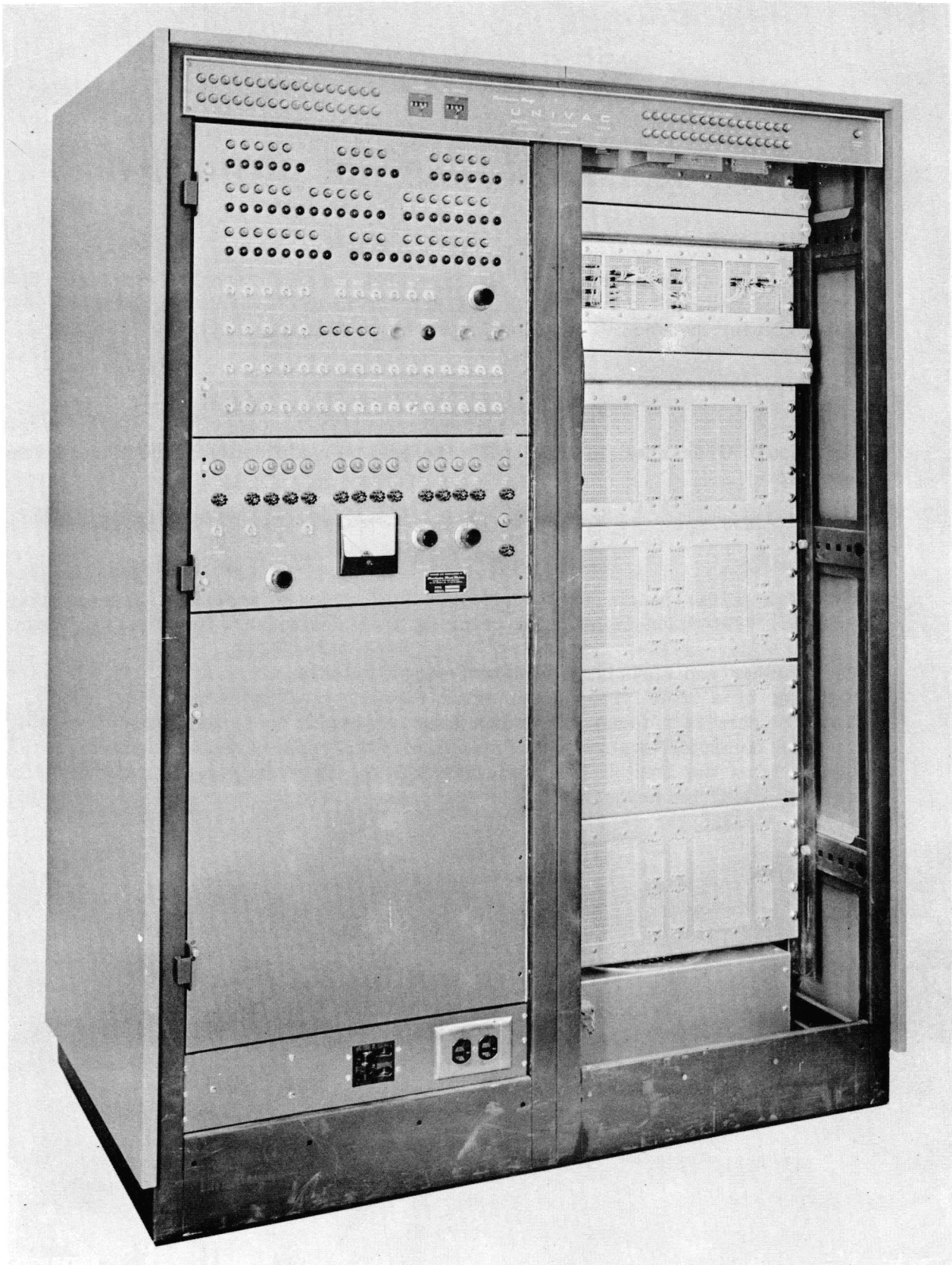
Programmer-Scanner Model H
