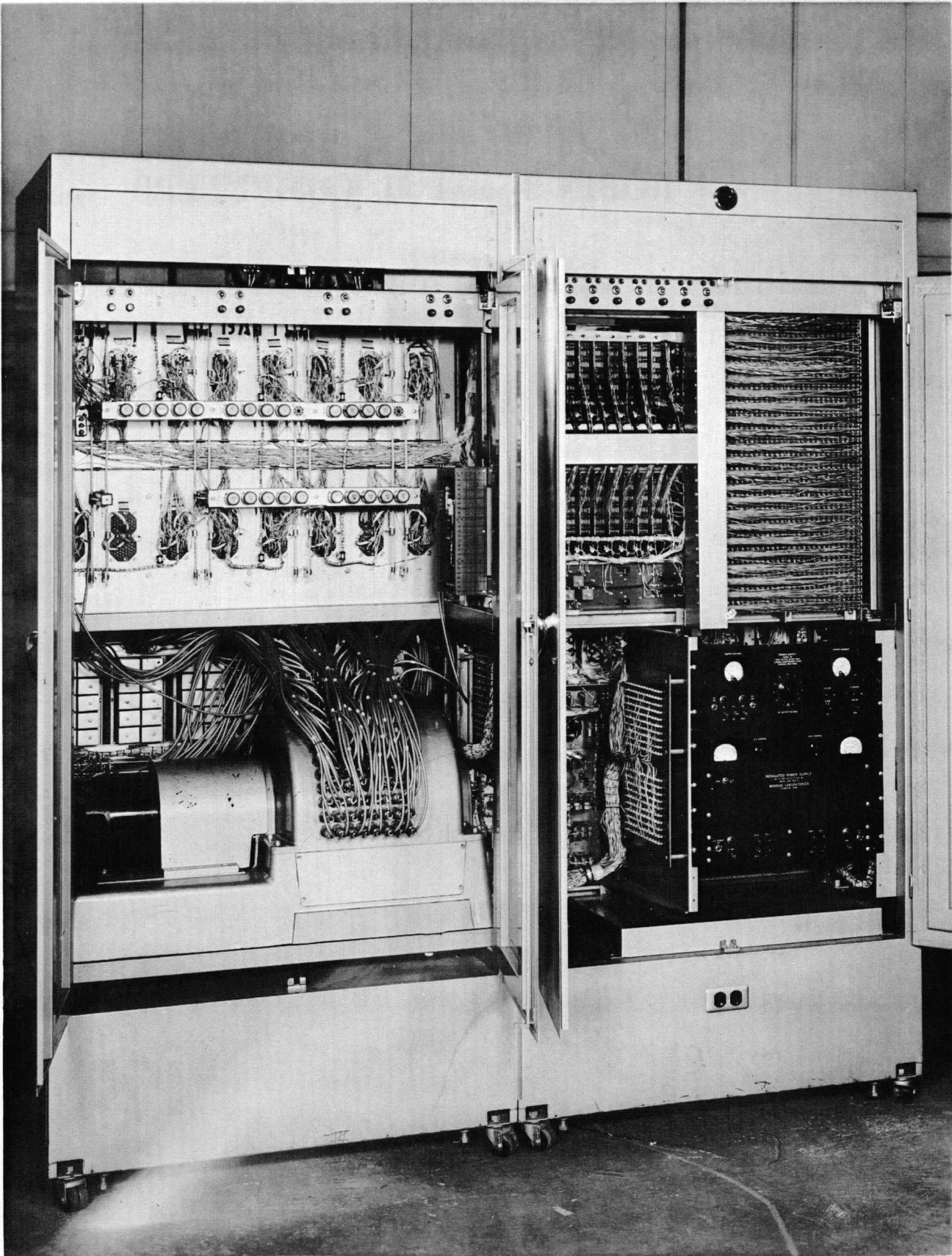
Speed Tally System - Memory Unit
