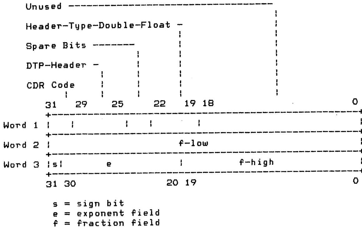
Figure 7-8 Double Precision Float Structure Format
