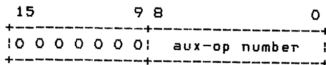
Figure 20-6 AUX-OP Instruction Format
