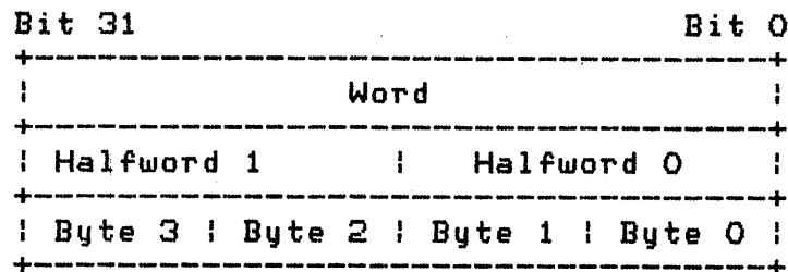
Figure 1-2 Layout of Words, Halfwords, and Bytes
