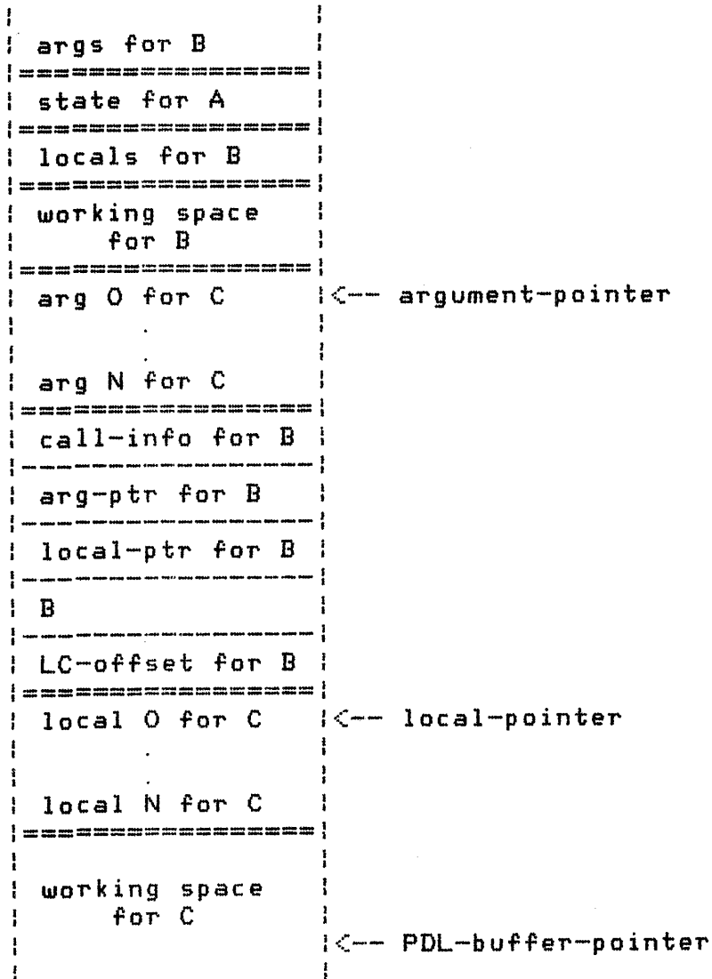
Figure 11-1 Call-Frame Layout
