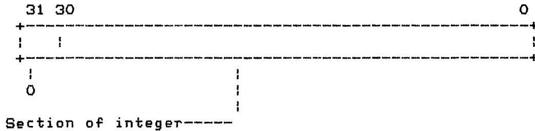
Figure 7-5 BIGNUM Data Format
