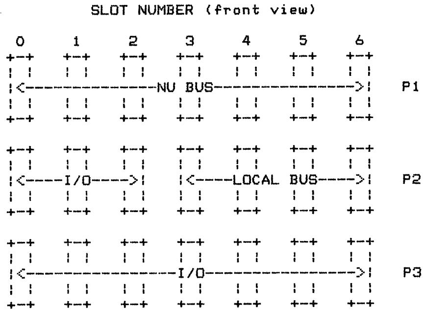
Figure 1-1 Backplane Configuration
