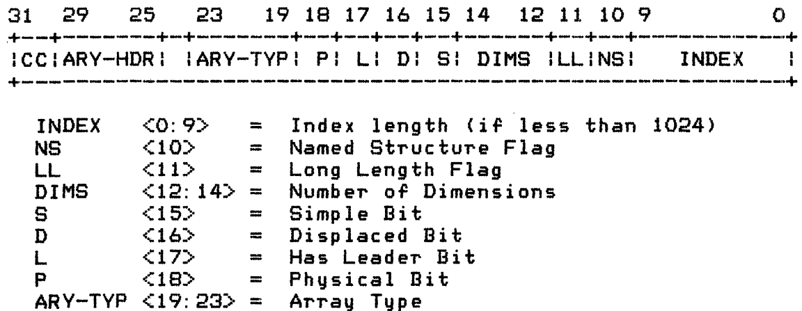
Figure 8-1 Array Header Word
