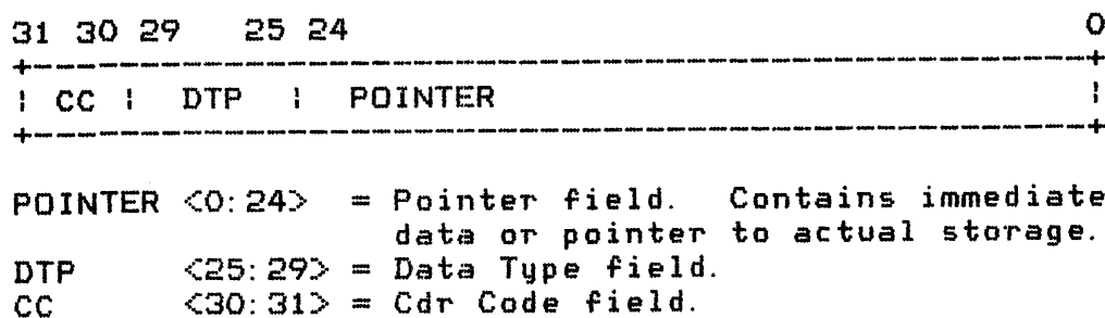
Figure 7-1 Q Format
