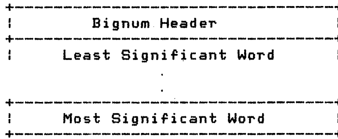
Figure 7-3 BIGNUM Structure
