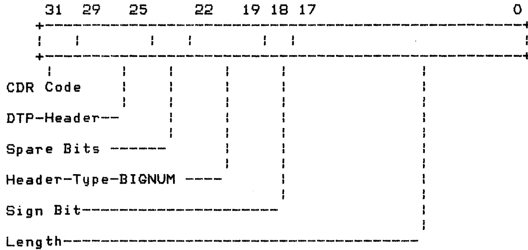
Figure 7-4 BIGNUM Header Format
