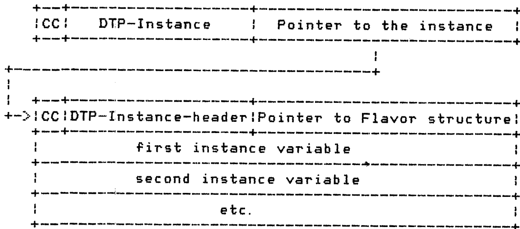
Figure 13-1 Flavor Instance
