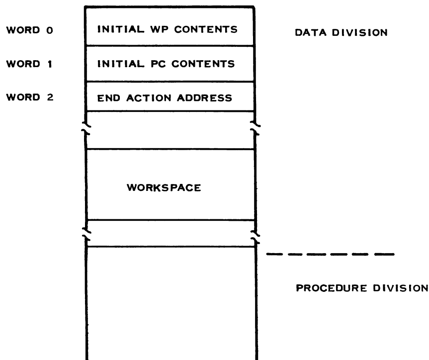
Figure 5-1. TX990 Task Structure
