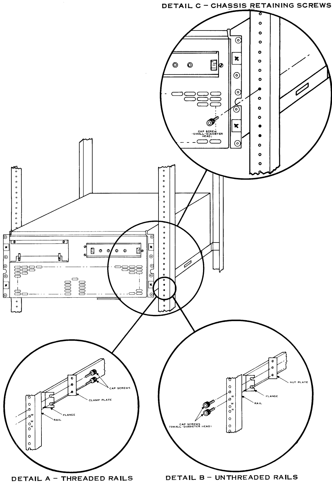
Figure 3-7. Perspective View of Slide Mounts
