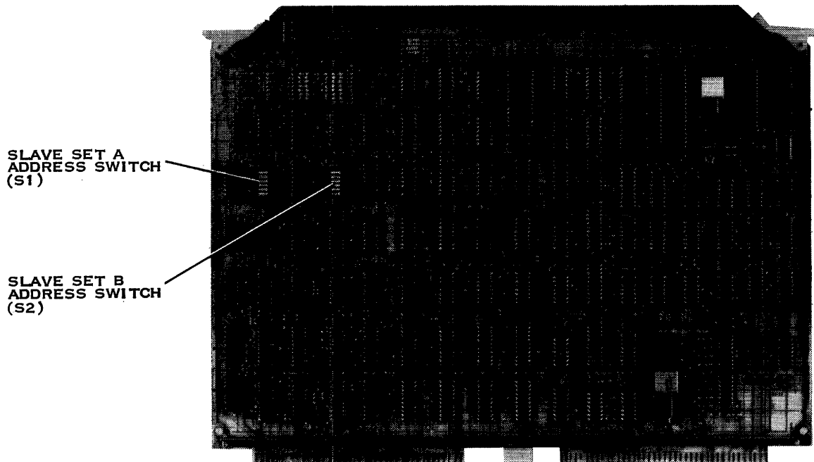
Figure 2-2. TPBI Board
