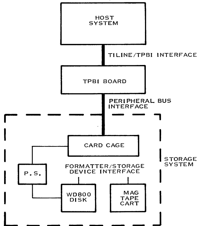
Figure 1-4. WD800 Functional Diagram
