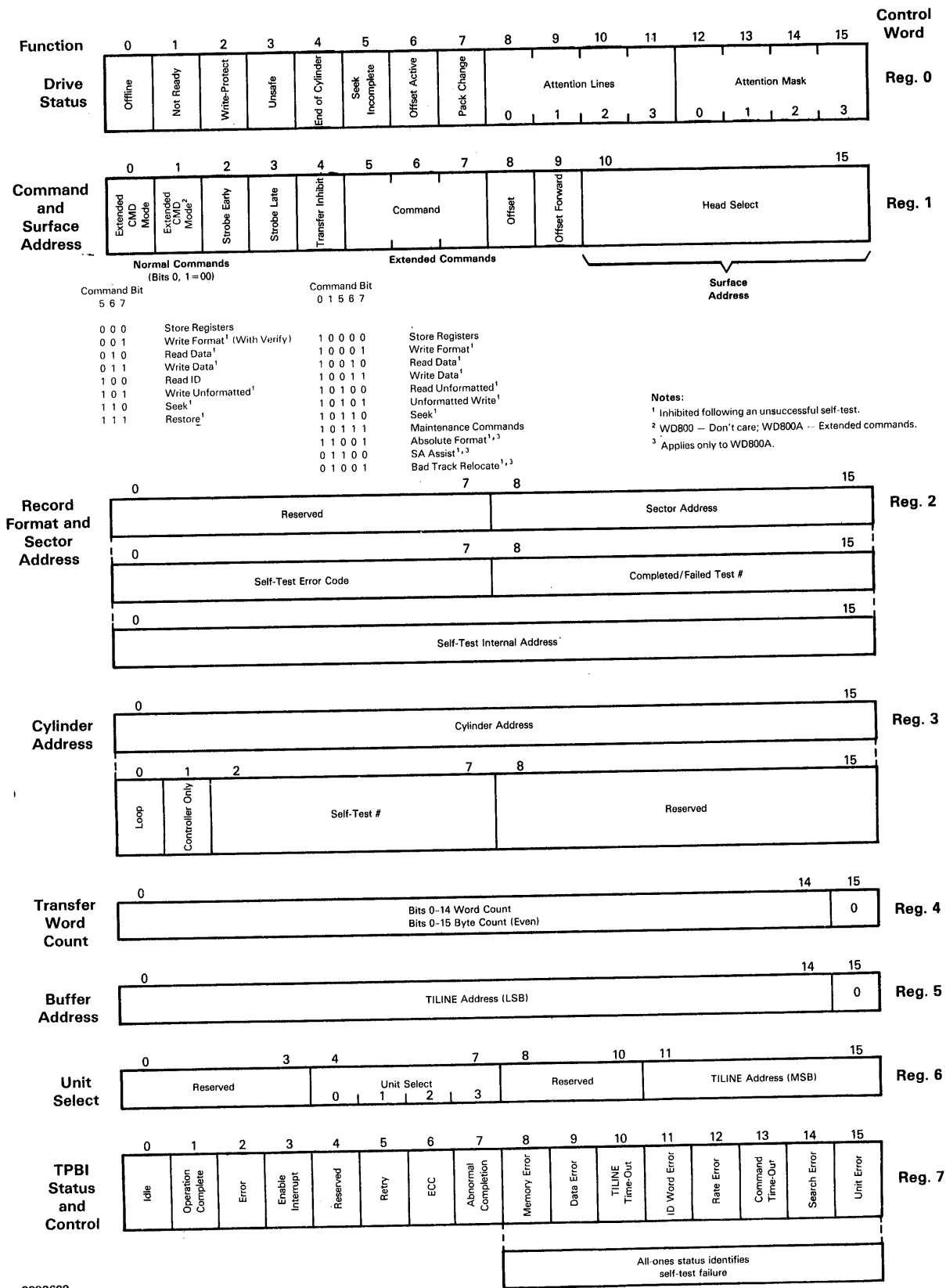
Figure 1-5. Disk Control and Status Block
