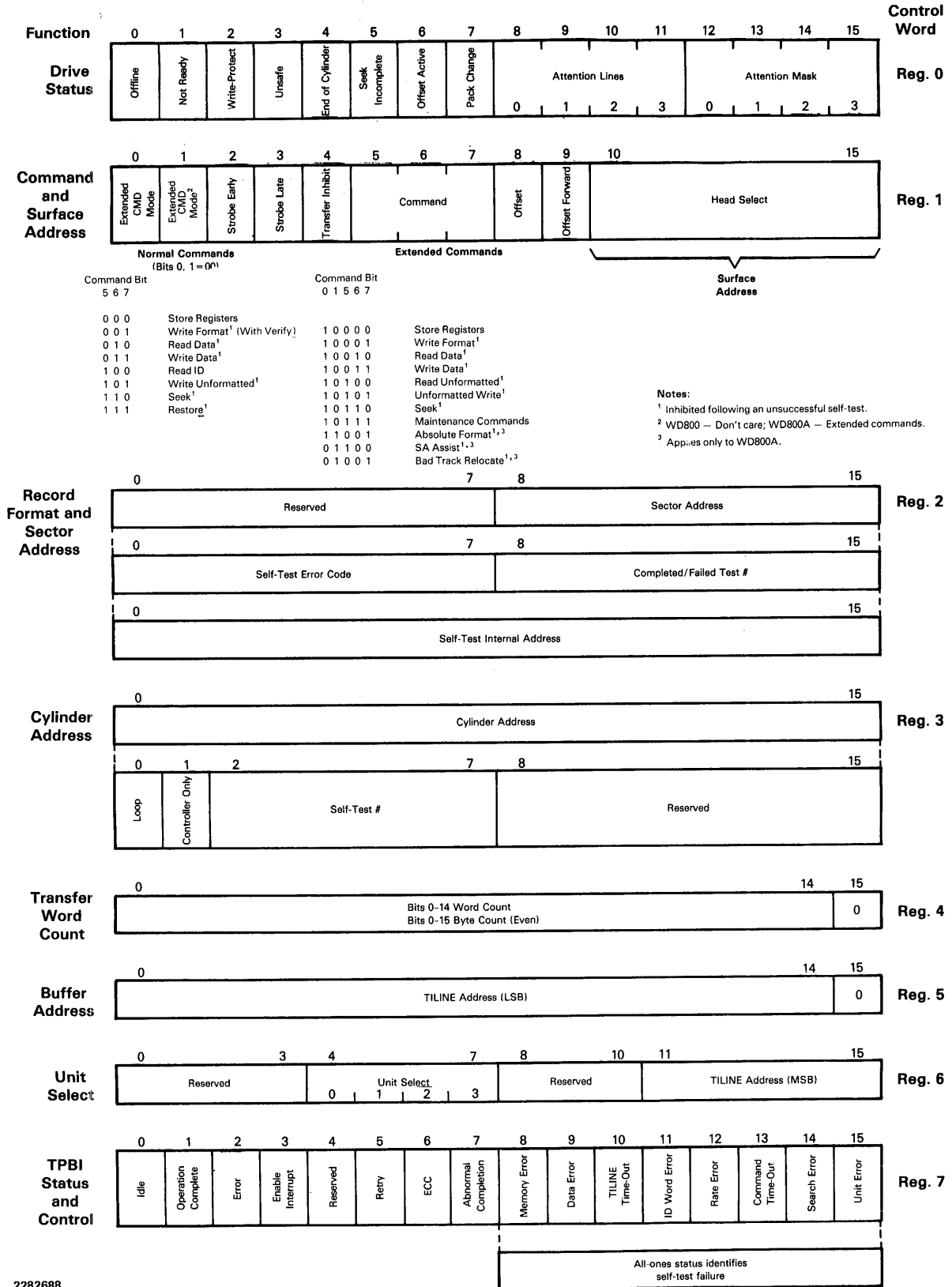
Figure 2-5. Disk Control and Status Word Formats
