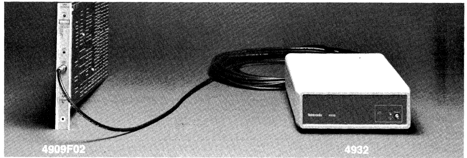
The 4909F02 GPIB Extender plugs directly into the Tektronix 4909 hard disk system bus and connects with a 4932 Extender through the coaxial "link" cable, extending GPIB data transmission over distances of 1650 feet to a 4050 System at the remote end.
