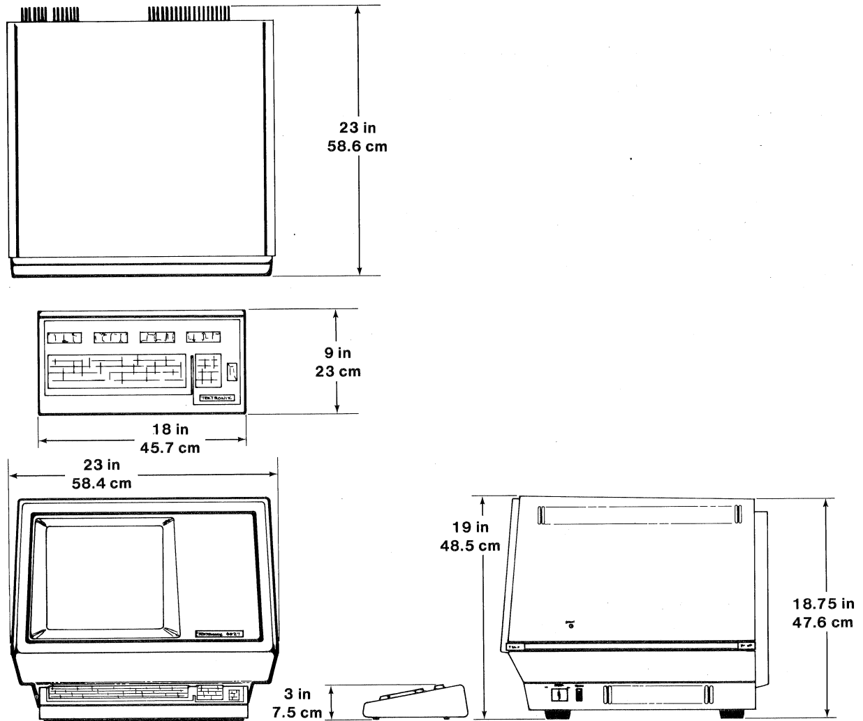
Figure 1-2. 4027 Dimensions.
