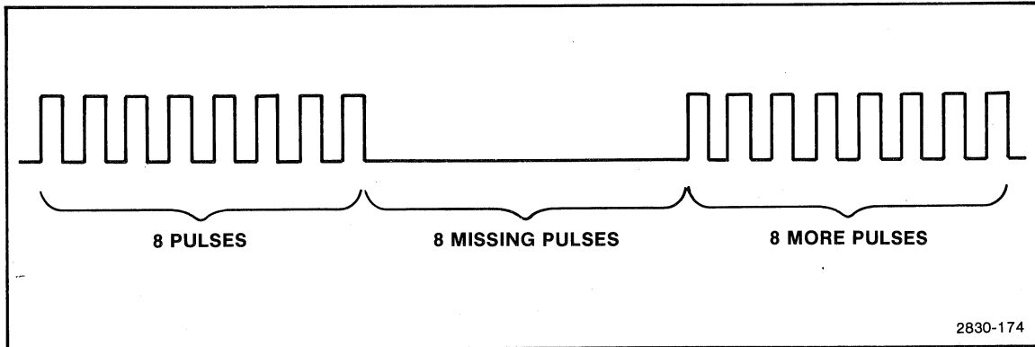
Figure 4-21. SCLK Waveform.
