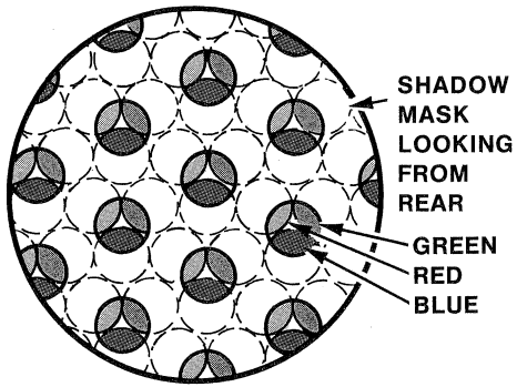
RELATIVE POSITION OF SHADOW MASK WITH RESPECT TO PHOSPHOR DOT TRIADS
