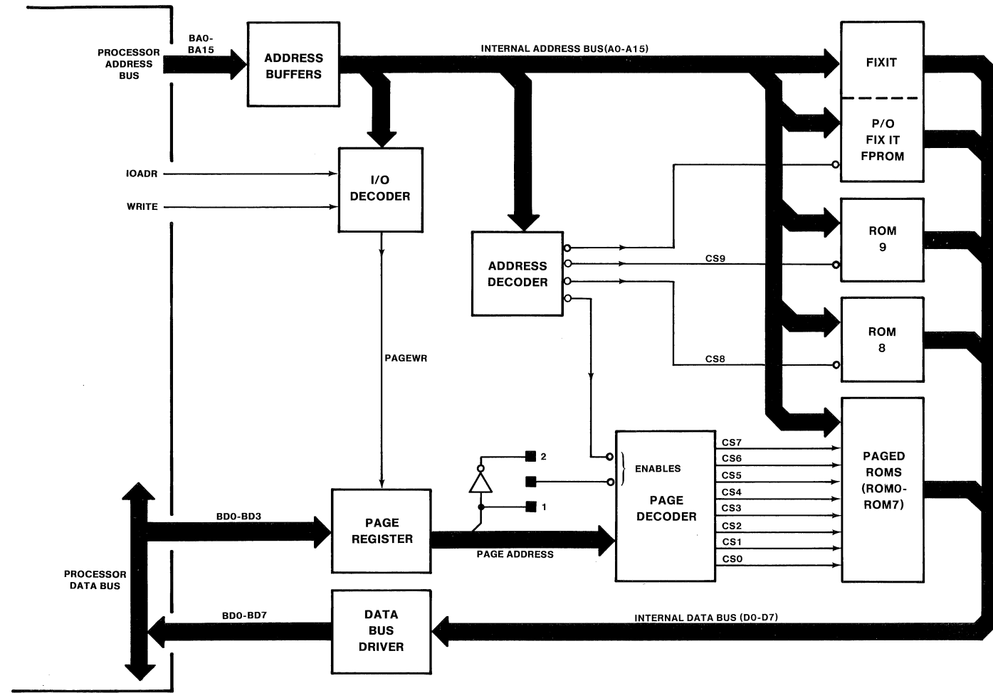
ROM EXPANSION BLOCK DIAGRAM
