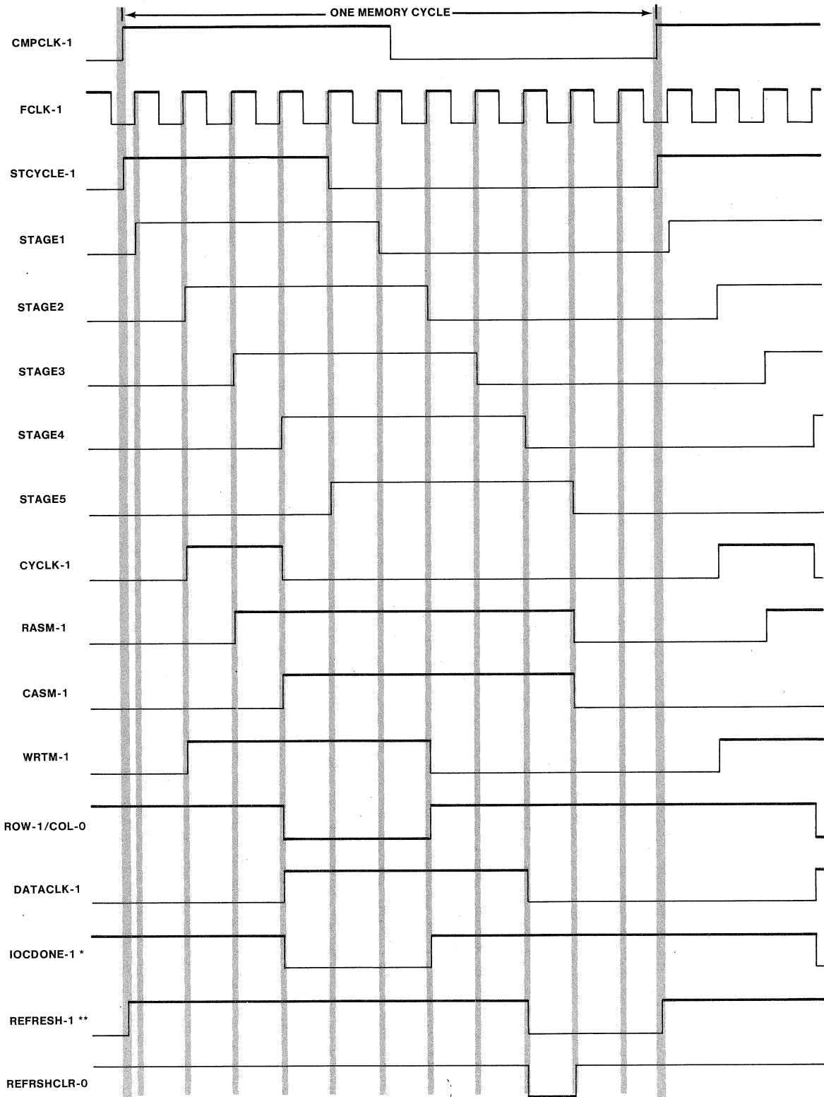
Figure 4-11. RAM Sequencer Waveforms.
