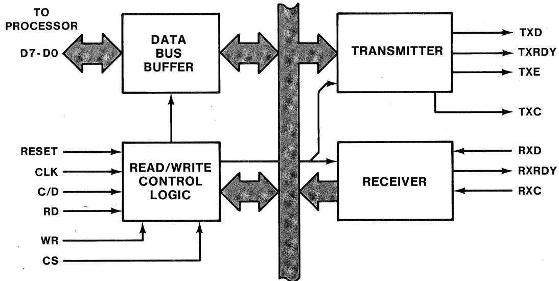
Figure 4-30. 8251 USART Functional Blocks.
