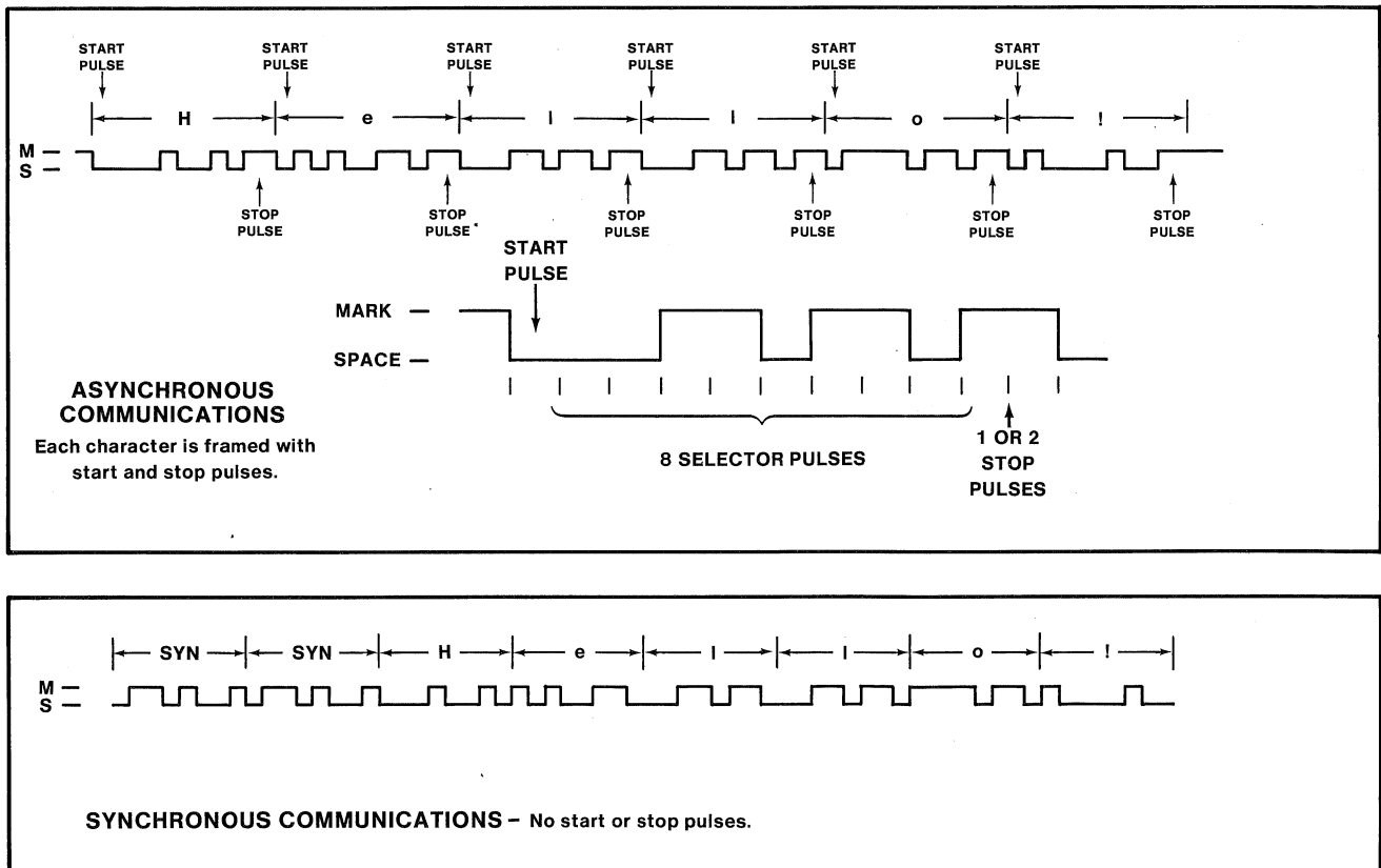
Figure 4-14. Asynchronous and Synchronous Serial Data Formats.
