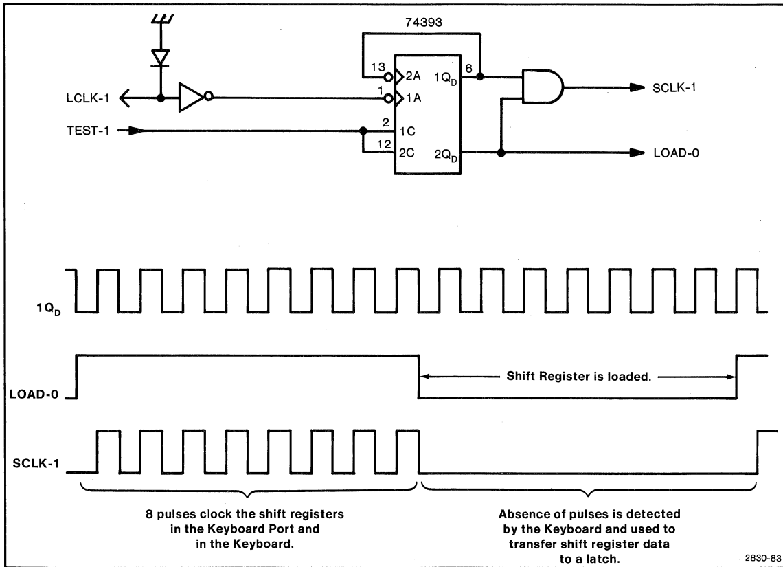
Figure 4-20. SCLK Generator and Waveforms.
