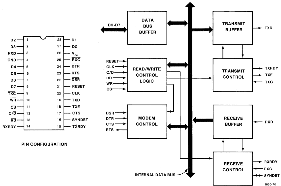
Figure 4-15. 8251A USART.
