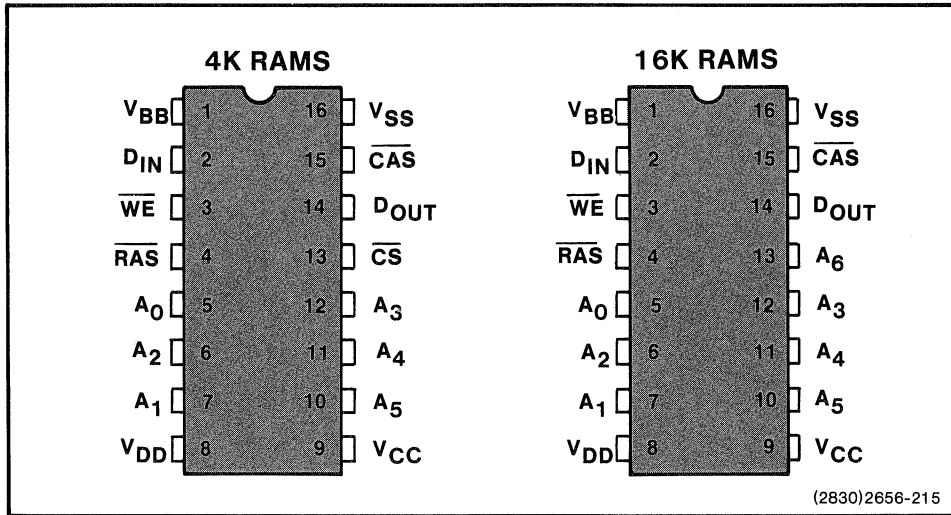
Figure 4-1. Pinouts for 4K and 16K RAMs.
