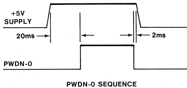
Figure 4-27. Power Up-Down Sequence.
