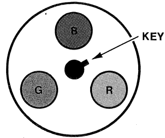
RELATIVE POSITION OF ELECTRON GUNS (LOOKING FROM REAR OF CRT).
