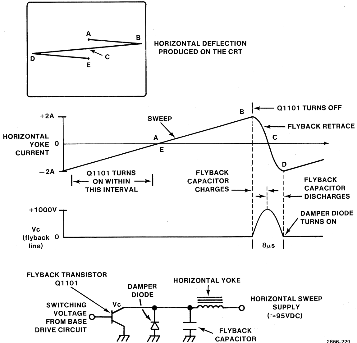
Figure 4-23. Horizontal Sweep.
