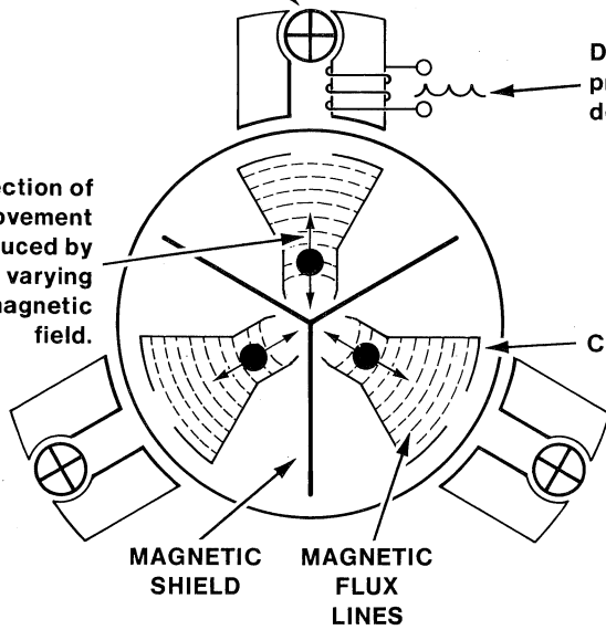
Figure 4-25. Convergence System
