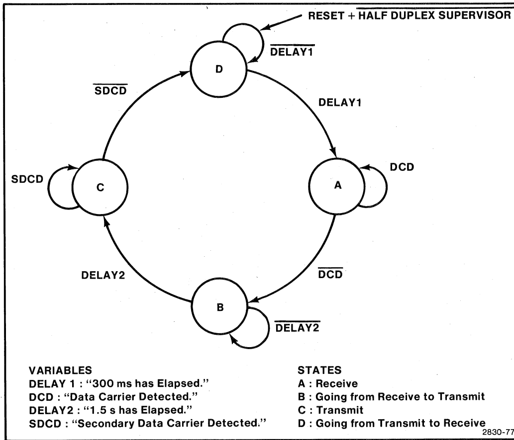
Figure 4-18. Line Turnaround State Diagram.
