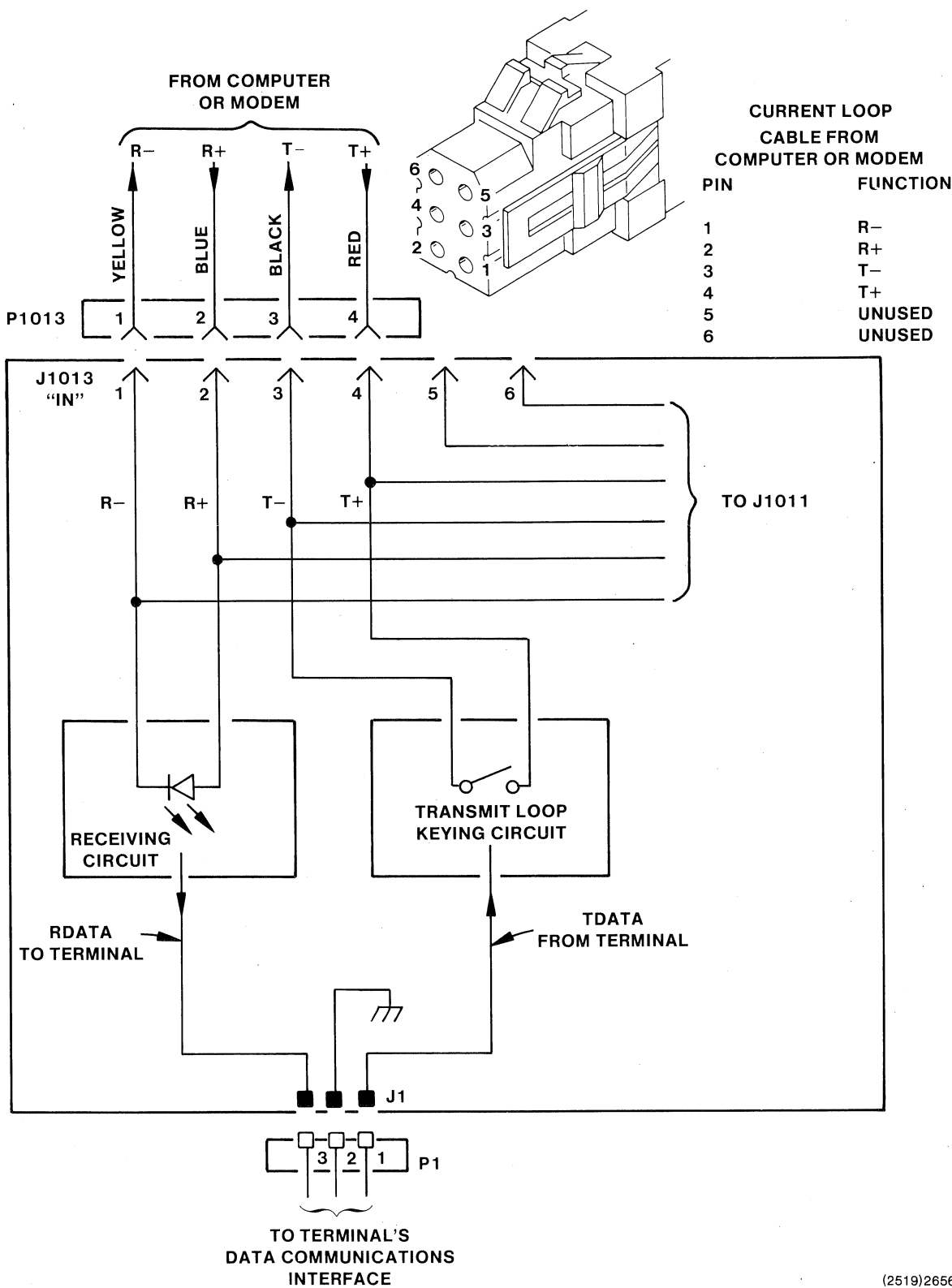
Figure 4-28. Option 2 in Passive Mode.
