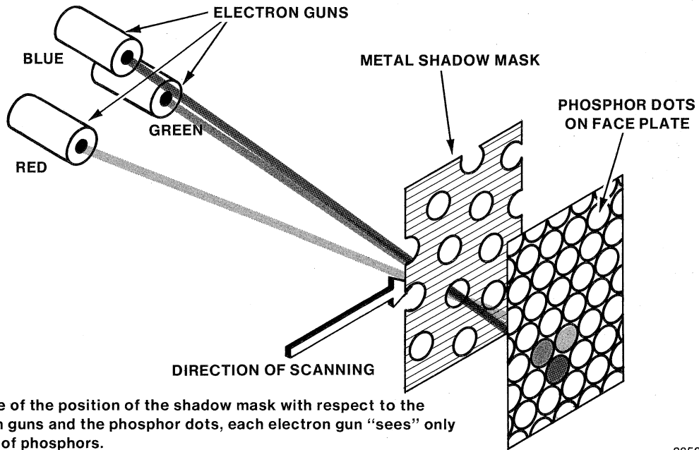
RELATIVE POSITION OF SHADOW MASK WITH RESPECT TO PHOSPHOR DOT TRIADS
