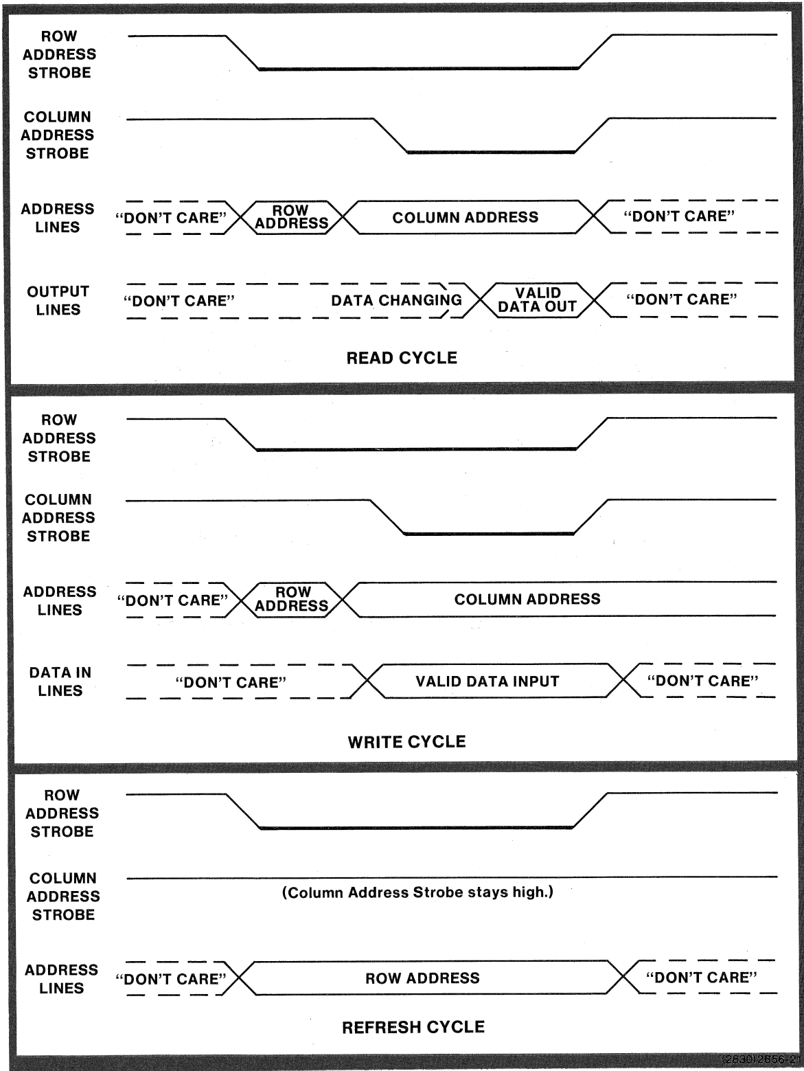
Figure 4-2. RAM Waveforms.
