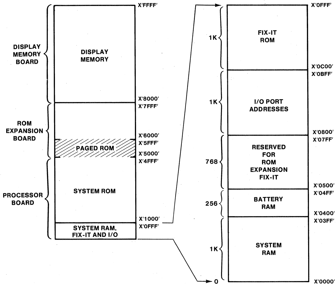
Figure 4-13. Microprocessor Address Space.
