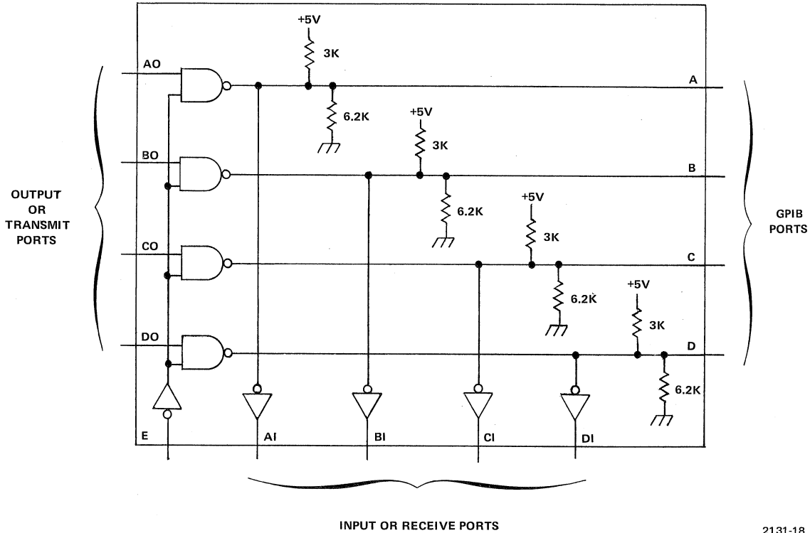
Figure 4-33. GPIB Transceiver.
