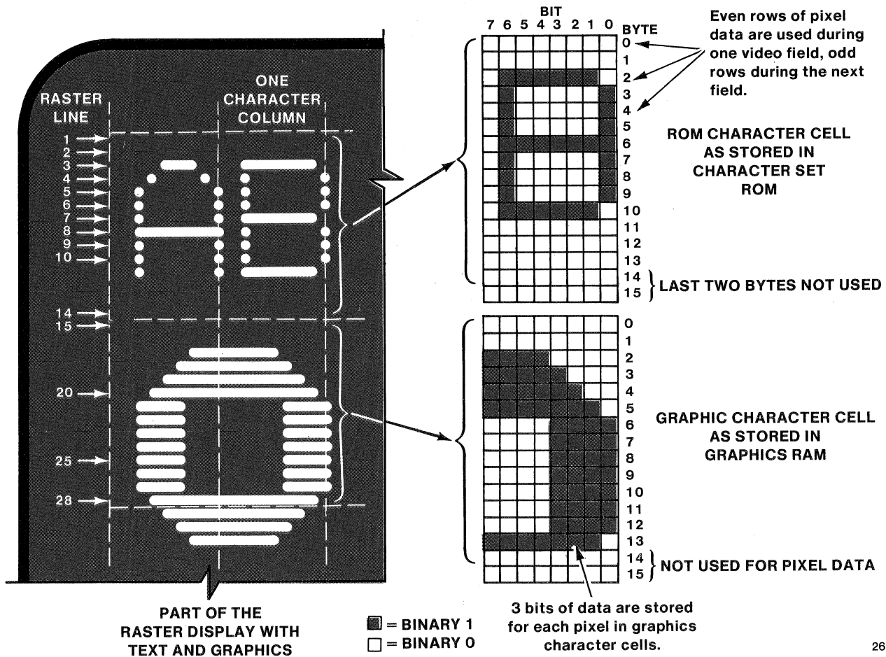
Figure 2-3. 4027 Character Cells.
