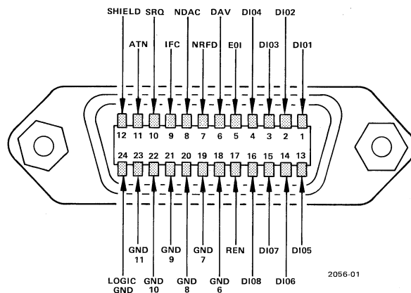
Figure 4-31. GPIB Connector.
