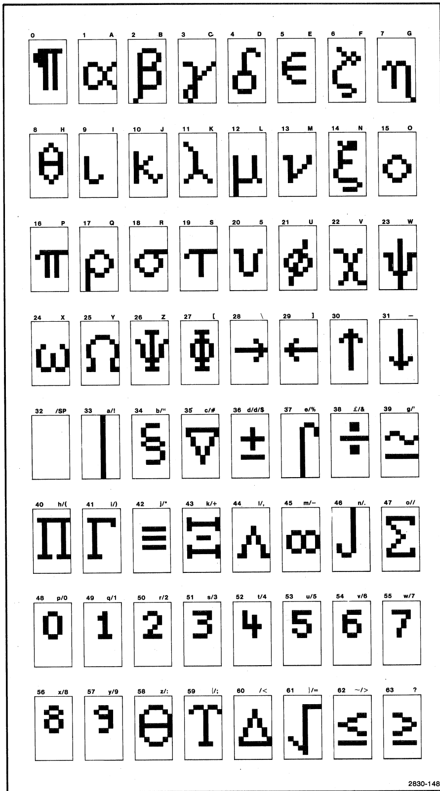
Figure 4-39. Math Characters.
