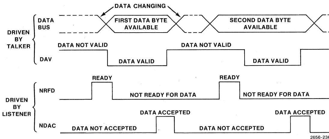
Figure 4-32. GPIB Transfer Bus Handshake Sequence.
