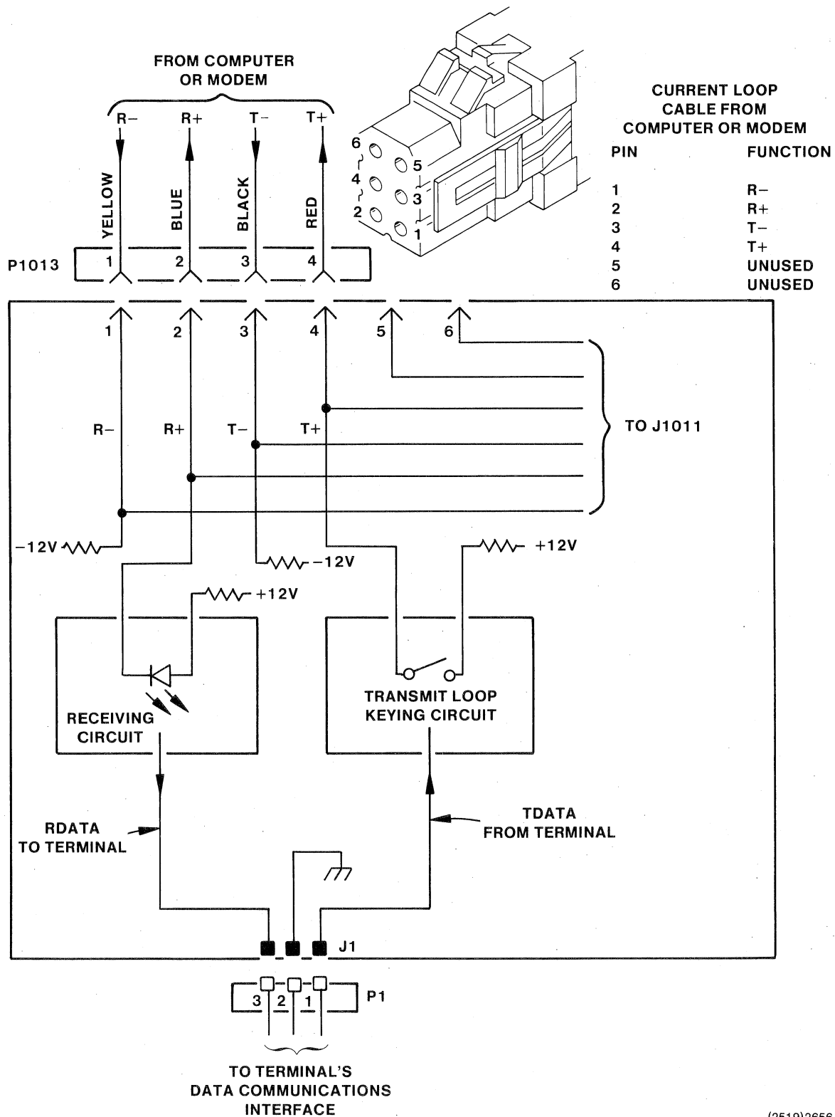
Figure 4-29. Option 2 in ACTIVE Mode.
