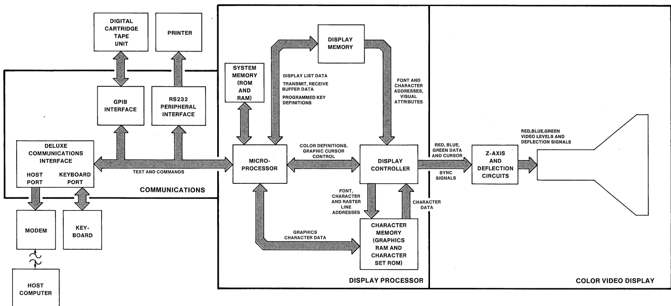
Figure 3-1. 4027 Functional Block Diagram.
