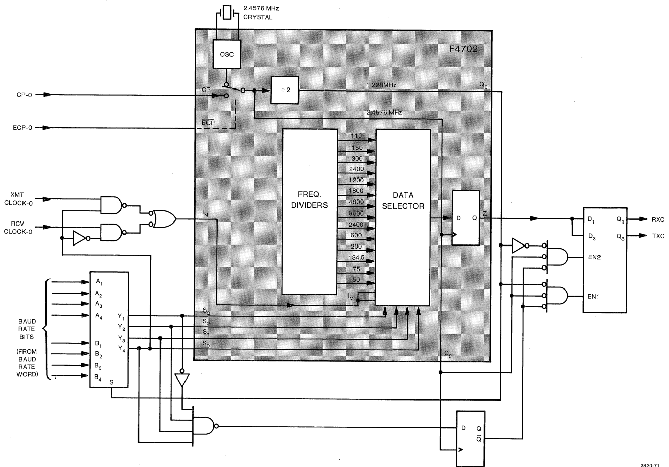
Figure 4-16. Baud Rate Generator.
