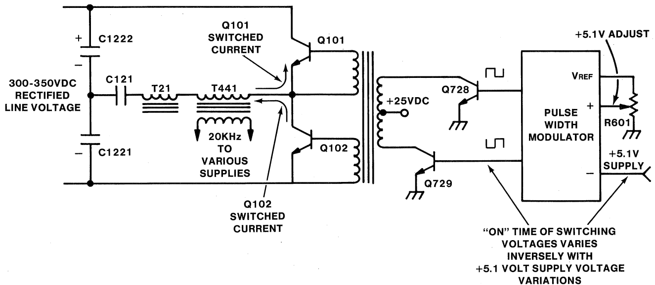
Figure 4-26. Low Voltage Power Supply Inverter, Simplified Schematic.
