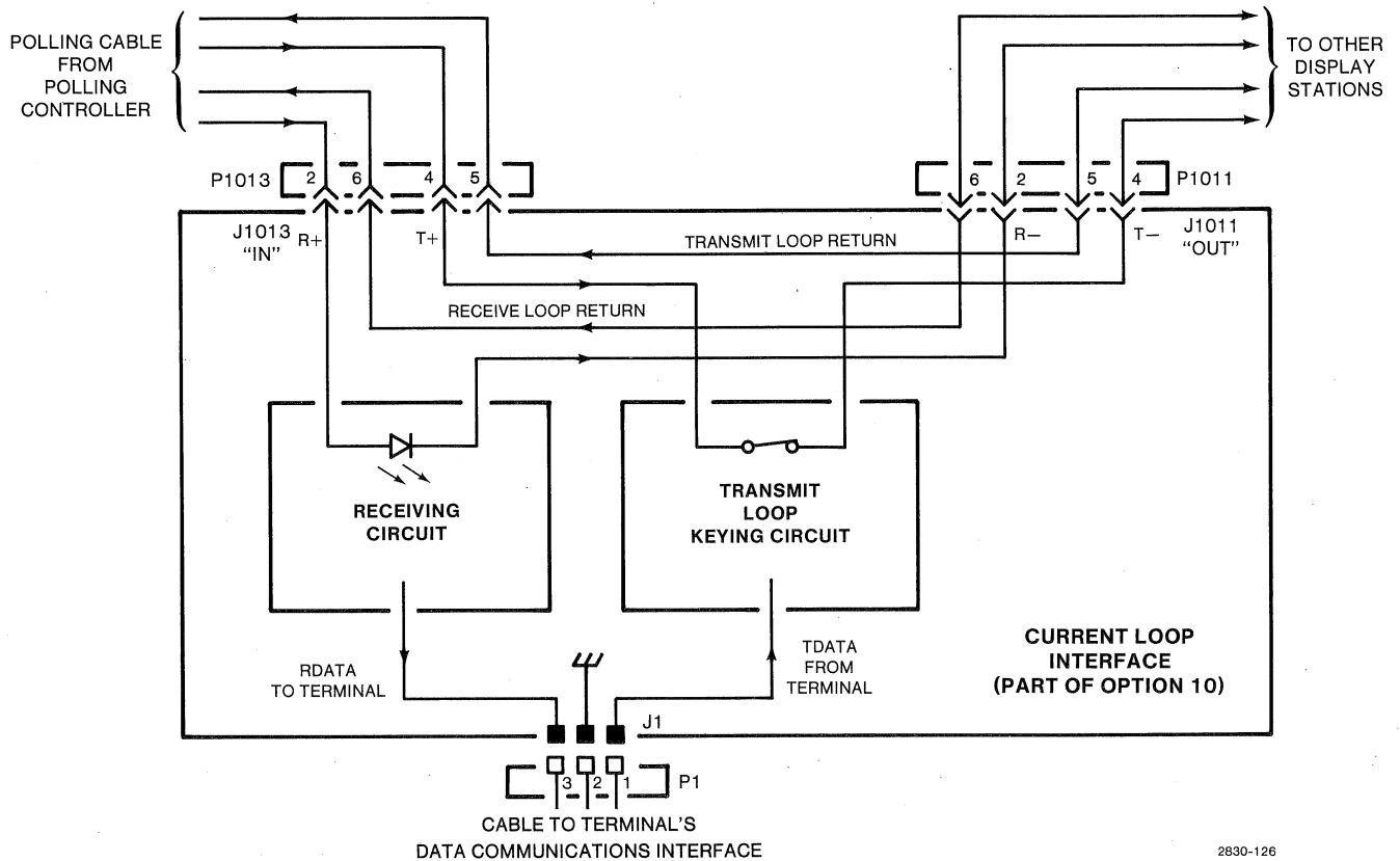
Figure 4-35. Current Loop Interface as used with Option 10.
