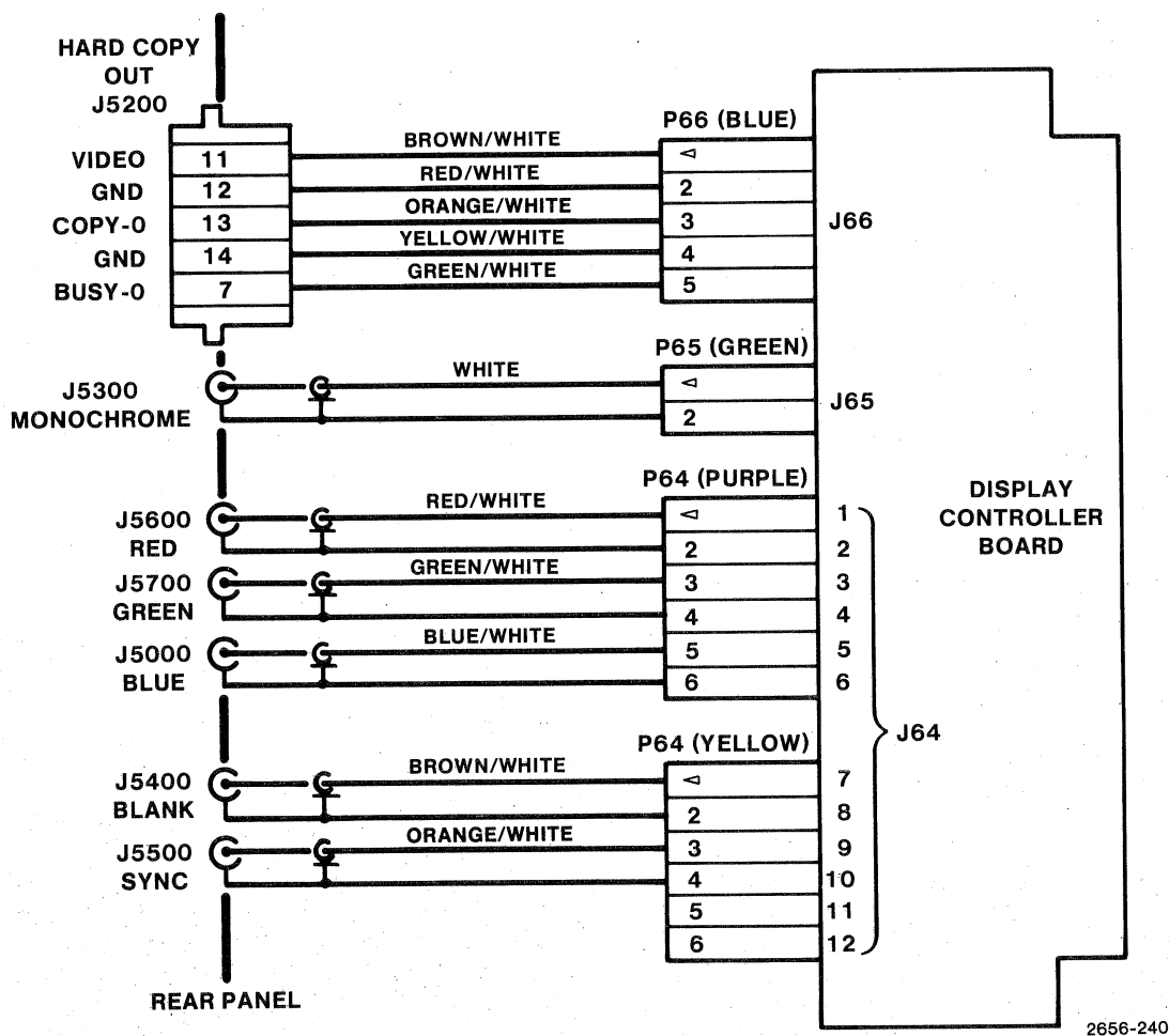
Figure 4-40. Option 42 Connectors.
