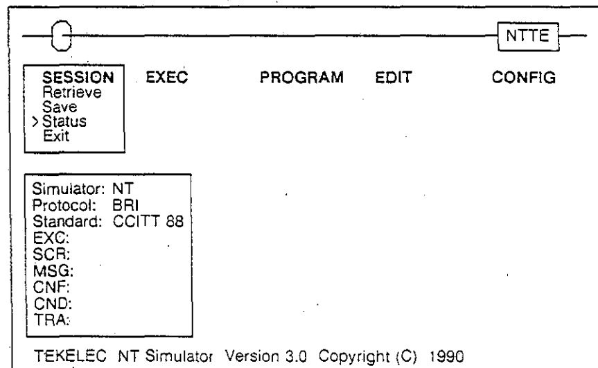
Figure 1.2: The User Interface
