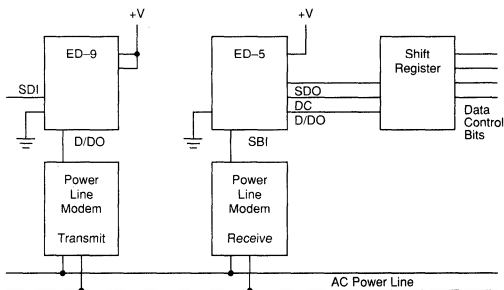
Figure 1. System Diagram
