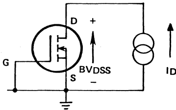
Figure 6. N-Channel BV_{DSS} Measurement
