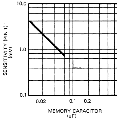
Detector Sensitivity vs CMEM
