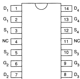
top view 14-pin DIP
