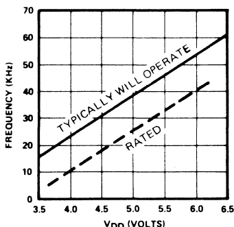
OPERATING vs V_{DD}
