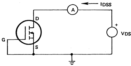
Figure 5. N-Channel I_{DSS} Measurement
