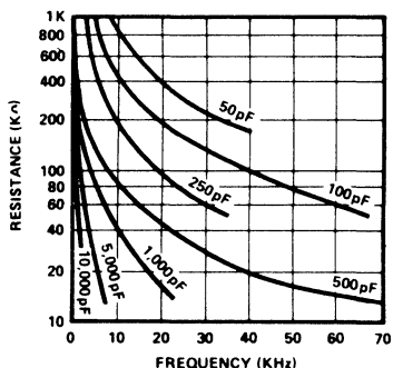
RESISTANCE vs OSCILLATOR FREQUENCY
