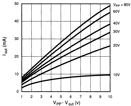
Typical HV04H/06H Source Current @ 25°C
