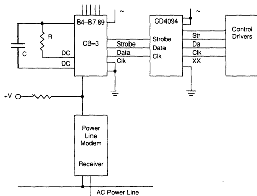
Figure 4. Receive Circuit
