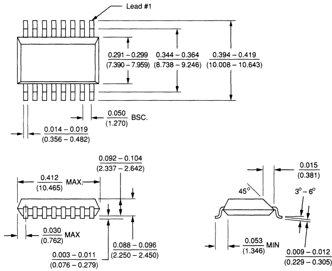
16 Lead Small Outline, Wide (WG)
