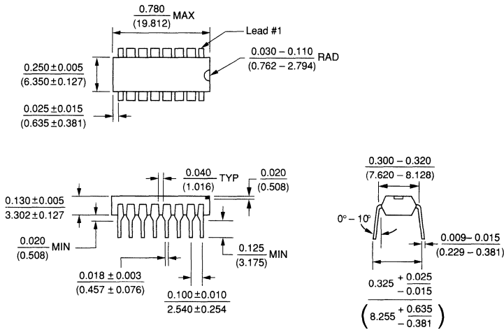
16 Lead Plastic DIP (P)
