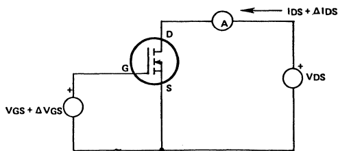
Figure 7. N-Channel G_{fs} Measurement
