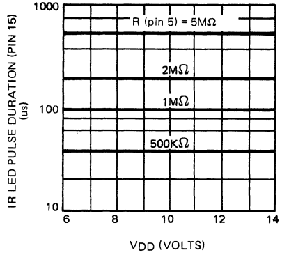
TPD vs VDD
