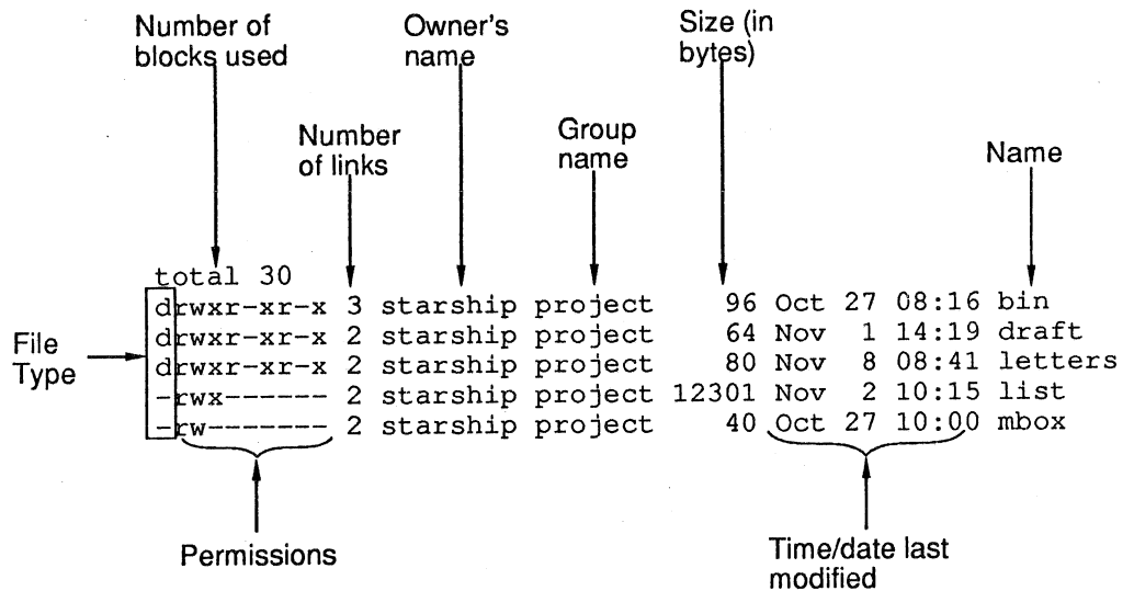
Figure 3-5. Output of the ls -l command
