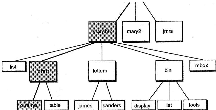
Figure 3-4. Relative Path from starship to outline
