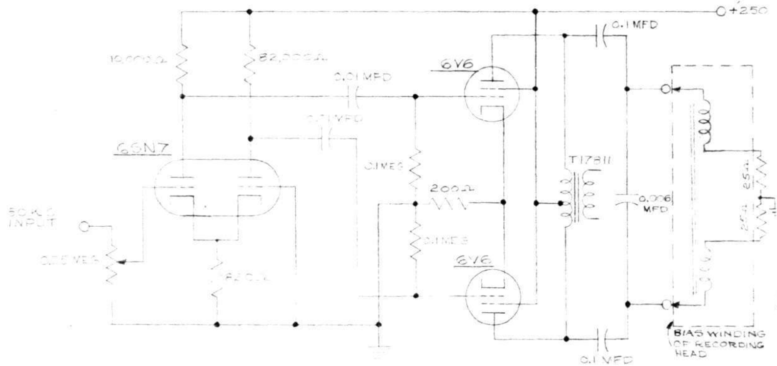
FIG. 14. CIRCUIT DIAGRAM OF BIAS AMPLIFIER.
