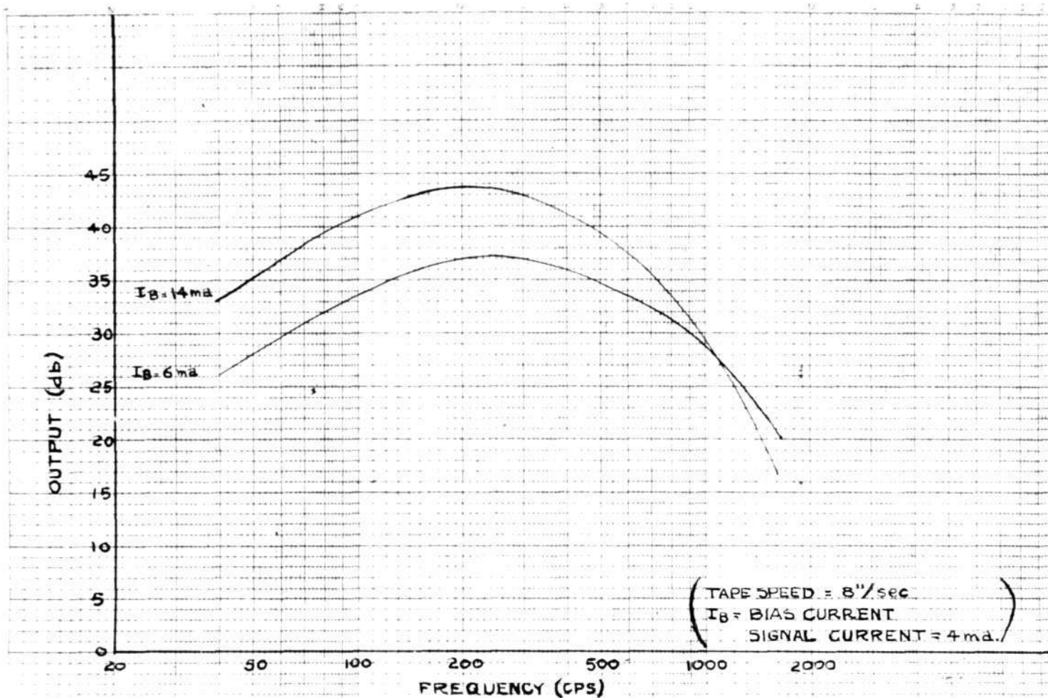
FIG.20. FREQUENCY RESPONSE OF "STEEL" TAPE FOR TWO VALUES OF BIAS CURRENT
