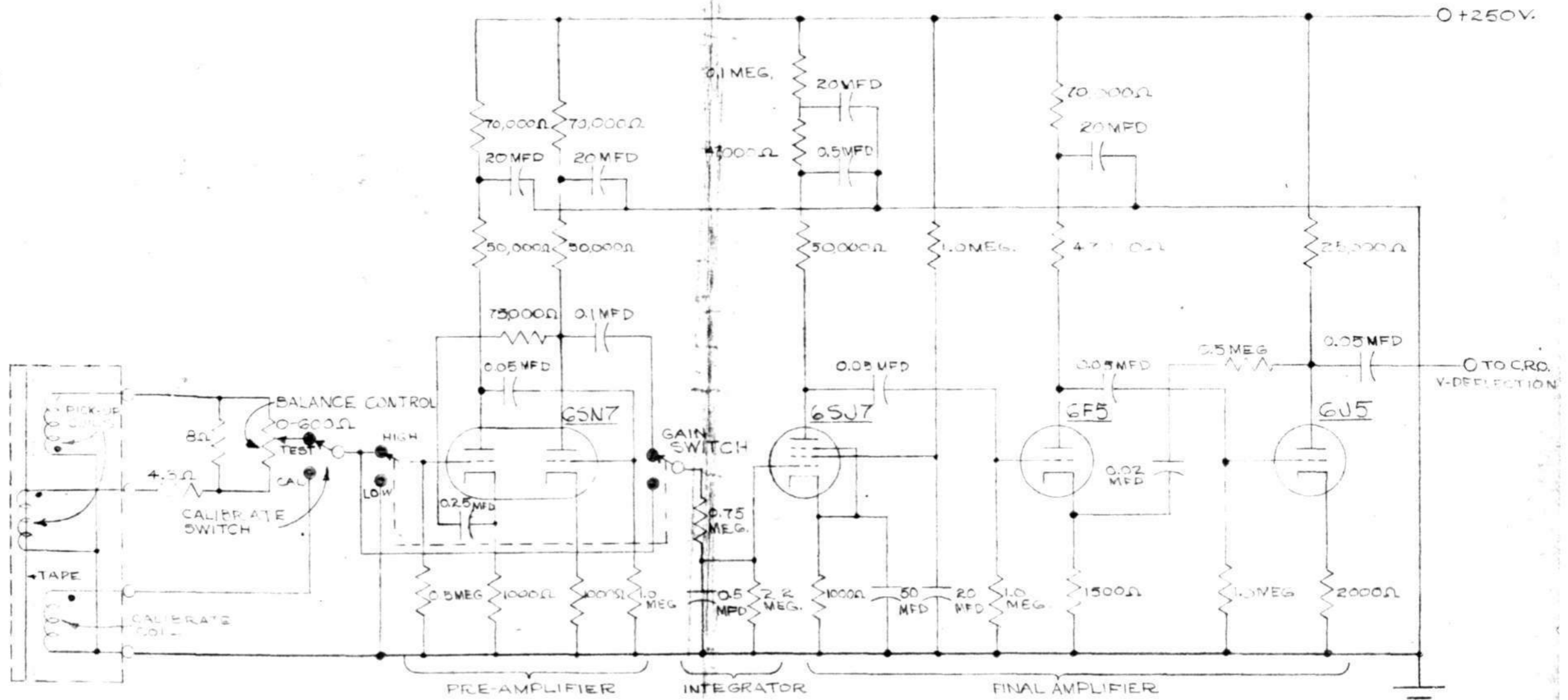
FIG. 26. B-AMPLIFIER FOR B-H CURVE TRACER
