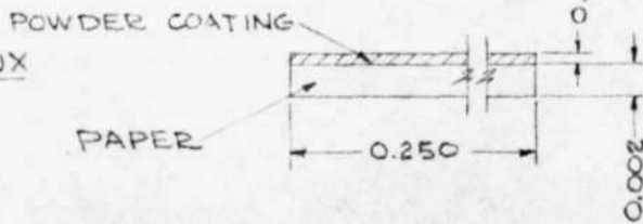
FIG. 17 CROSS-SECTIONS OF TAPES FOR MAGNETIC RECORDING
