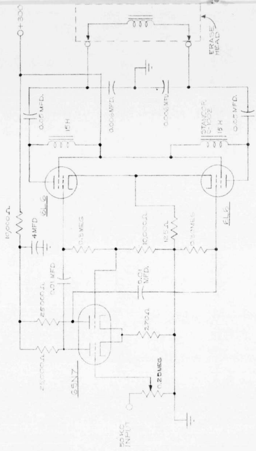
FIG. 13. CIRCUIT DIAGRAM OF ERASING AMPLIFIER.
