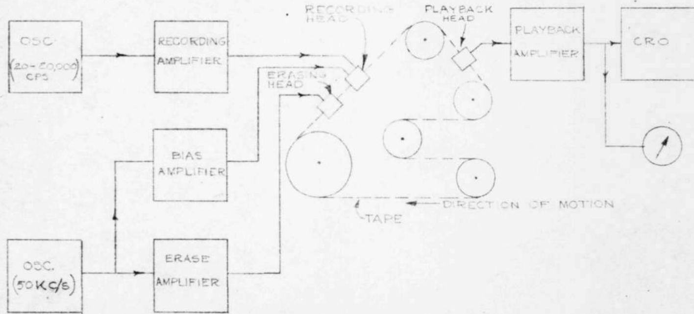
FIG. 11. SCHEMATIC DIAGRAM OF COMPLETE EXPERIMENTAL MAGNETIC RECORDING SYSTEM.
