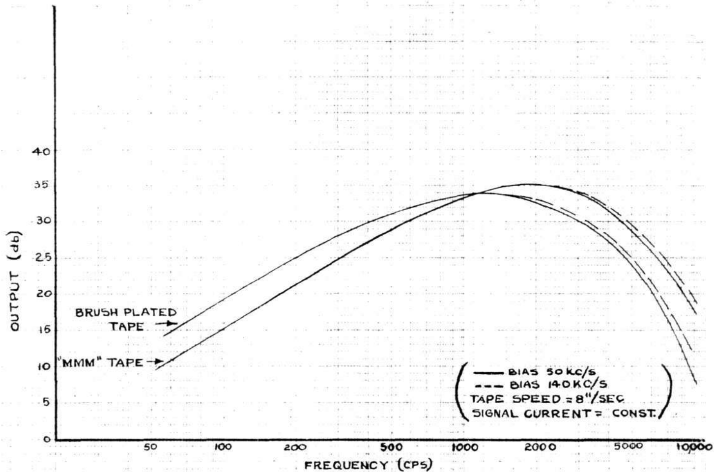
FIG. 22. VARIATION OF FREQUENCY RESPONSE OF RECORDING MEDIA WITH CHANGE IN BIAS FREQUENCY.
