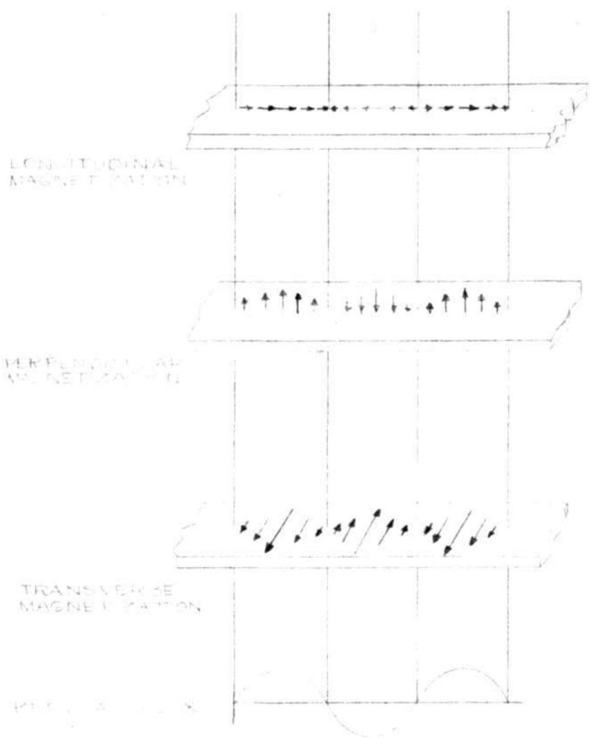
FIG. 1 TYPES OF MAGNETIC RECORDINGS. ARROWS INDICATE DIRECTION AND MAGNITUDE OF FLUX IN SECTIONS OF THE RECORDING MEDIUM.
