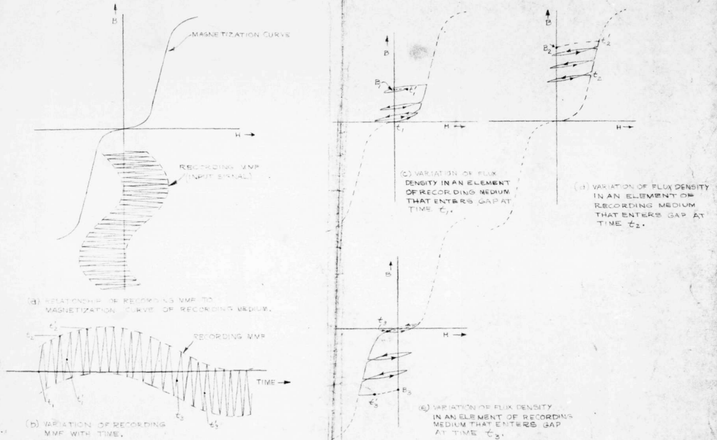
FIG. 5. RELATIONSHIP BETWEEN INPUT SIGNAL AND RECORDED FLUX DENSITY FOR THE A-C BIAS METHOD OF RECORDING.
