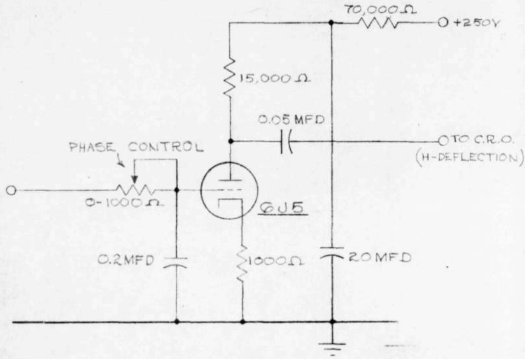
FIG. 25. H-AMPLIFIER FOR B-H CURVE TRACER
