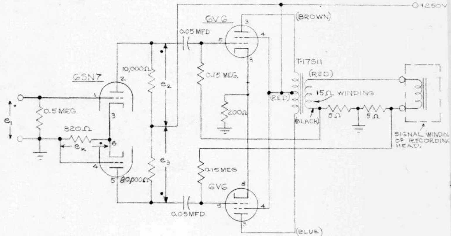
FIG. 15. CIRCUIT DIAGRAM OF RECORDING AMPLIFIER.
