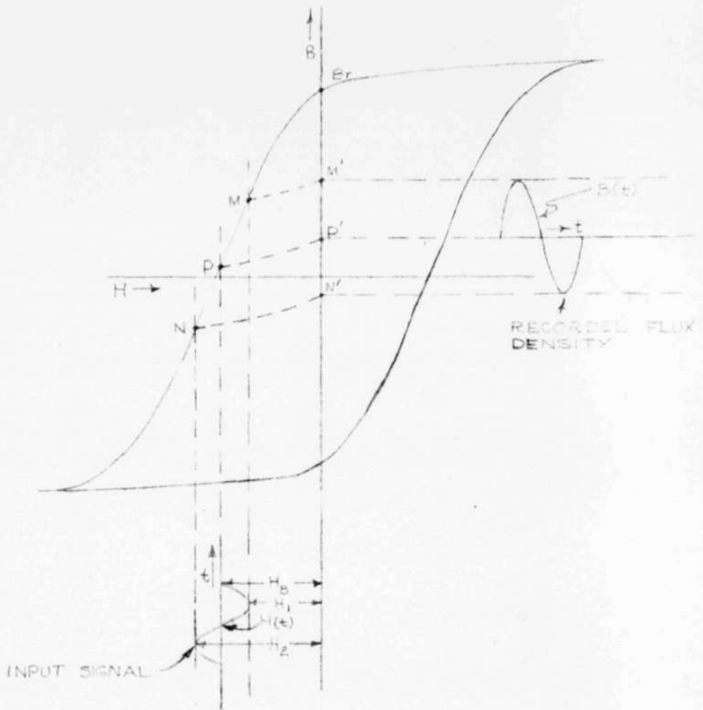
FIG. 4. RELATIONSHIP BETWEEN INPUT SIGNAL AND RECORDED FLUX DENSITY FOR THE D.C. BIAS METHOD OF RECORDING.
