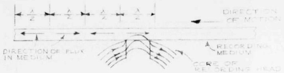
(a) FLUX CONFINED TO REGION BETWEEN GAP FACES.
