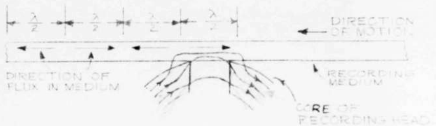
(b) LEAKAGE FLUX SPREADING BEYOND REGION BETWEEN GAP FACES.
