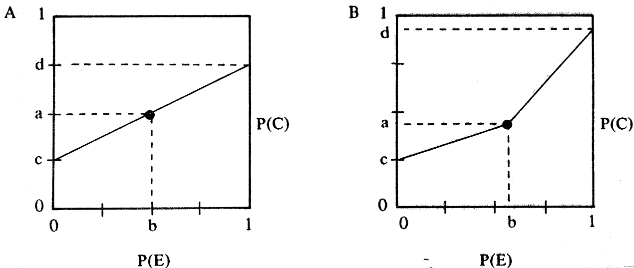
Figure 12: The probability of a conclusion given the probability of the evidence for it. The probability for evidence certain to be absent is c . The probability for evidence certain is d . The prior probabilities of the conclusion and the evidence are a and b in both graphs. Part a illustrates the way the numbers should be related theoretically. Part b illustrates the sort of numbers people give, when asked, and what Duda et al. do with them.
