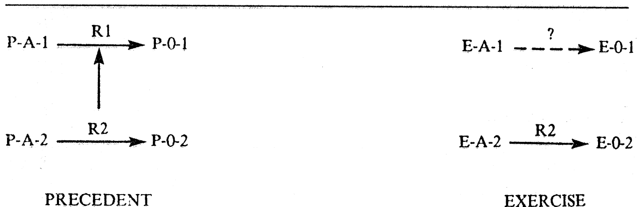
Figure 2: An example illustrating reasoning by analogy. Relation R1 may be justified in the exercise by reason of the causal structure of the precedent and the known relation, R2, in the exercise. Unlabeled relations are CAUSE.
