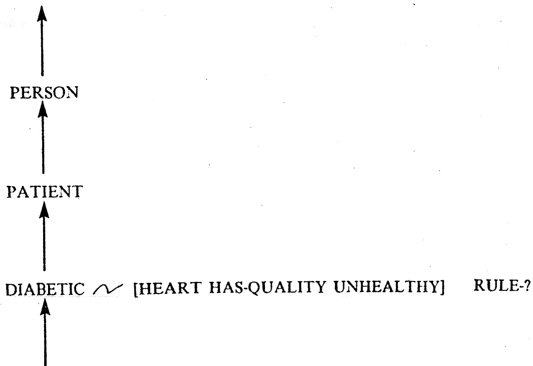
Figure 9: The rule for unhealthy hearts is stored under DIABETIC since the unhealthy heart used to construct the rule was part of a diabetic.
