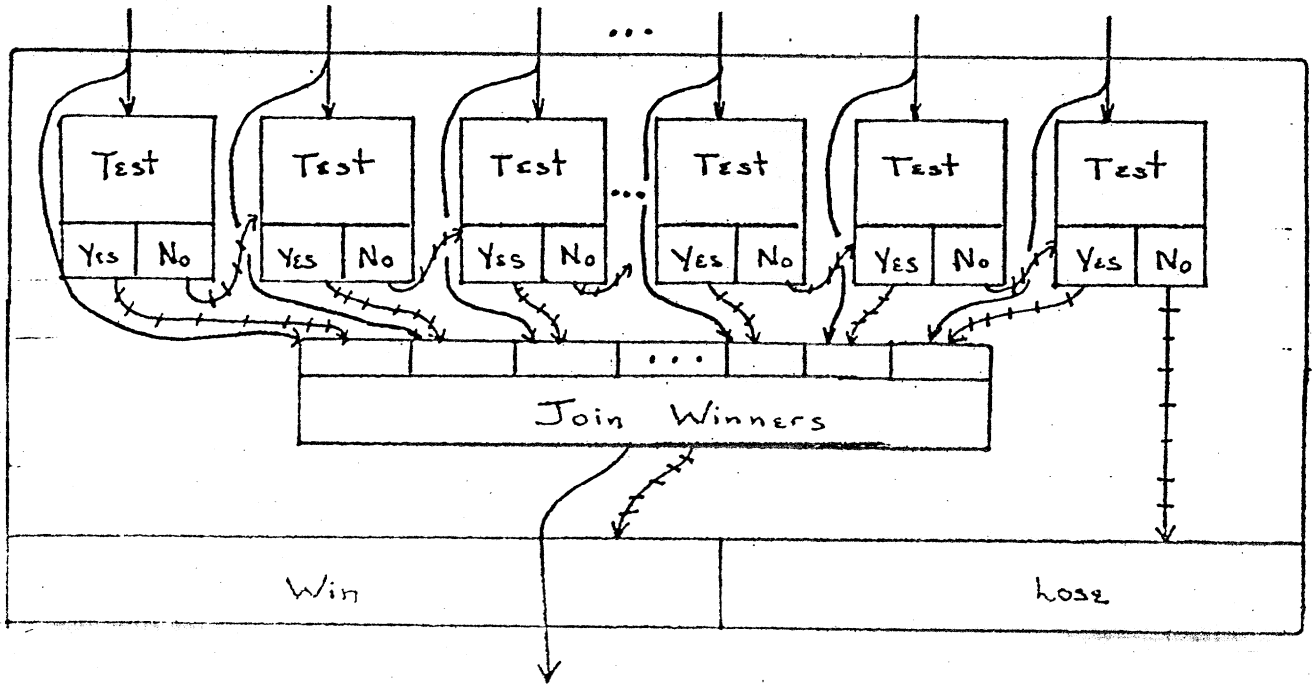
Figure 8: Plan diagram for Linear Search.
