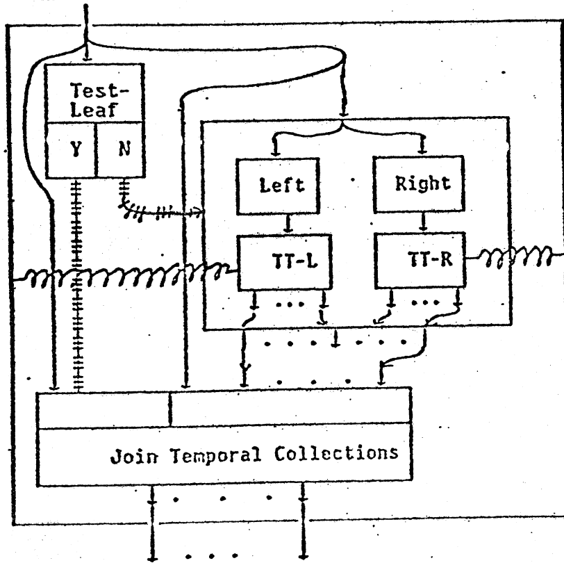
Figure 3: The plan diagram for Tree Traversal.
