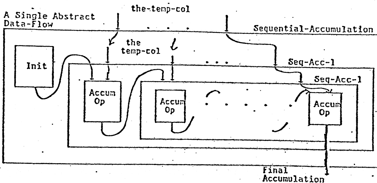
Figure 4: Sequential Accumulation with a Temporal Collection input.
