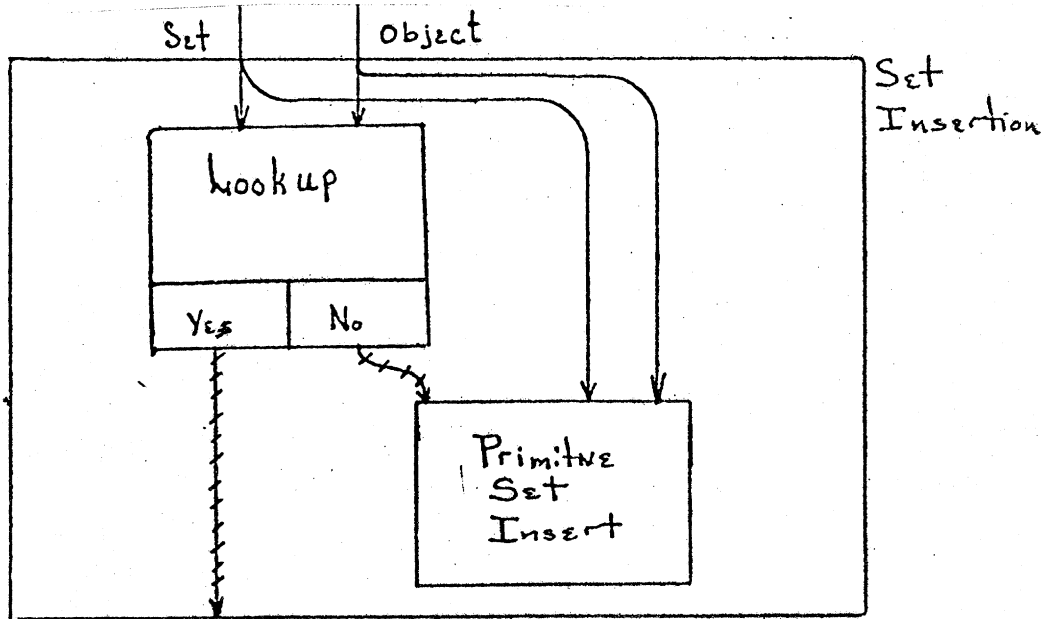
Figure 11: Plan for Set Insertion.
