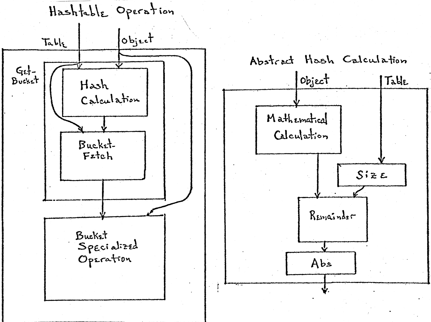
Figure 7: Hashing operations.
