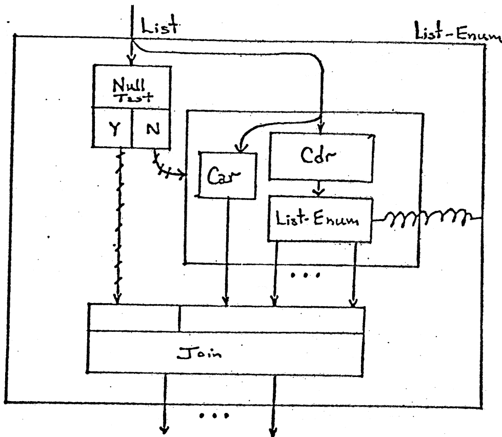
Figure 2: The plan diagram for List Enumeration.
