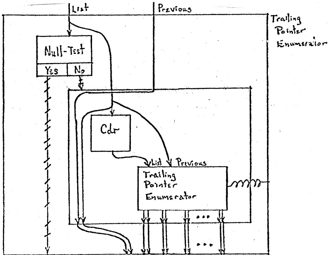
Figure 9: Plan diagram for 'Trailing Pointer Enumeration.
