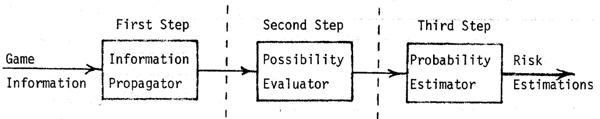
Figure 3.1 The Three Steps of the Locator Algorithm
