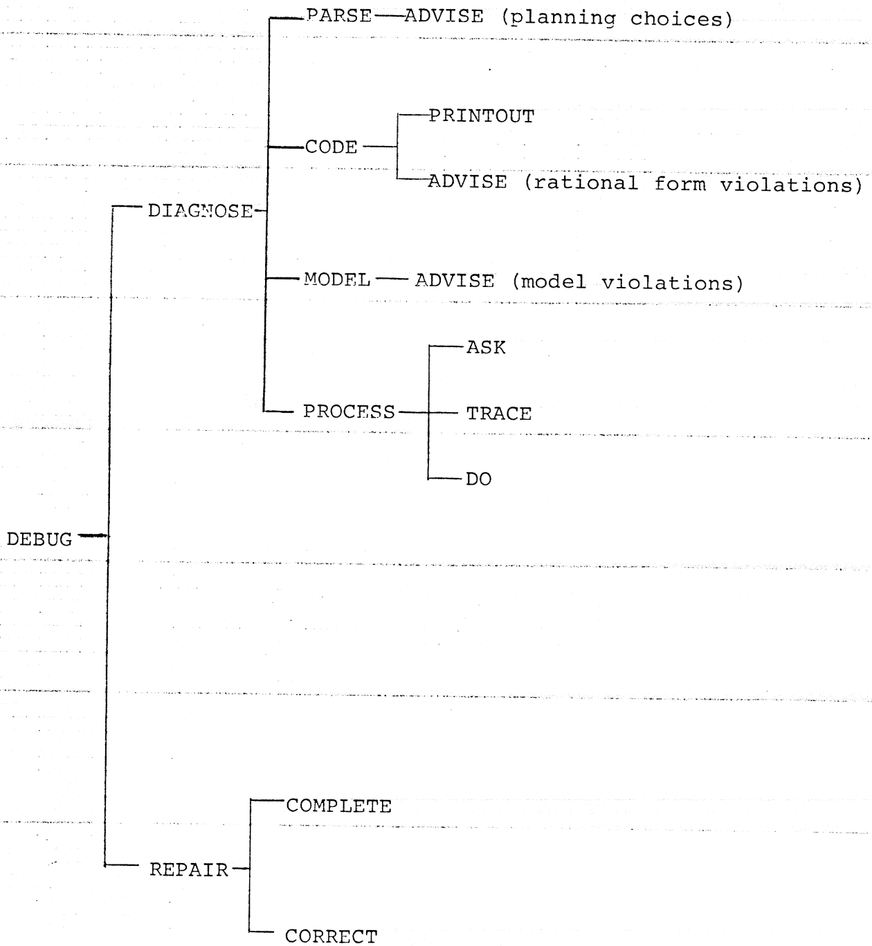
FIGURE 15 - A TAXONOMY OF DEBUGGING TECHNIQUES
