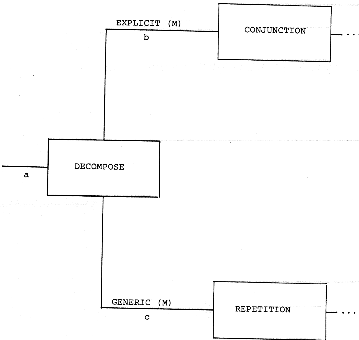
FIGURE 24 PATN'S DECOMPOSE NODE
