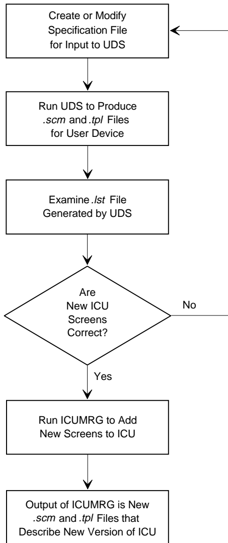
Figure C-1. Adding Drivers with UDS and ICUMRG
