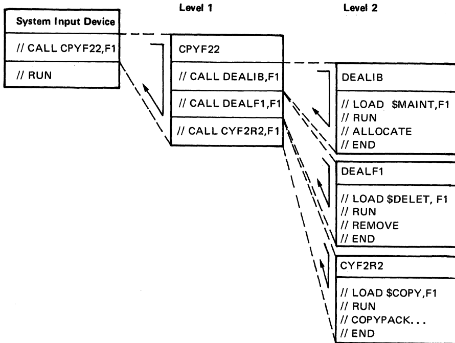
Figure 18. Nested Procedures
