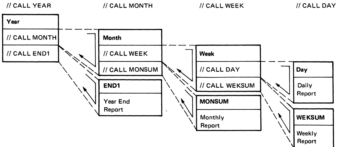
Figure 19. Inventory Example
