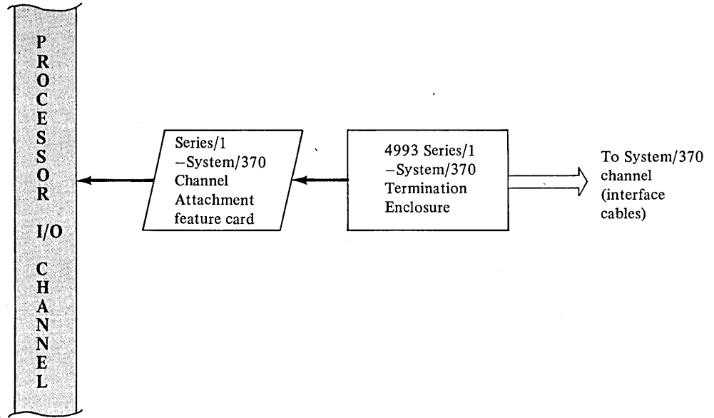
Figure 9-2. Block diagram of 4993 Series/1—System/370 Termination Enclosure
