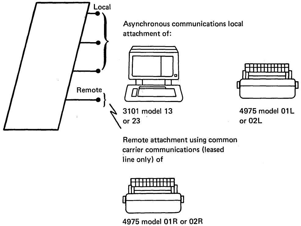
Figure 6-3 (Part 2 of 2). Attachment port configurations
