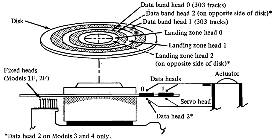
Figure 3-2. Disk and access mechanism
