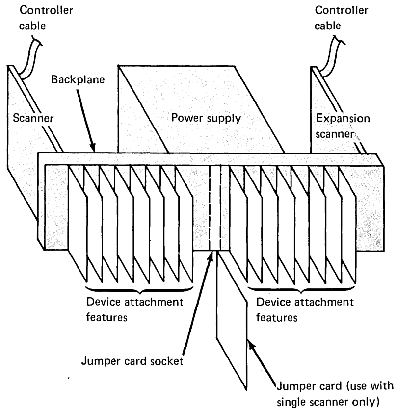
Figure 8-6. 4987 device attachment feature card sockets (rear view)
