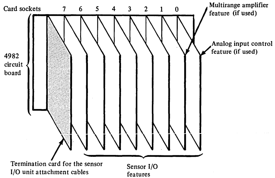
Figure 5-3. 4982 Sensor I/O Unit card sockets (rear view)
