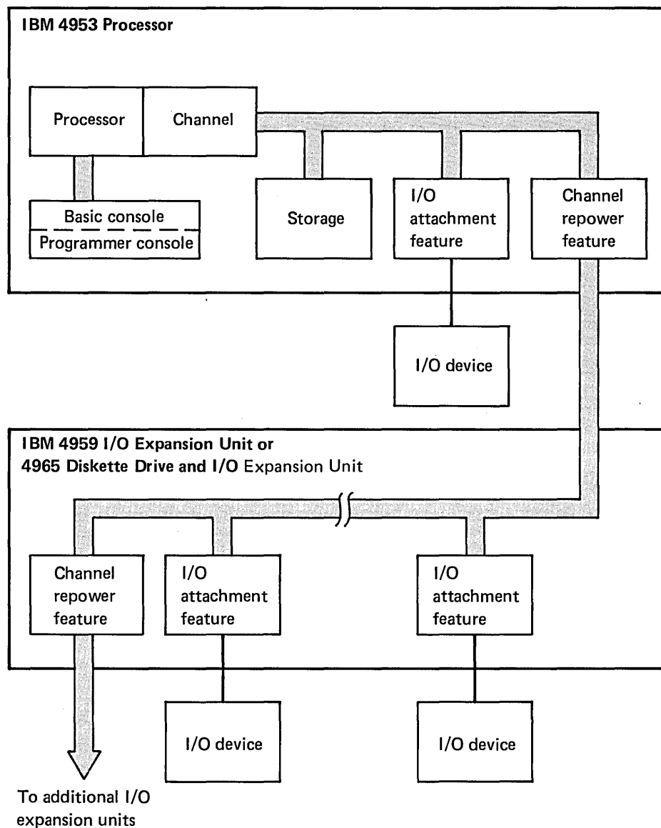
Figure 2-7. Block diagram of a 4953 Processor and a 4959 Input/Output Expansion Unit or a 4965 Diskette Drive and Input/Output Expansion Unit
