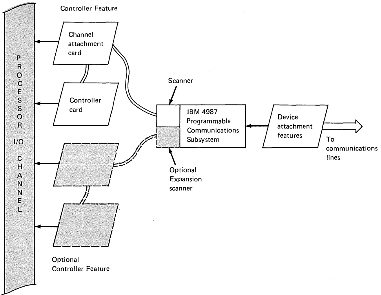
Figure 8-5. Block diagram of a 4987 Programmable Communications Subsystem
