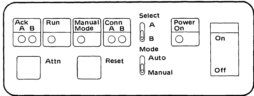
Figure 2-17. TCS console
