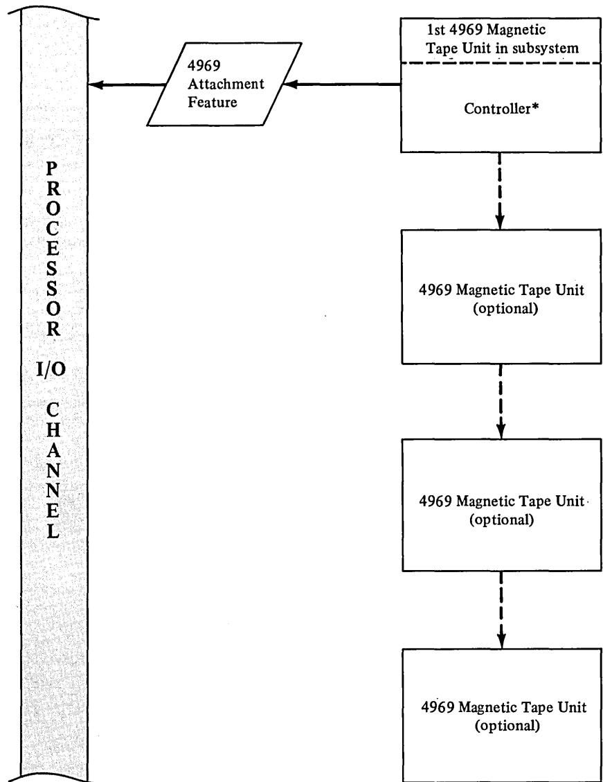
Figure 3-13. Block diagram of a 4969 Magnetic Tape Subsystem
