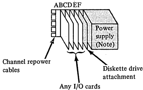
Figure 3-9. Diskette Drive and I/O Expansion Unit card plugging assignments
