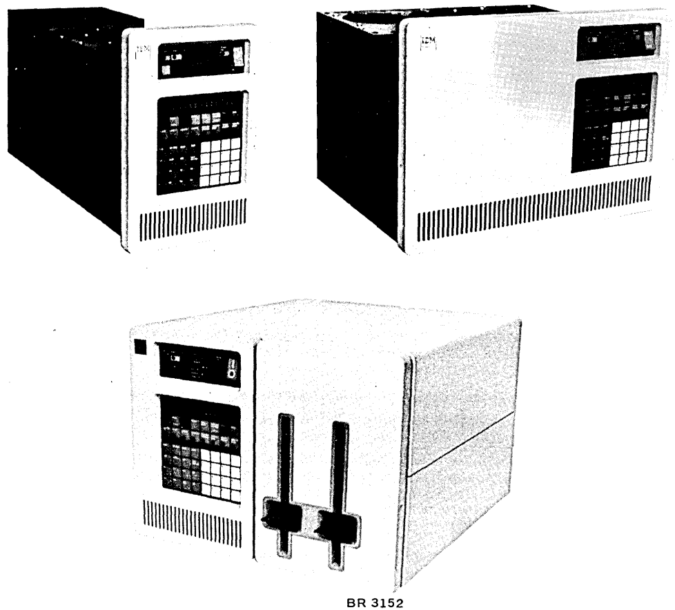
Figure 2-3. 4952 Processor models
