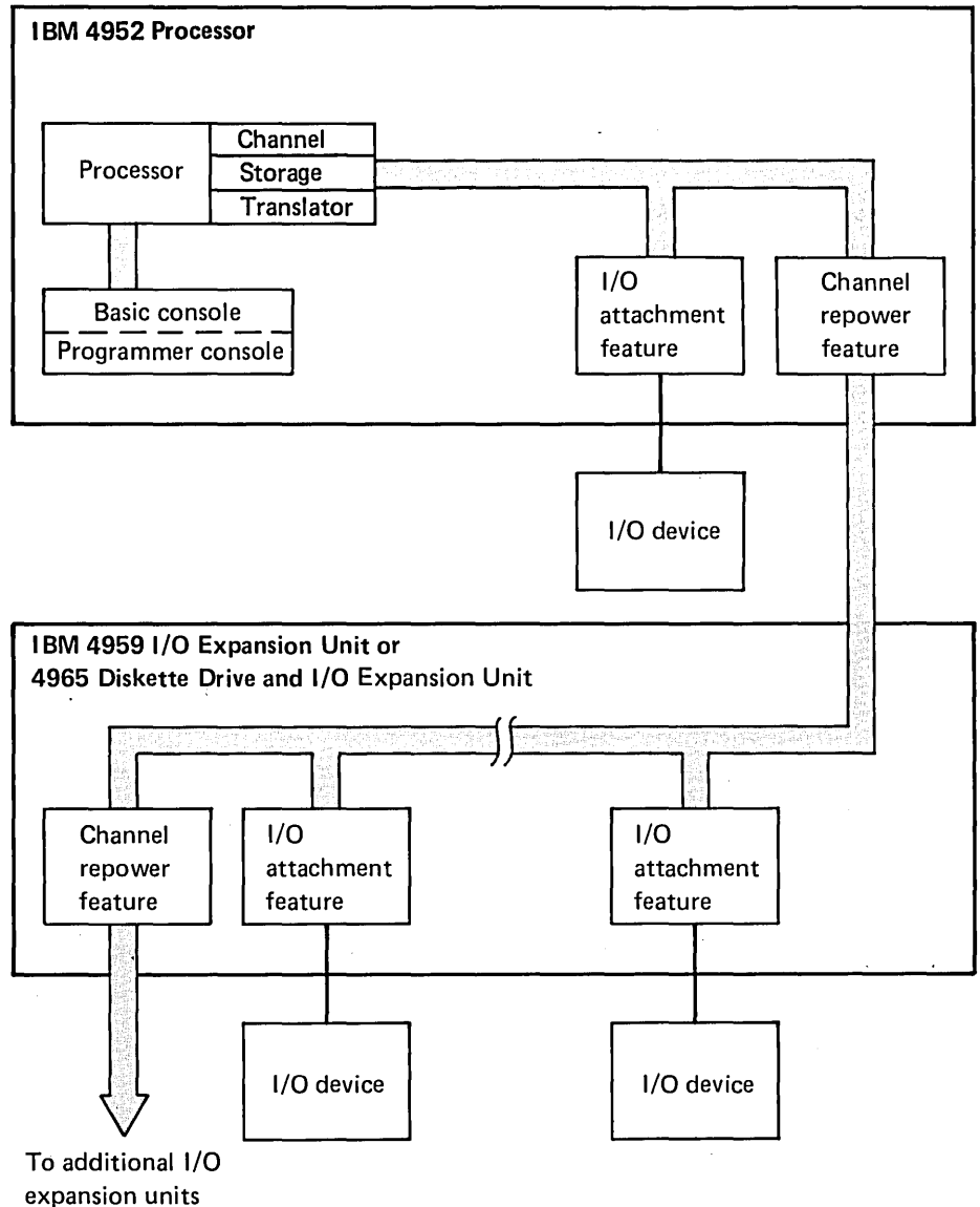
Figure 2-4. Block diagram of a 4952 Processor and a 4959 Input/Output Expansion Unit or 4965 Diskette Drive and Input/Output Expansion Unit
