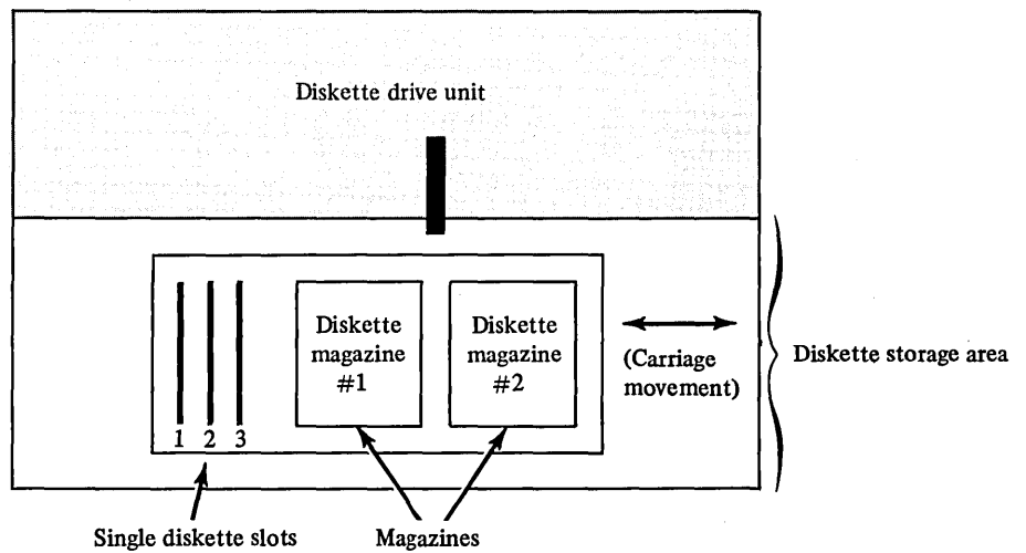
Figure 3-11. Block diagram of the 4966 Diskette Magazine Unit (top view)
