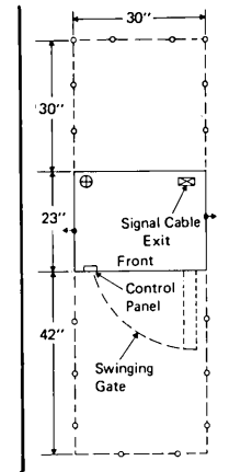
PLAN VIEW (Scale: 1/4" = 1')
